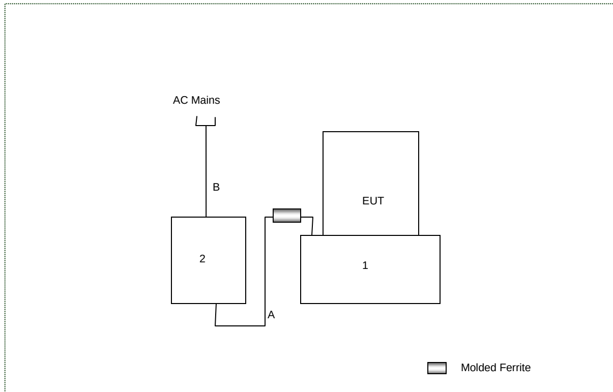
Figure 6-2: EUT Test Setup Power Line Conducted Emissions
