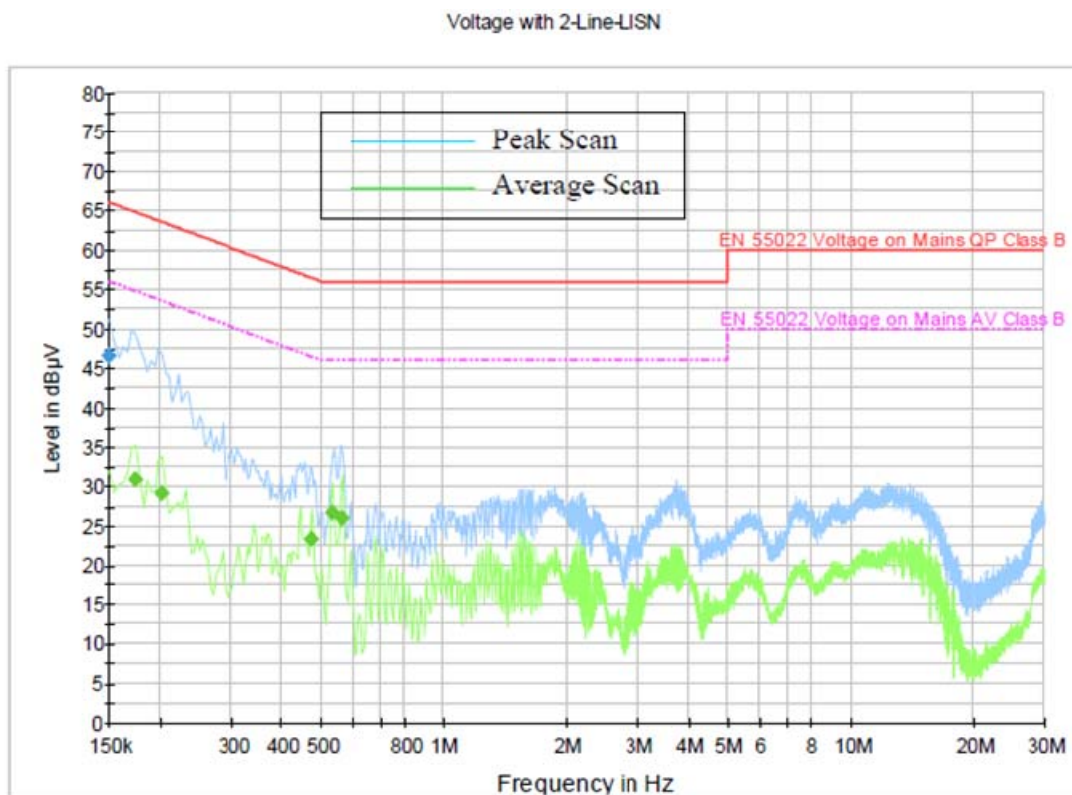
6F-10 – Radio on Transmit Line/Neutral 815.0125 MHz (TMO)
