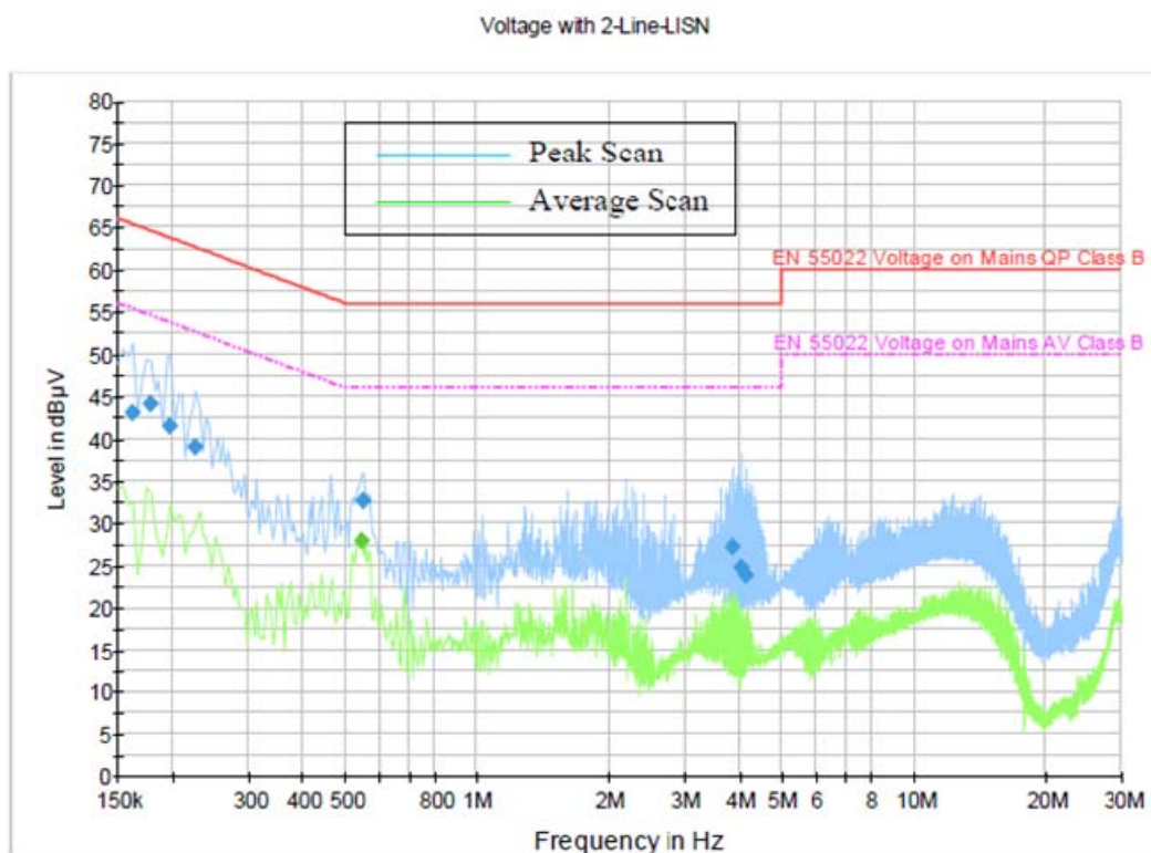
6F-9 – Radio on Transmit Line/Neutral 809.0125 MHz (TMO)
