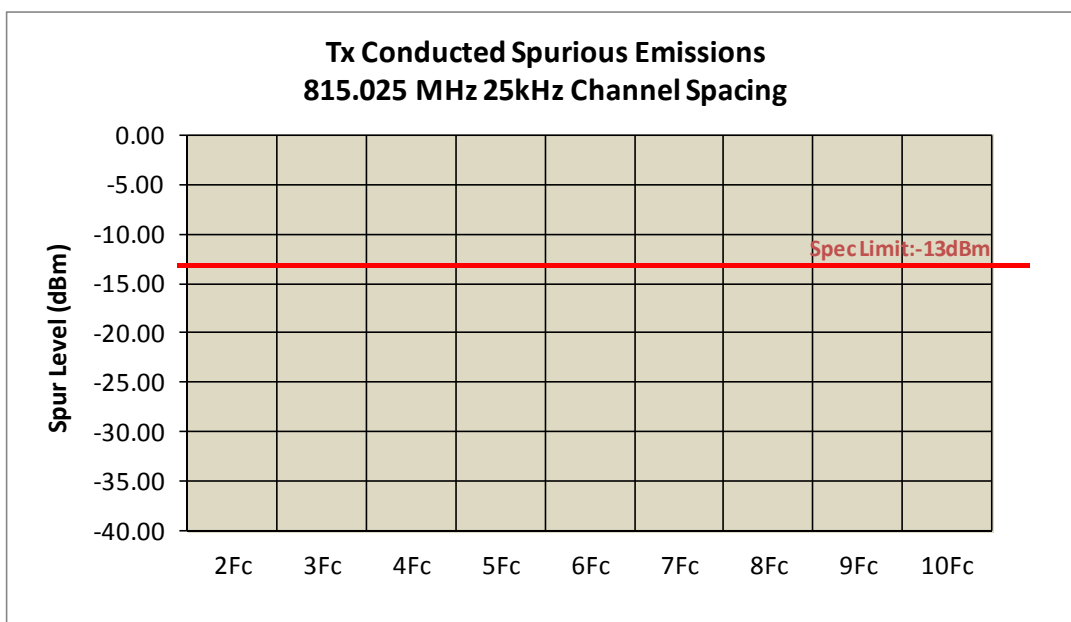
6C-3 – 2 Watts, 815.025 MHz, 25 kHz Channel Spacing
