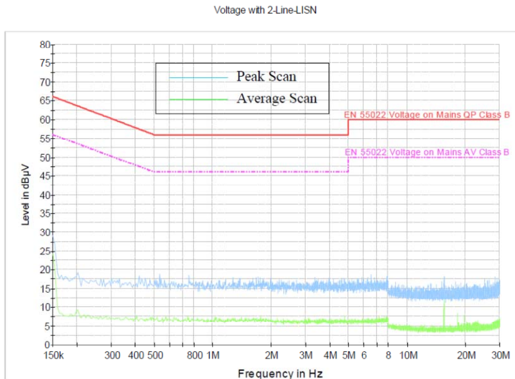
6F-1 – Ambient Noise
