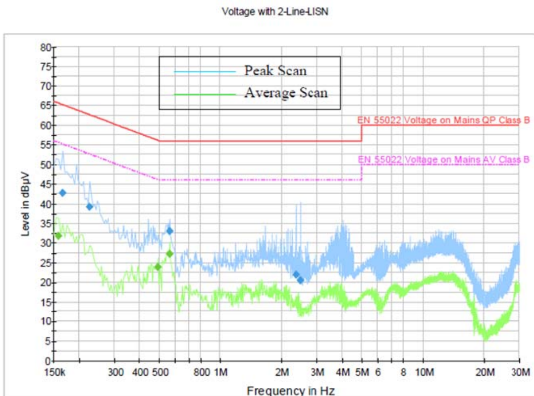
6F-7 – Radio on Transmit Line/Neutral 859.025 MHz (DMO)
