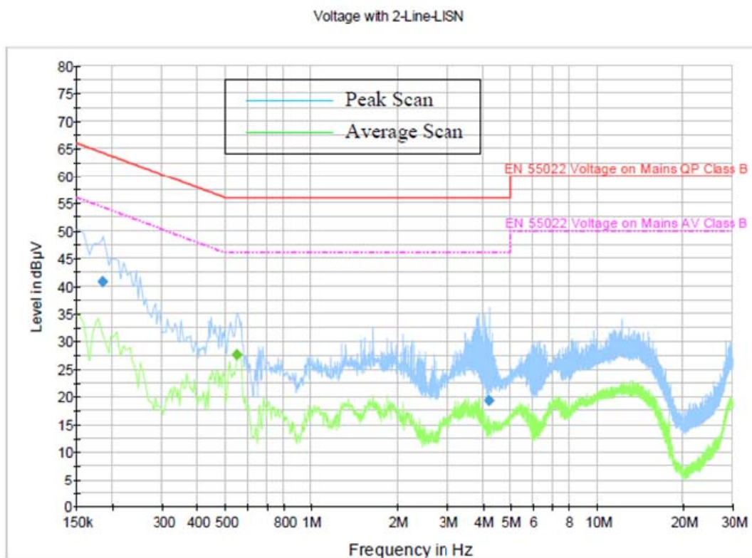
6F-8 – Radio on Transmit Line/Neutral 868.9875 MHz (DMO)
