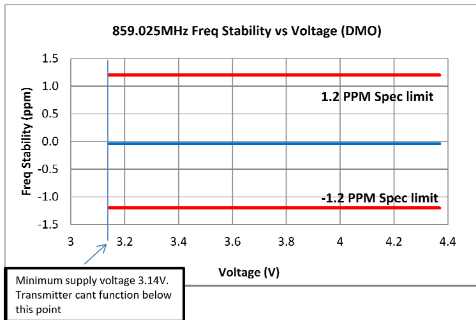
6E-4 – 859.025 MHz Frequency Stability vs. Supply Voltage (DMO)
