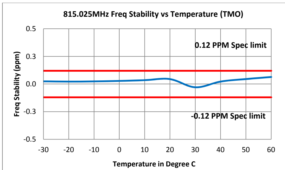
6E-1 – 815.025 MHz Frequency Stability vs. Temperature (TMO)
