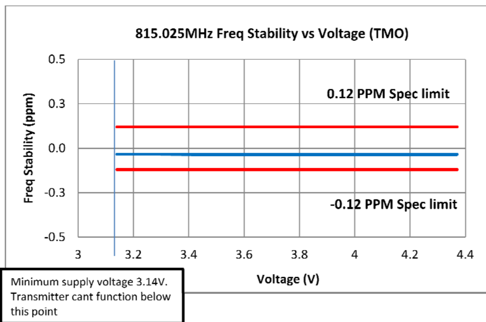
6E-2 – 815.025 MHz Frequency Stability vs. Supply Voltage (TMO)
