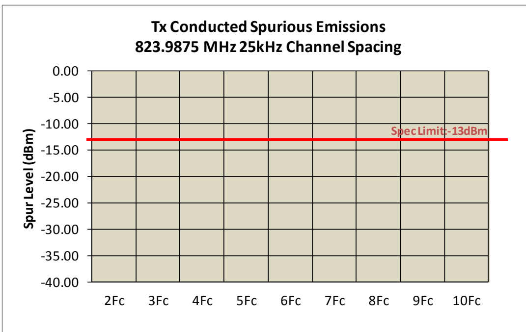
6C-4 – 2 Watts, 823.9875 MHz, 25 kHz Channel Spacing
