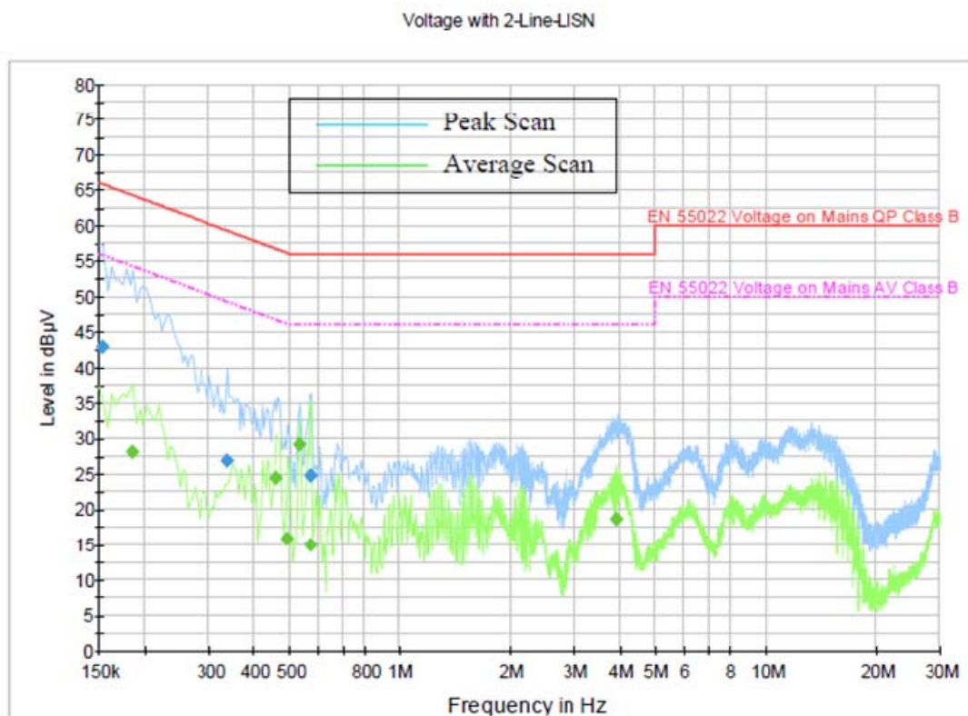
6F-2 – Radio Off Line/Neutral
