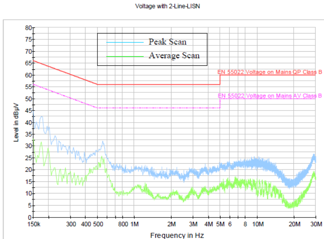
6F-5 – Radio on Receive Line/Neutral 868.9875 MHz (DMO)
