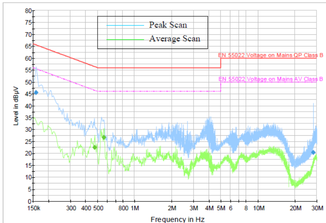
Voltage with 2-Line-LISN
