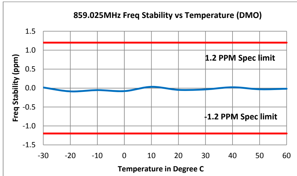
6E-3 – 859.025 MHz Frequency Stability vs. Temperature (DMO)
