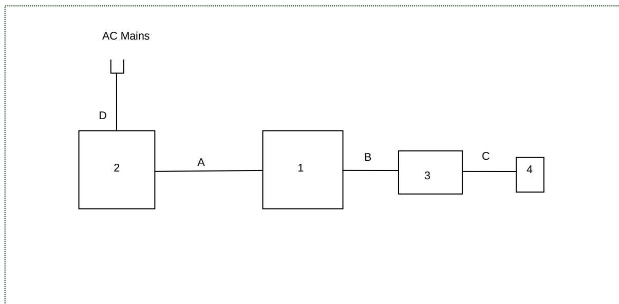
Figure 6-1: Power Line Conducted Emissions Setup
