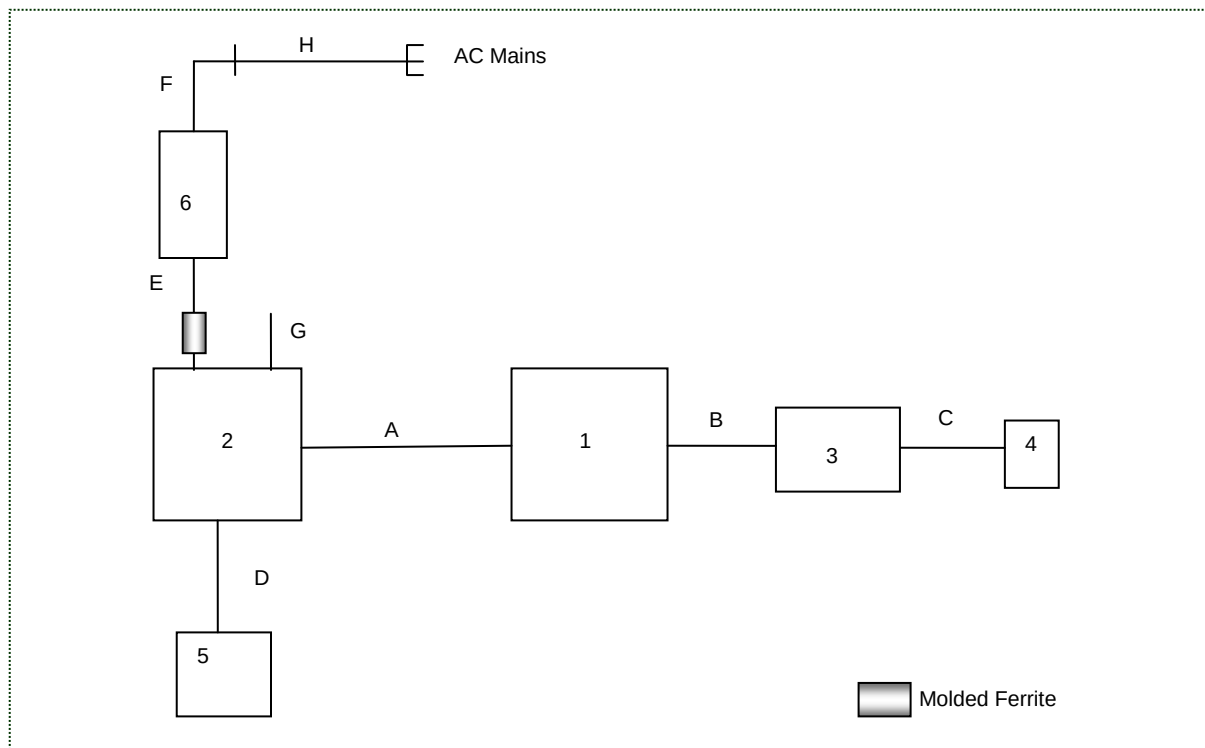
Figure 6-1: Radiated Emissions Setup
