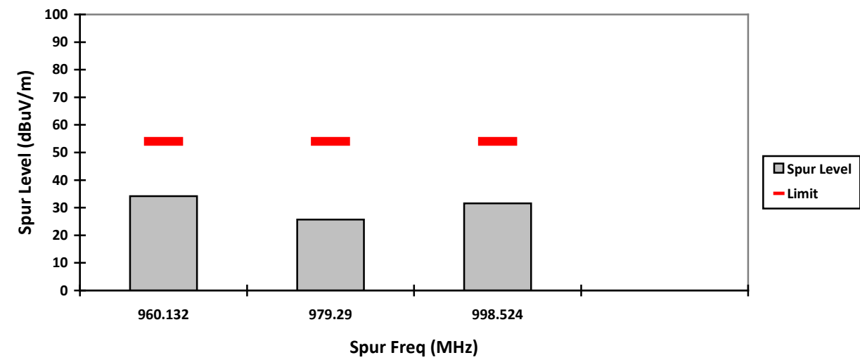
HORIZONTAL, QPK
