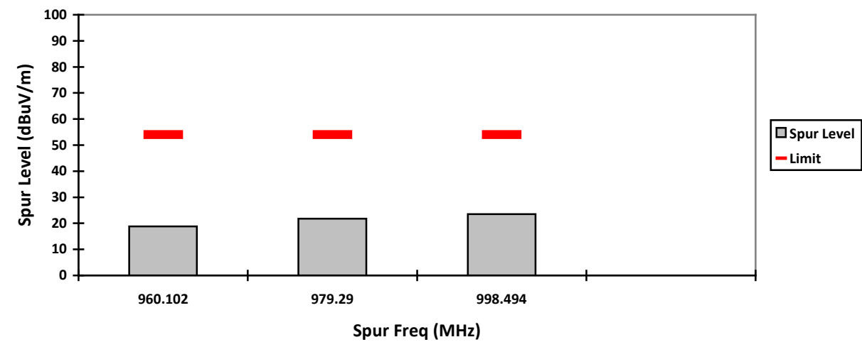
VERTICAL, QPK
