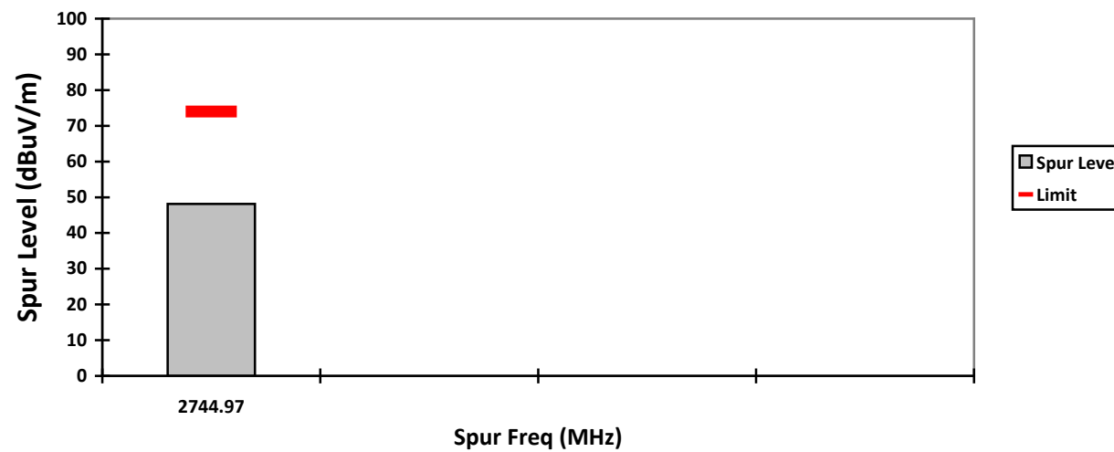
VERTICAL, PK
