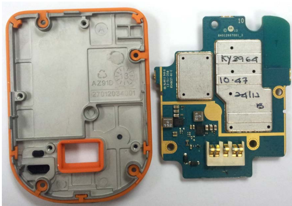
PCB Top with shield
