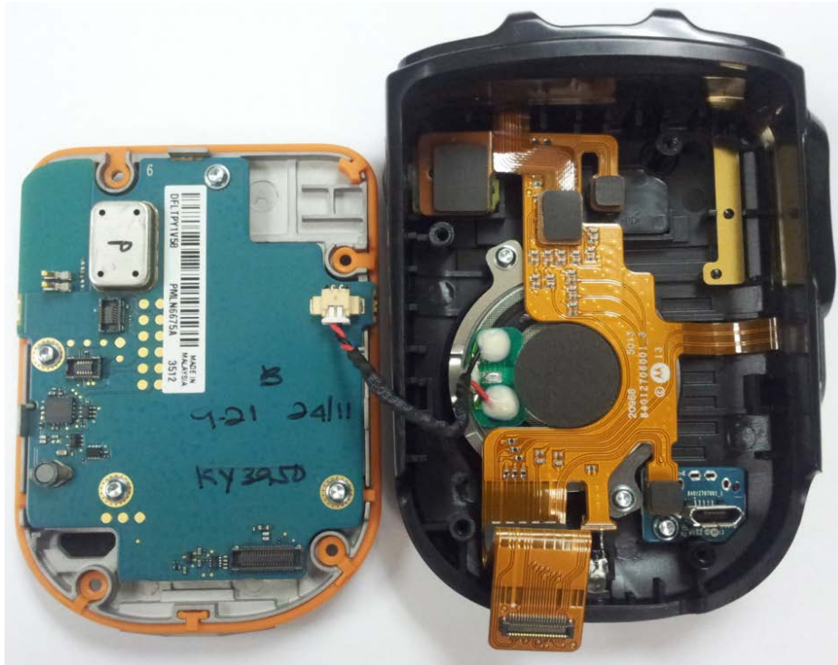
Overall Internal Assembly with housing
