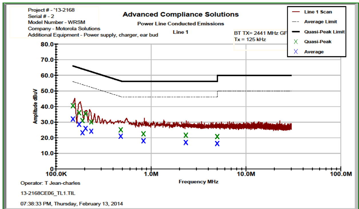
Figure 7.4.2-1: Conducted Emissions Results – Line 1
