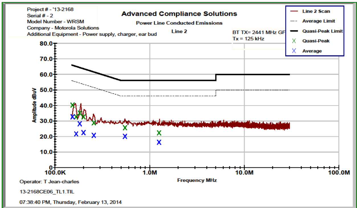
Figure 7.4.2-2: Conducted Emissions Results – Line 2
