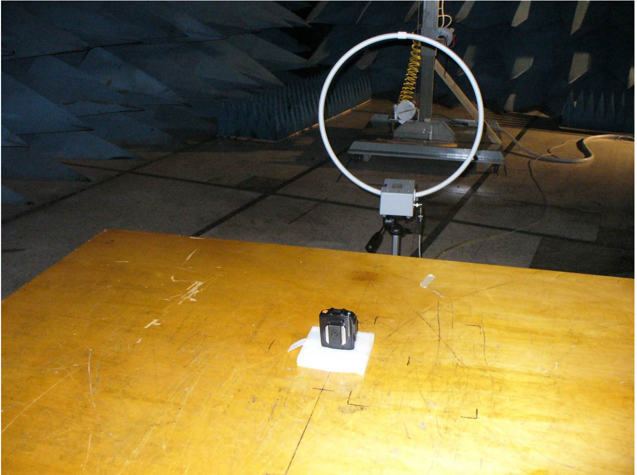
Figure 2: Radiated Emissions – Back View 1
