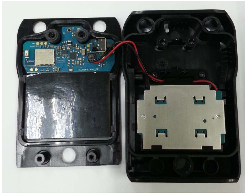
Overall Internal Assembly
