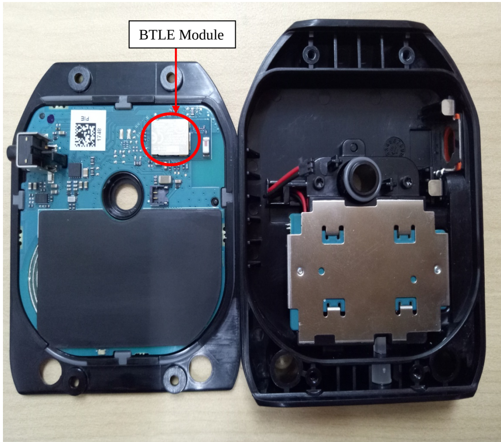
Overall Internal Assembly
