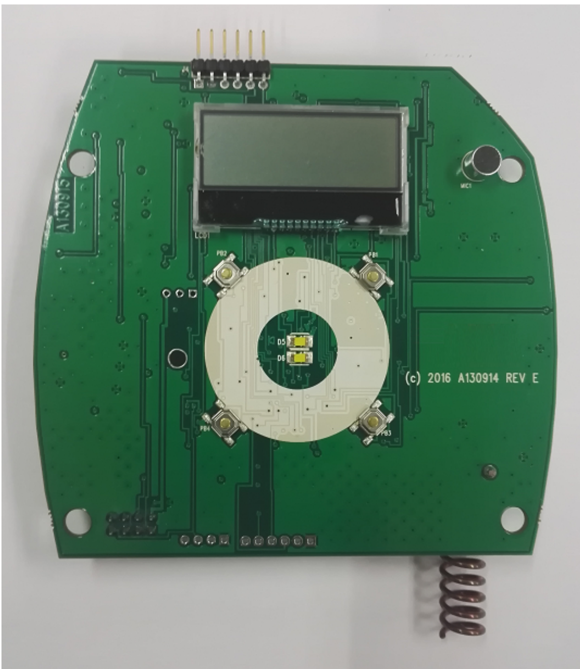
Board Side 2
