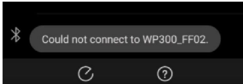
Figure 1 : Message-guide
