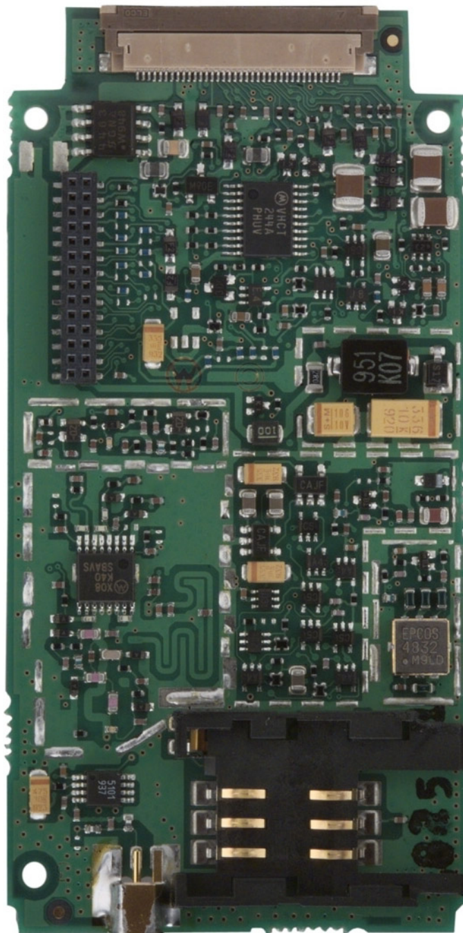
Typical Unit (Top View Shields Removed)
