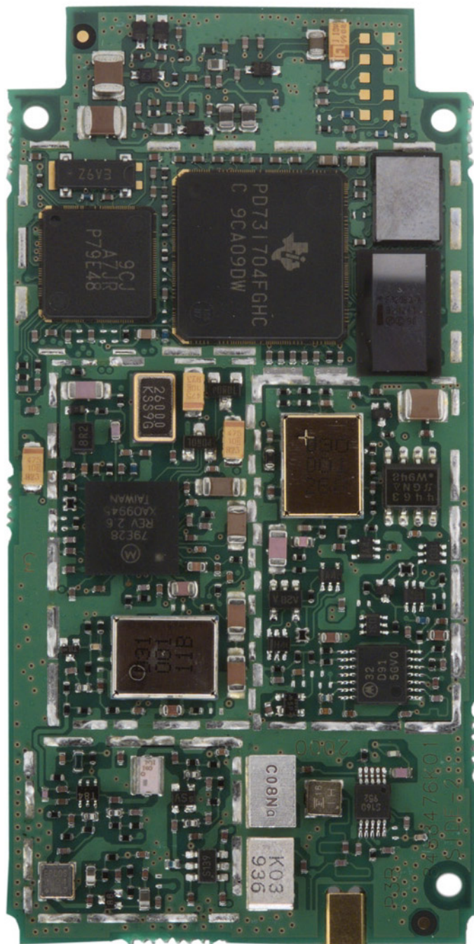
Typical Unit (Bottom View Shields Removed)
