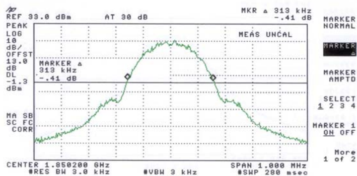
Fig 8.4: Channel 512. -26dBc Bandwidth.
