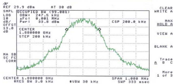
Fig 8.2: Channel 661. 99% Power Bandwidth.
