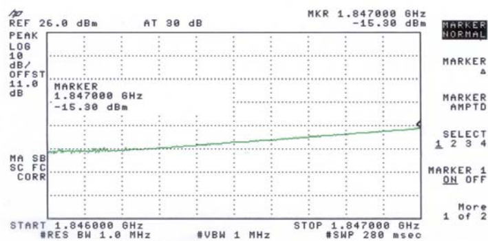
Fig 9.1: Carrier 1850.2 MHz spectrum 1846 to 1847 MHz.
