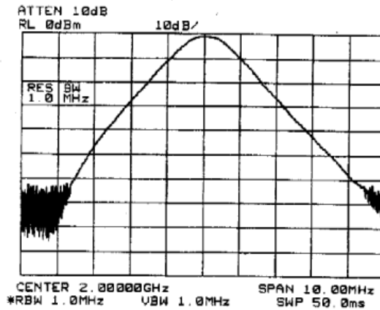
Fig.9.5: Spectrum Analyzer 1 MHz Resolution Bandwidth Filter Response
