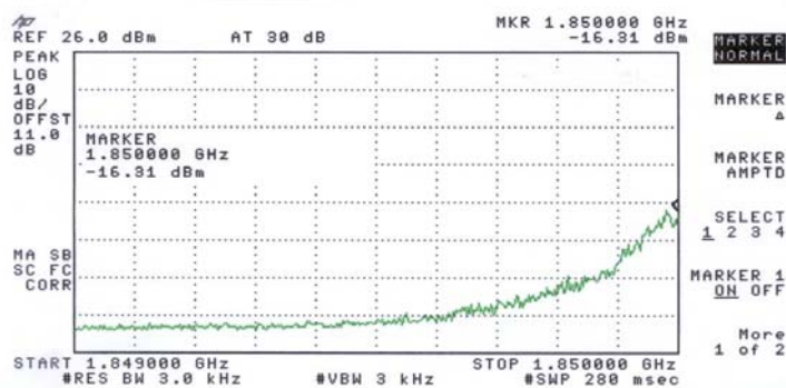
Fig 9.2: Carrier 1850.2 MHz spectrum 1849 to 1850 MHz.
