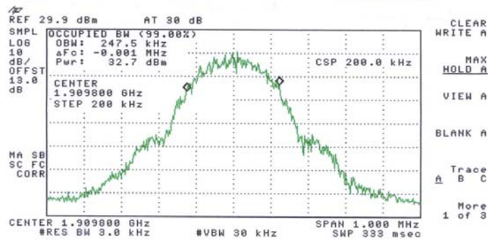
Fig 8.3: Channel 810. 99% Power Bandwidth.
