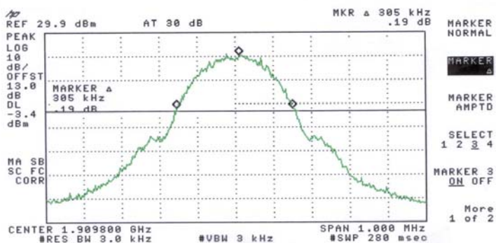
Fig 8.6: Channel 810. -26dBc Bandwidth.
