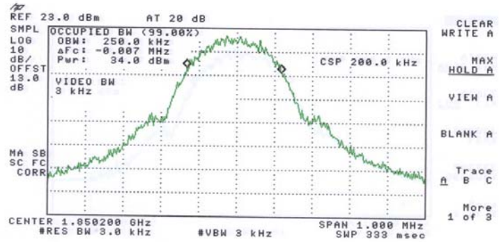
Fig 8.1: Channel 512. 99% Power Bandwidth.
