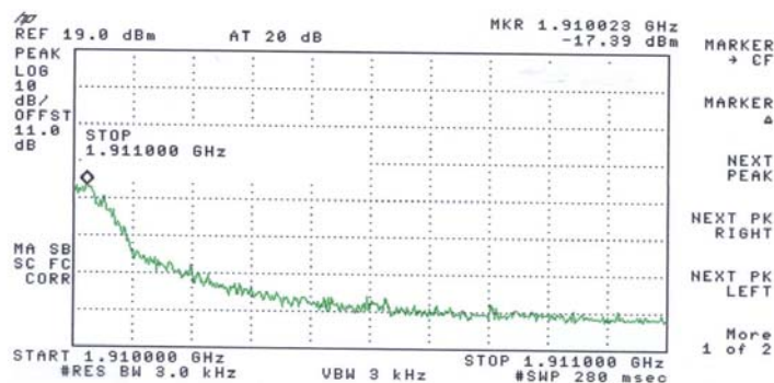
Fig 9.3: Carrier 1909.8 MHz spectrum 1910 to 1911 MHz.
