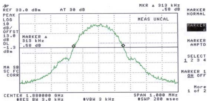
Fig 8.5: Channel 661. -26dBc Bandwidth.
