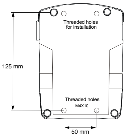
Back side of HDT 600 Cradle
