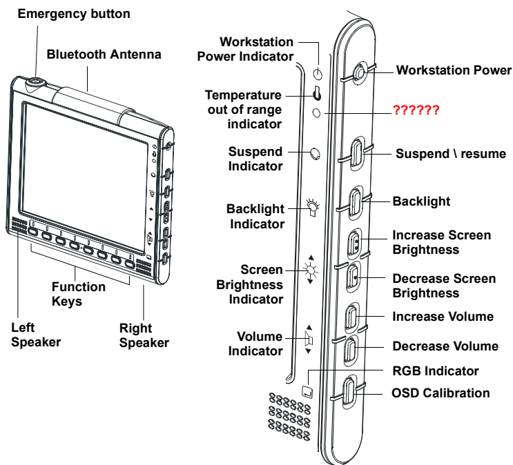
Figure 4 Color Display Unit
