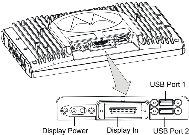
Figure 6 Display - Connectors
