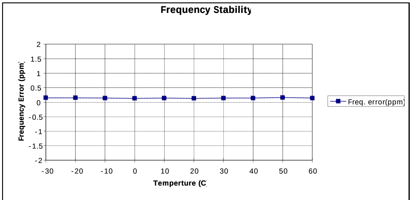
Figure 6-19: Frequency Stability vs. Temperature
