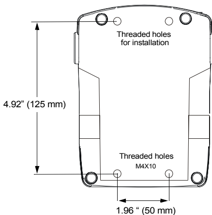
Back side of HDT 600 Cradle
