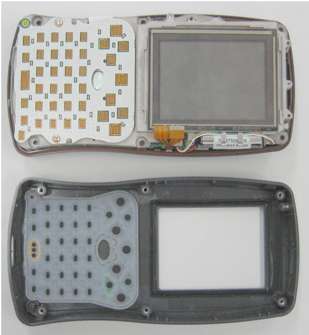
Photograph No.1 X-PAD handheld data terminal internal view
