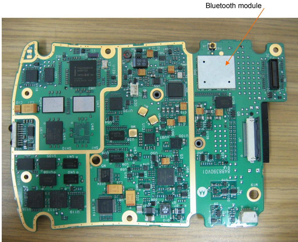
Photograph No.8 Second side of the main PCB
