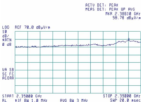
Plot 7.3.21 Radiated emission measurements at band edge at the low carrier frequency, bitrate 1 MBit/s
