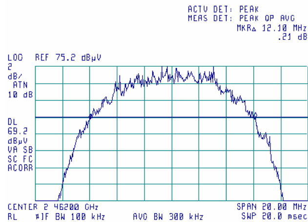
Plot 7.1.12 The 6 dB bandwidth test result at high frequency, bitrate 11 Mbit/s
