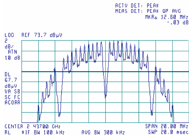
Plot 7.1.6 The 6 dB bandwidth test result at mid frequency, bitrate 2 Mbit/s
