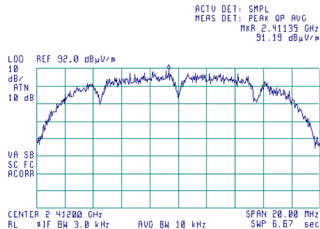
Plot 7.4.2 Peak spectral power density at low frequency zoomed at the peak, 1 MBit/s
