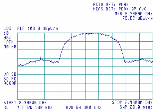
Plot 7.3.23 Radiated emission measurements at band edge at the low carrier frequency, bitrate 11 MBit/s
