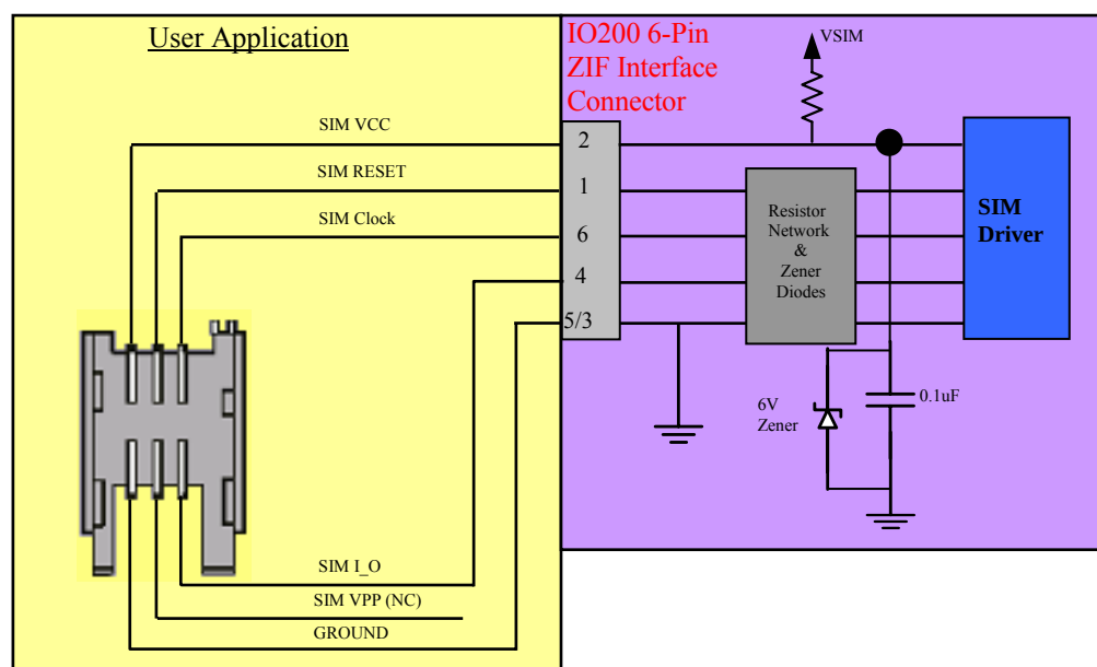
Figure 4. Shows IO200 SIM connection
