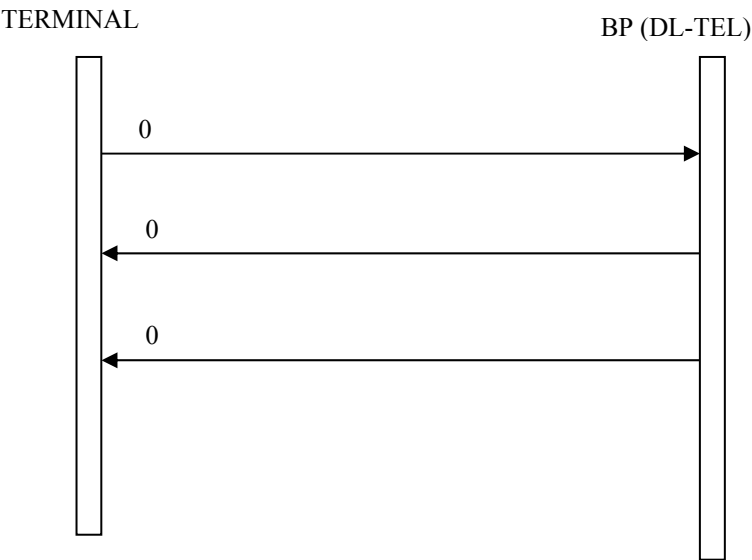
Figure 17. Trace Mode Query and Enable
