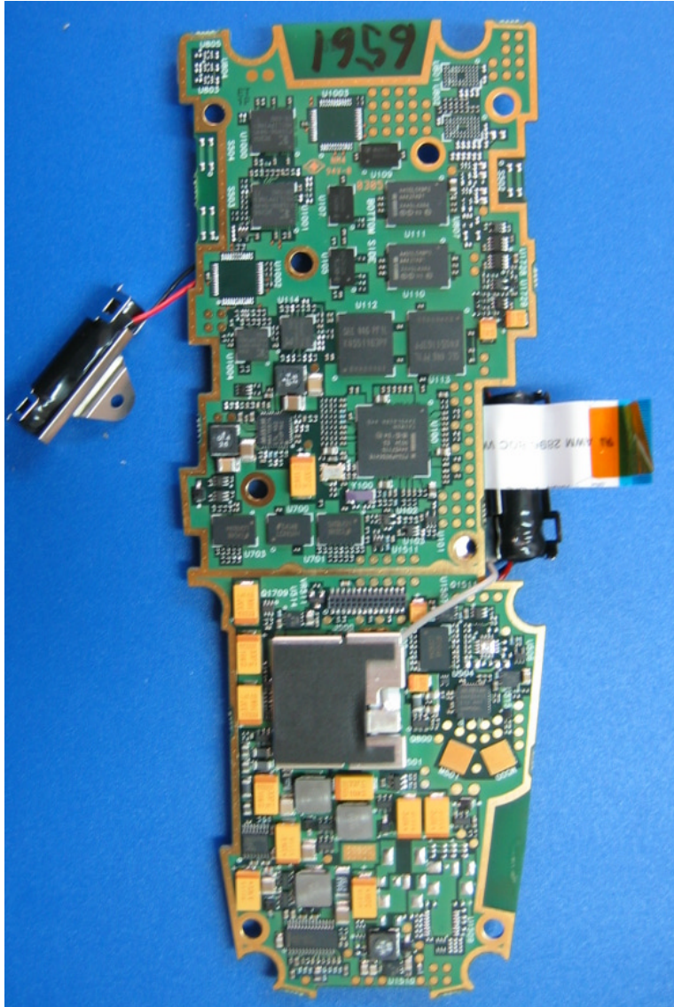
Photograph No.4 IMD SV, second side of the main PCB
