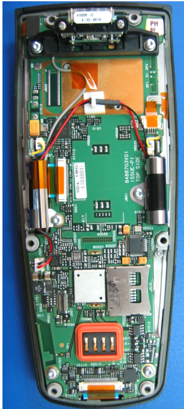
Photograph No.1 Intelligent Mail Device Surface Visibility (IMD SV) internal view
