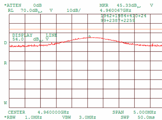
Plot 7.3.64 Radiated emission measurements at the second harmonic of high carrier frequency
