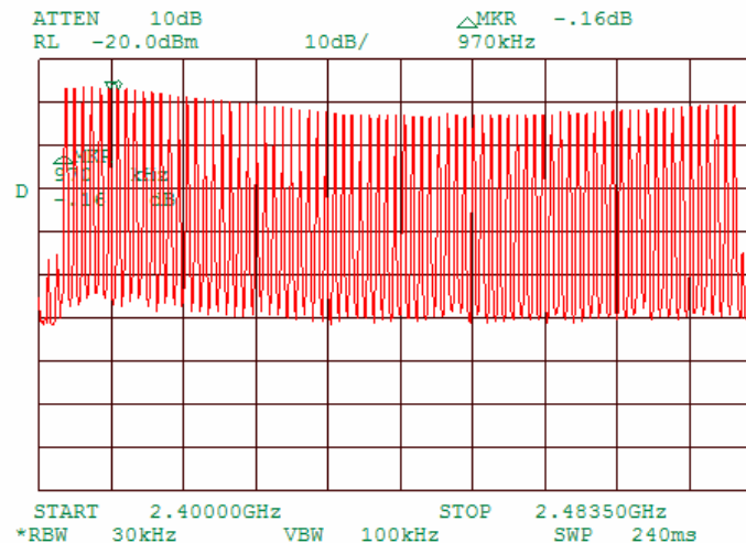
Plot 8.3.1 Carrier frequency separation
