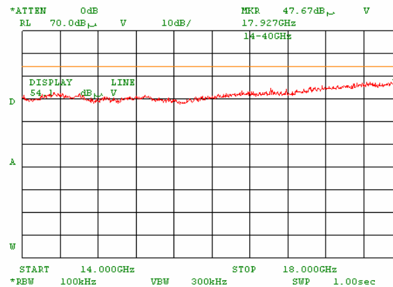
Plot 7.3.48 Radiated emission measurements from 14000 to 18000 MHz at the mid carrier frequency
