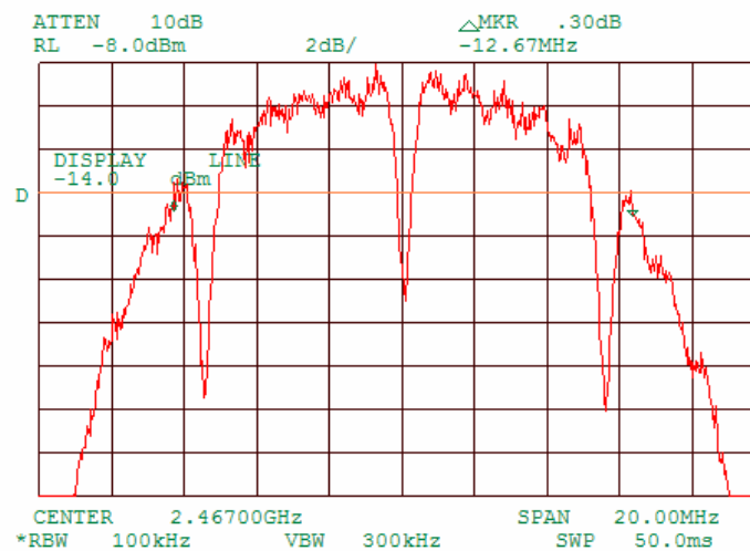
Plot 7.1.10 6 dB bandwidth test result at high frequency, 2 MBPS
