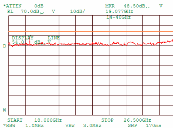
Plot 7.3.51 Radiated emission measurements from 18000 to 26500 MHz at the mid carrier frequency
