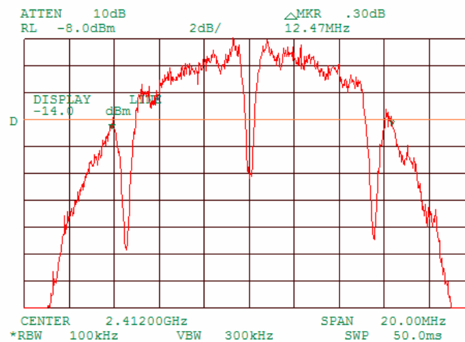
Plot 7.1.2 6 dB bandwidth test result at low frequency, 2 MBPS
