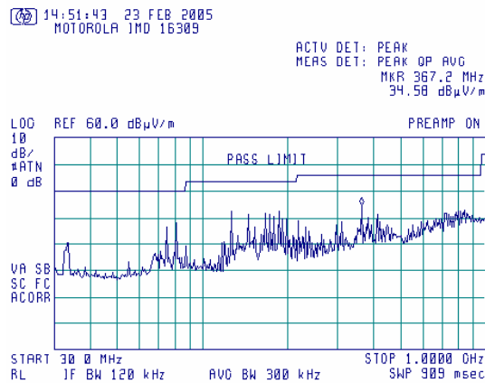
Plot 7.3.17 Radiated emission measurements from 30 to 1000 MHz at the mid carrier frequency
