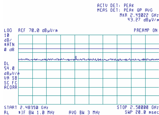
Plot 7.3.30 Radiated emission measurements from 2483.5 to 2500 MHz at the mid carrier frequency
