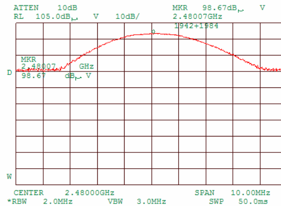
Plot 8.6.3 Field strength of carrier at high frequency
