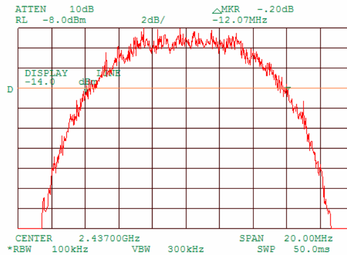
Plot 7.1.7 6 dB bandwidth test result at mid frequency, 5.5 MBPS
