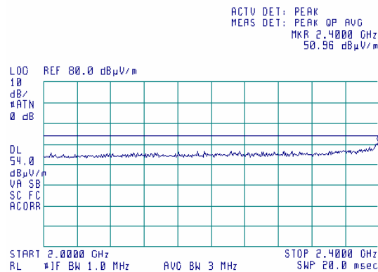
Plot 7.3.28 Radiated emission measurements from 2000 to 2400 MHz at the high carrier frequency
