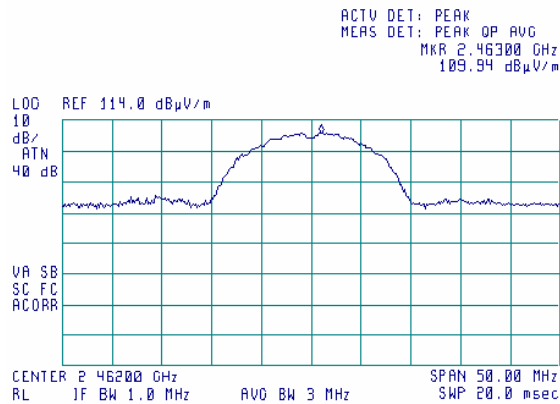
Plot 7.3.92 Radiated emission measurements at carrier, average
