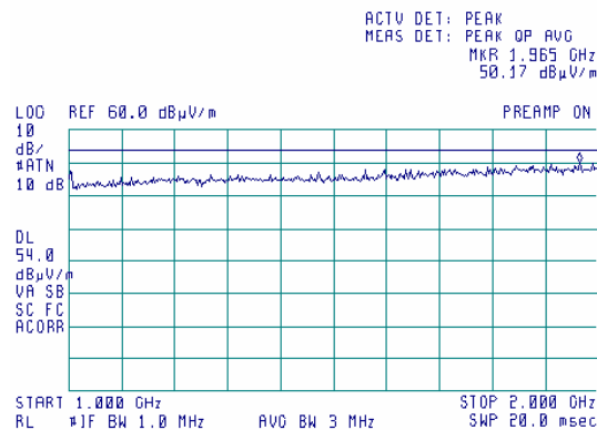
Plot 7.3.22 Radiated emission measurements from 1000 to 2000 MHz at the mid carrier frequency
