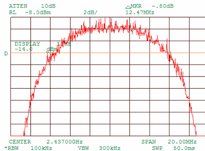
Plot 7.1.8 6 dB bandwidth test result at mid frequency, 11 MBPS
