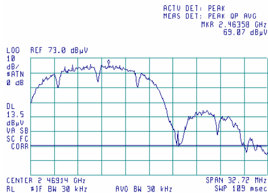
Plot 7.3.94 Radiated emission measurements at band edge
