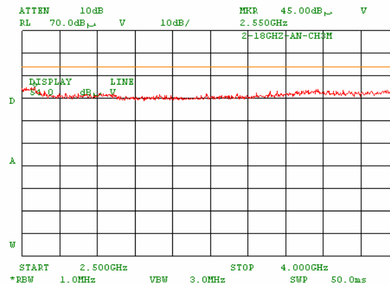
Plot 7.3.35 Radiated emission measurements from 2500 to 4000 MHz at the mid carrier frequency
