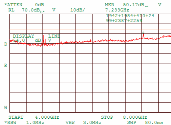
Plot 7.3.38 Radiated emission measurements from 4000 to 8000 MHz at the mid carrier frequency
