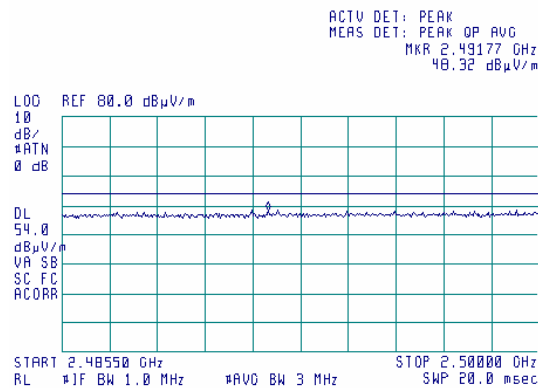
Plot 7.3.33 Radiated emission measurements from 2485.5* to 2500 MHz at the high carrier frequency
