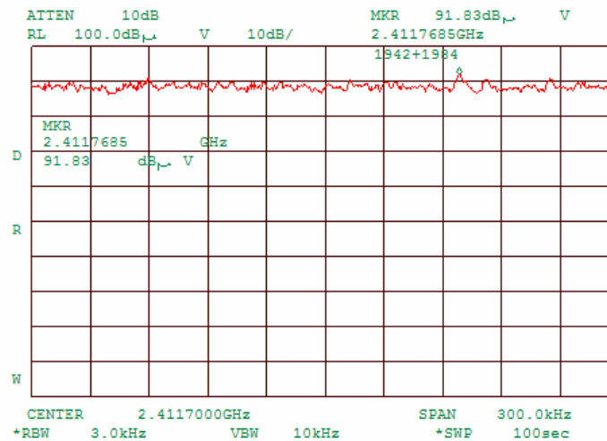
Plot 7.4.8 Peak spectral power density at low frequency zoomed at the peak, 11 MBPs
