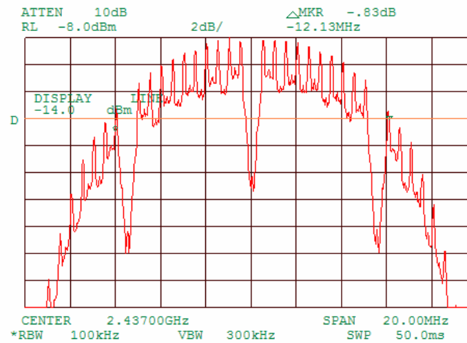
Plot 7.1.5 6 dB bandwidth test result at mid frequency, 1 MBPS
