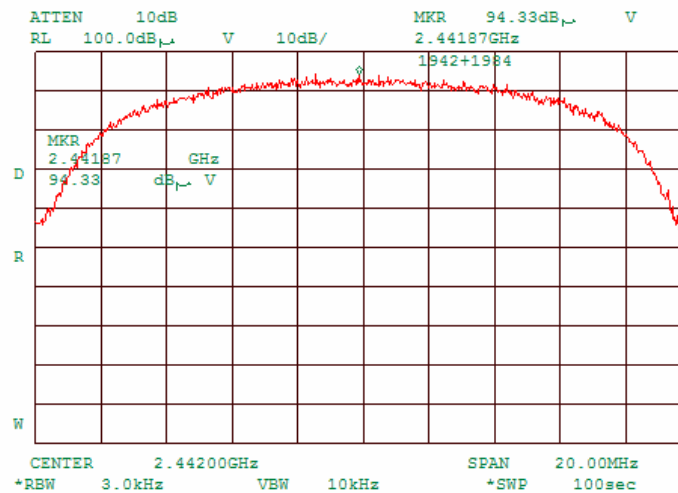
Plot 7.4.10 Peak spectral power density at mid frequency zoomed at the peak, 11 MBPs
