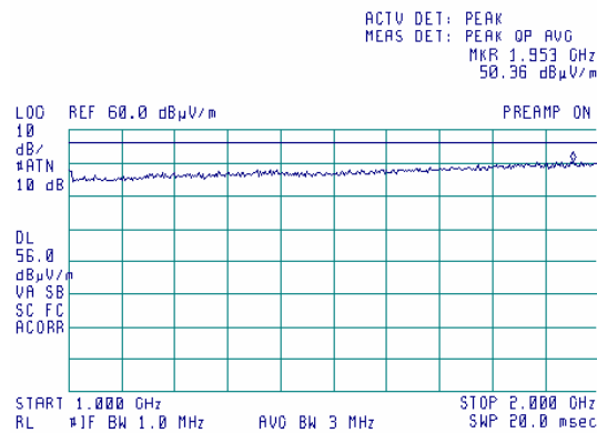
Plot 7.3.24 Radiated emission measurements from 1000 to 2000 MHz at the high carrier frequency
