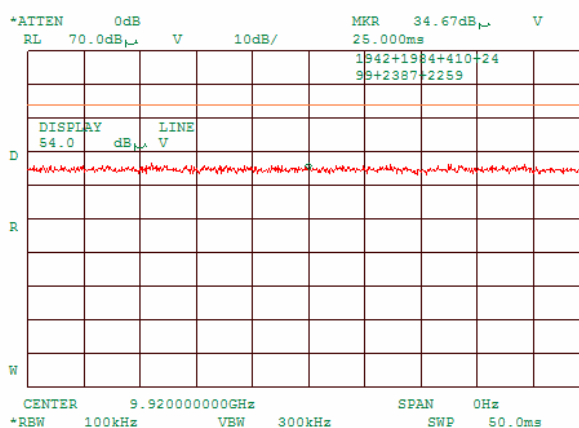
Plot 7.3.82 Radiated emission measurements at the forth harmonic of high carrier frequency
