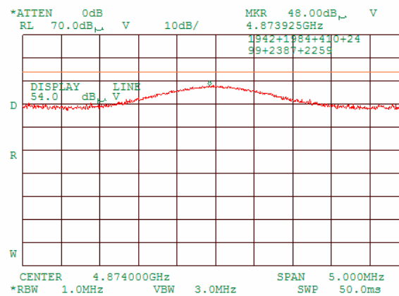
Plot 7.3.62 Radiated emission measurements at the second harmonic of mid carrier frequency
