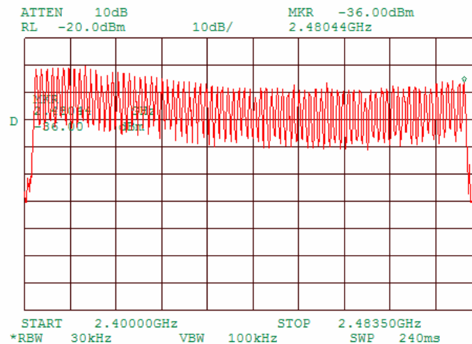
Plot 8.4.1 Number of hopping frequencies
