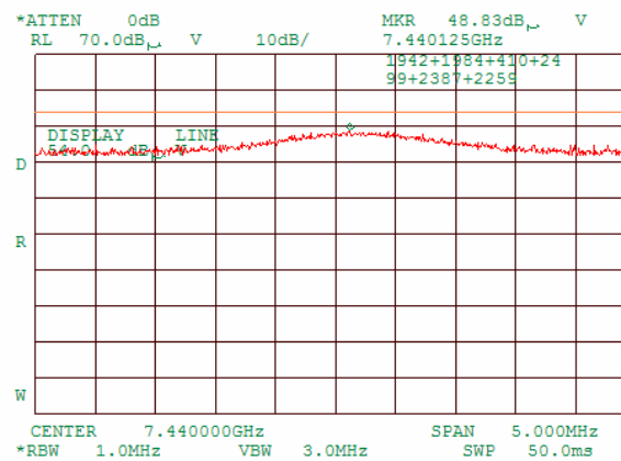
Plot 7.3.74 Radiated emission measurements at the third harmonic of high carrier frequency
