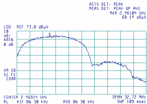
Plot 7.3.98 Radiated emission measurements at band edge
