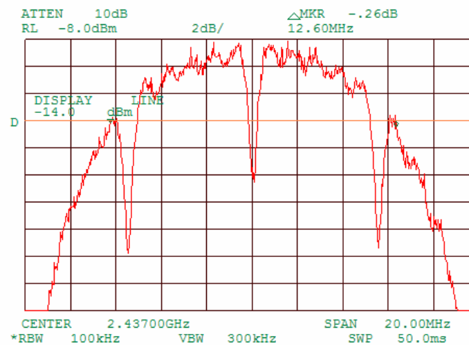
Plot 7.1.6 6 dB bandwidth test result at mid frequency, 2 MBPS
