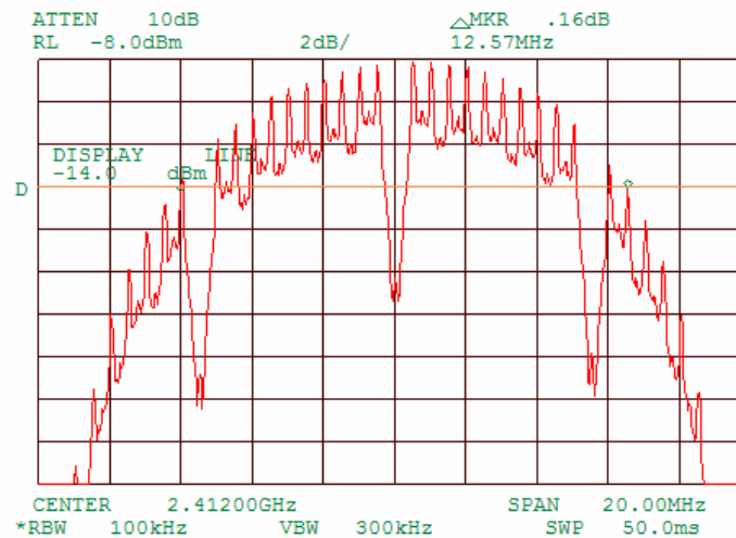
Plot 7.1.1 6 dB bandwidth test result at low frequency, 1 MBPS
