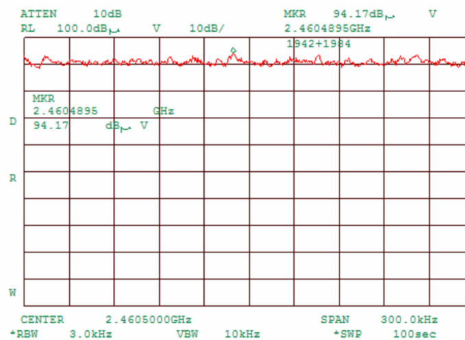
Plot 7.4.12 Peak spectral power density at high frequency zoomed at the peak, 11 MBPs
