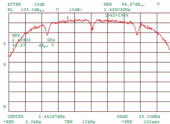
Plot 7.4.4 Peak spectral power density at mid frequency zoomed at the peak, 1 MBPs
