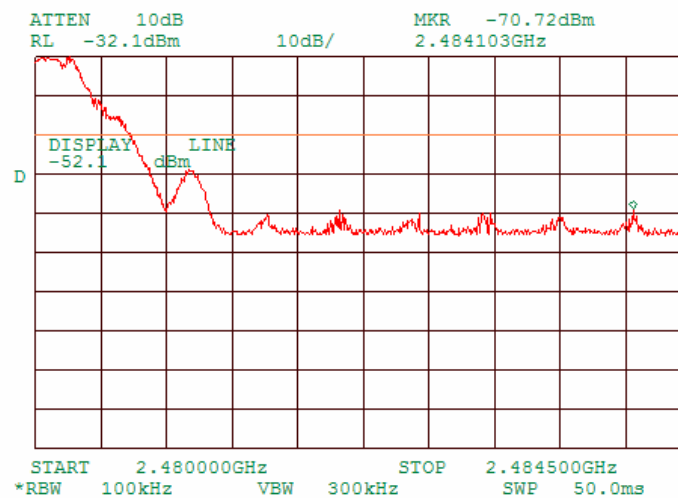
Plot 8.7.6 The highest band edge emission at high carrier frequency with hopping function enabled
