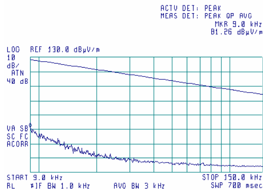
Plot 7.3.11 Radiated emission measurements from 9 to 150 kHz at the mid carrier frequency
