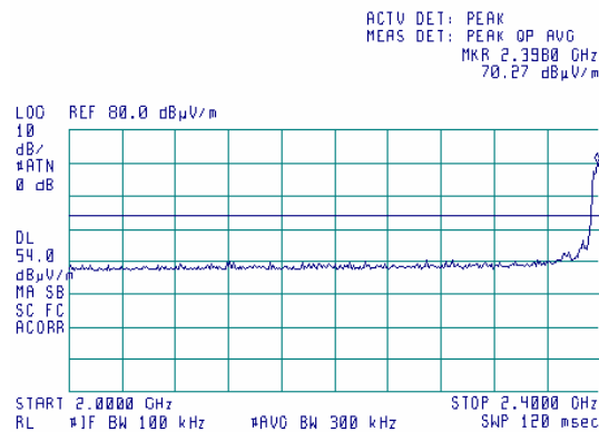
Plot 7.3.26 Radiated emission measurements from 2000 to 2400 MHz at the low carrier frequency
