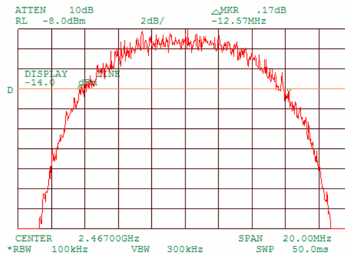
Plot 7.1.12 6 dB bandwidth test result at high frequency, 11 MBPS
