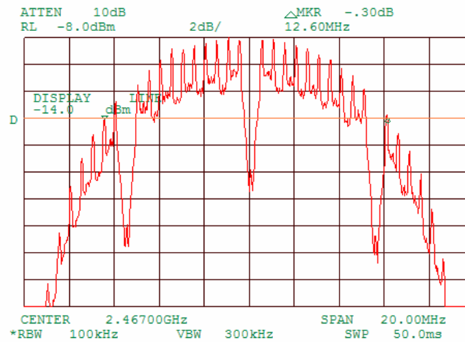
Plot 7.1.9 6 dB bandwidth test result at high frequency, 1 MBPS
