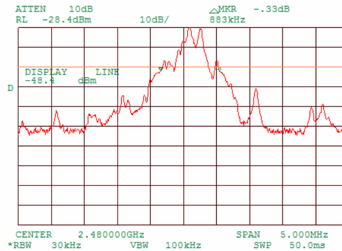
Plot 8.2.3 20 dB bandwidth test result at high frequency, 1 MBPS
