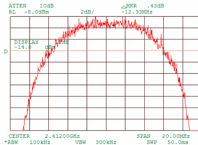
Plot 7.1.4 6 dB bandwidth test result at low frequency, 11 MBPS
