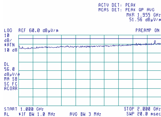
Plot 7.3.20 Radiated emission measurements from 1000 to 2000 MHz at the low carrier frequency
