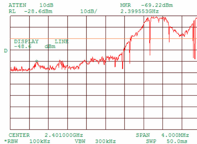
Plot 8.7.5 The highest band edge emission at low carrier frequency with hopping function enabled
