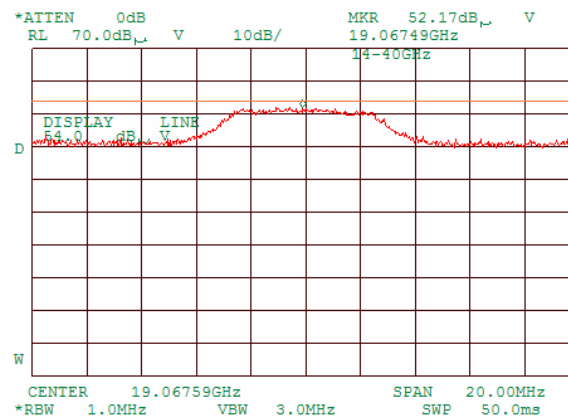
Plot 7.3.54 Radiated emission measurements at the spurious frequency at 19067.59 MHz
