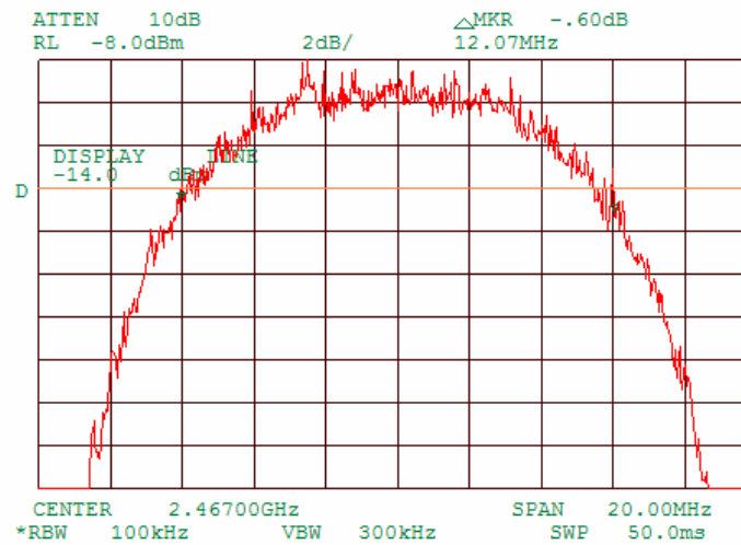
Plot 7.1.11 6 dB bandwidth test result at high frequency, 5.5 MBPS
