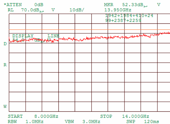
Plot 7.3.45 Radiated emission measurements from 8000 to 14000 MHz at the mid carrier frequency
