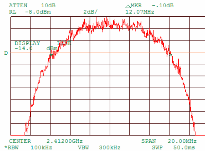
Plot 7.1.3 6 dB bandwidth test result at low frequency, 5.5 MBPS
