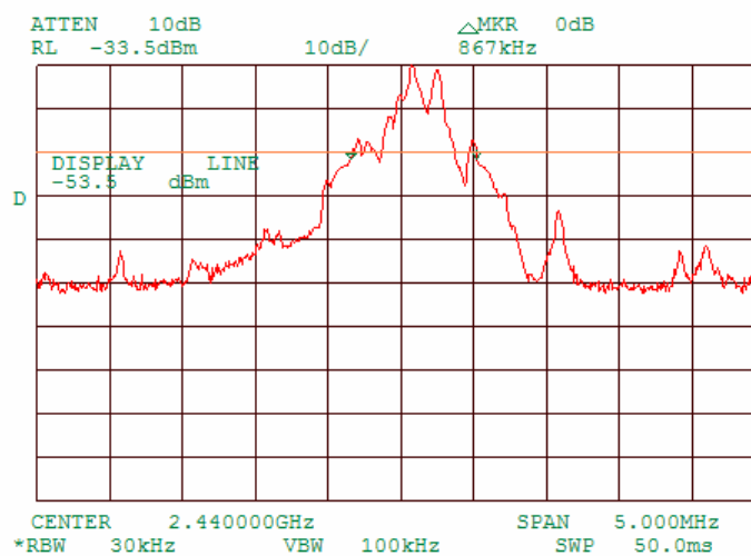
Plot 8.2.2 20 dB bandwidth test result at mid frequency, 1 MBPS
