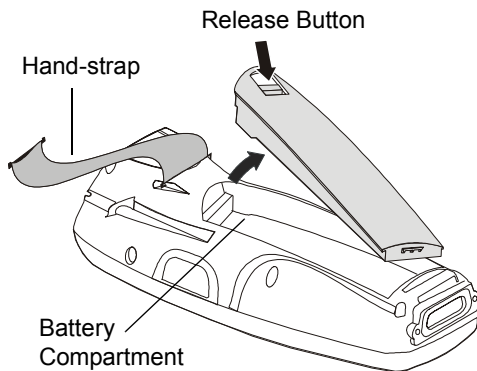
Figure 3. Battery Installation and Removal
