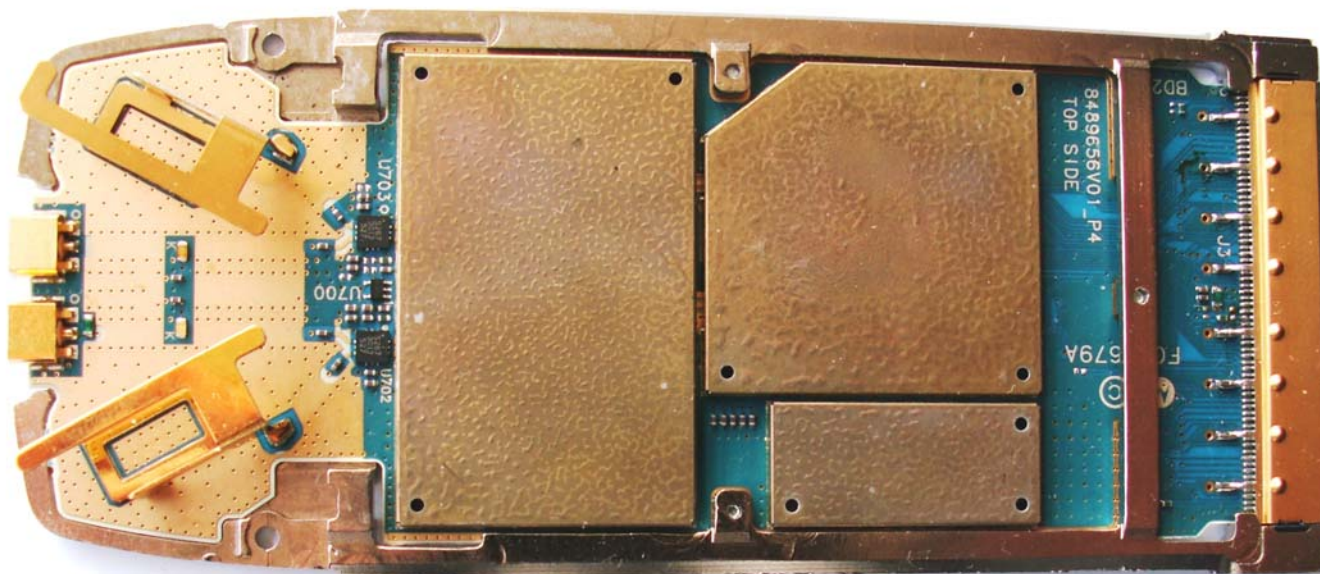
Photograph 9.1: Top view of WDE1000.
