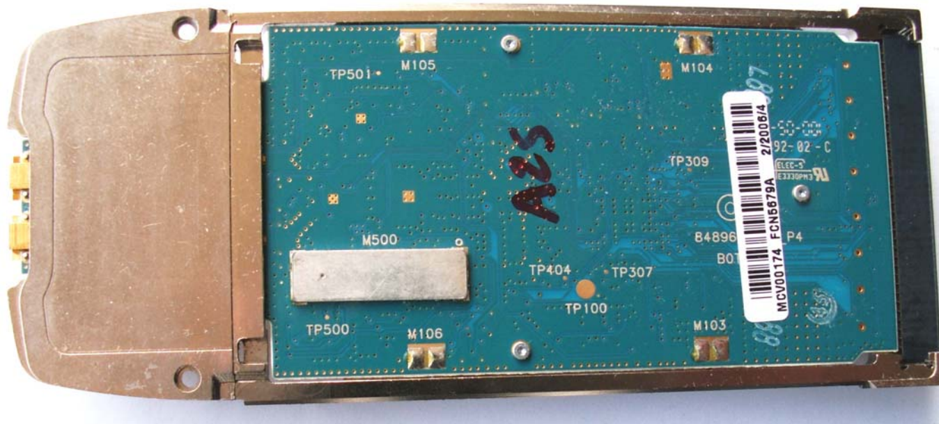
Photograph 9.3: Bottom view of WDE1000.
