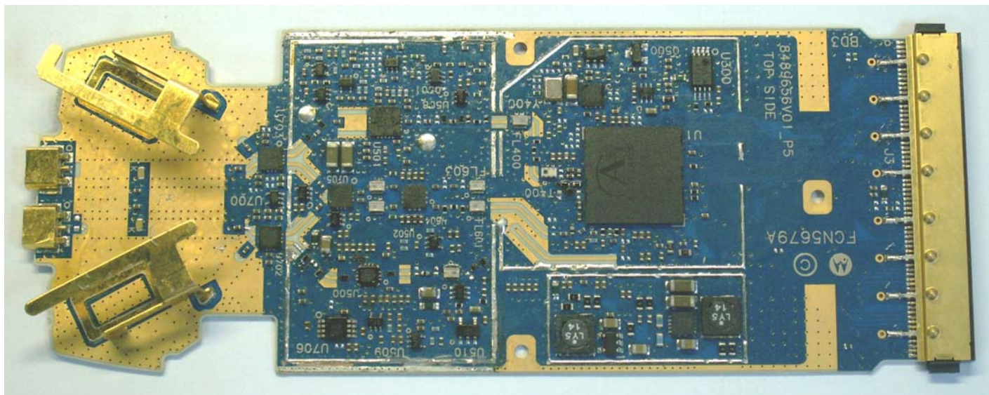
Photograph 9.2: Top view with cans ‘removed’ of WDE1000.
