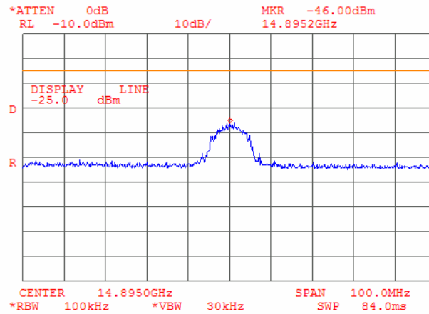
Plot 6.6.38: Tx Conducted spurious emission measurements at the 3 rd harmonic of mid carrier frequency, OBW 5 MHz
