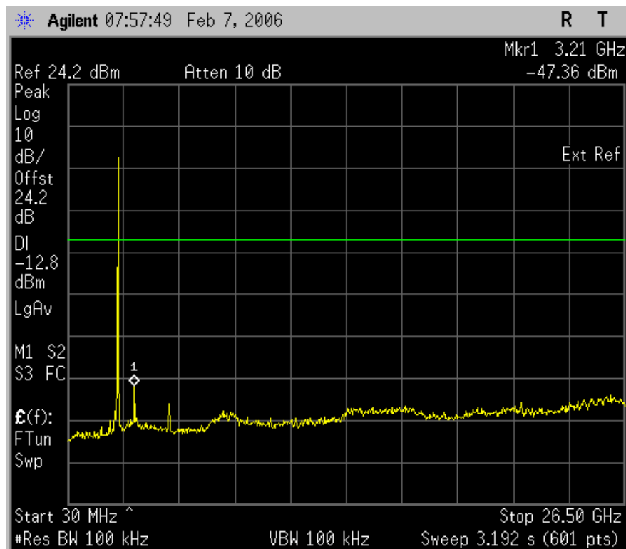
Plot 6.16.2: Tx Conducted emission measurements 0.03-26.5GHz at the low carrier frequency, 802.11b mode,
