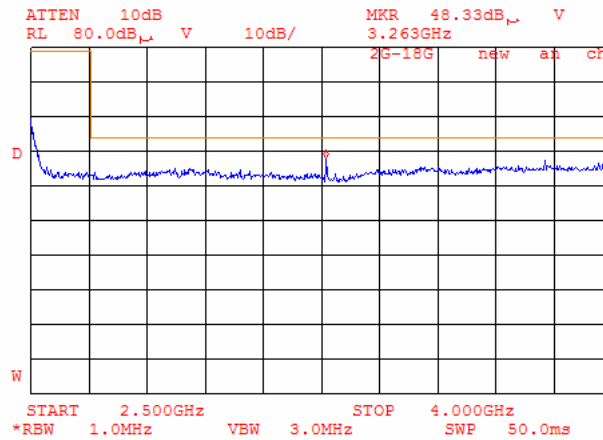
Plot 6.17.66: Tx Radiated emission measurements, 2500 - 4000MHz, at the mid* carrier frequency, 802.11g mode.
