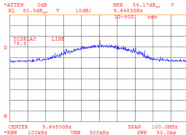
Plot 6.17.85: Tx Radiated emission measurement at 9648MHz, at the low carrier frequency, 802.11g mode.
