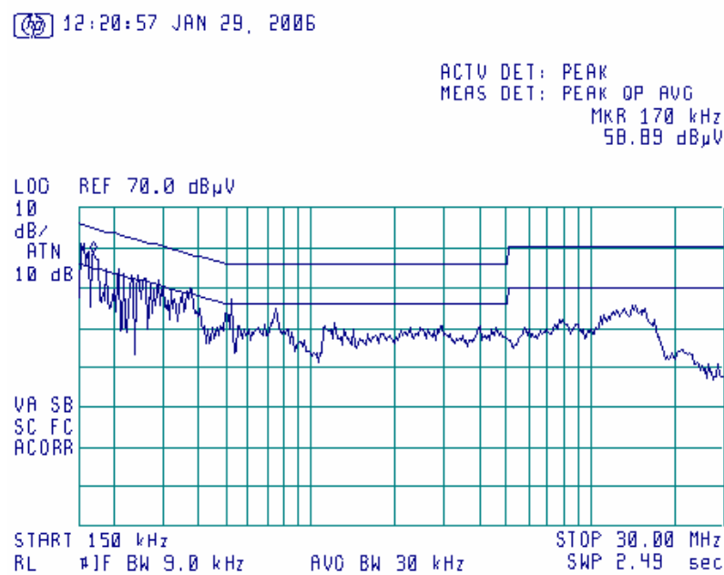
Plot 6.11.5: Conducted emission measurements, Transmit mode, Line L2, Quasi-Peak & Average Limits.
