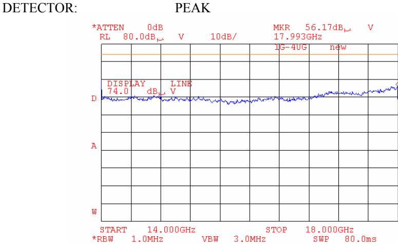
Plot 6.17.96: Tx Radiated emission measurements, 14 - 18GHz, at the high carrier frequency, 802.11g mode.
