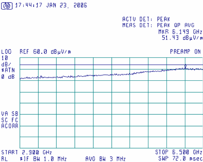
Plot 6.18.6: Rx Radiated Emission measurements in 2900 - 6500 MHz range, Vertical and Horizontal Antenna polarization.
