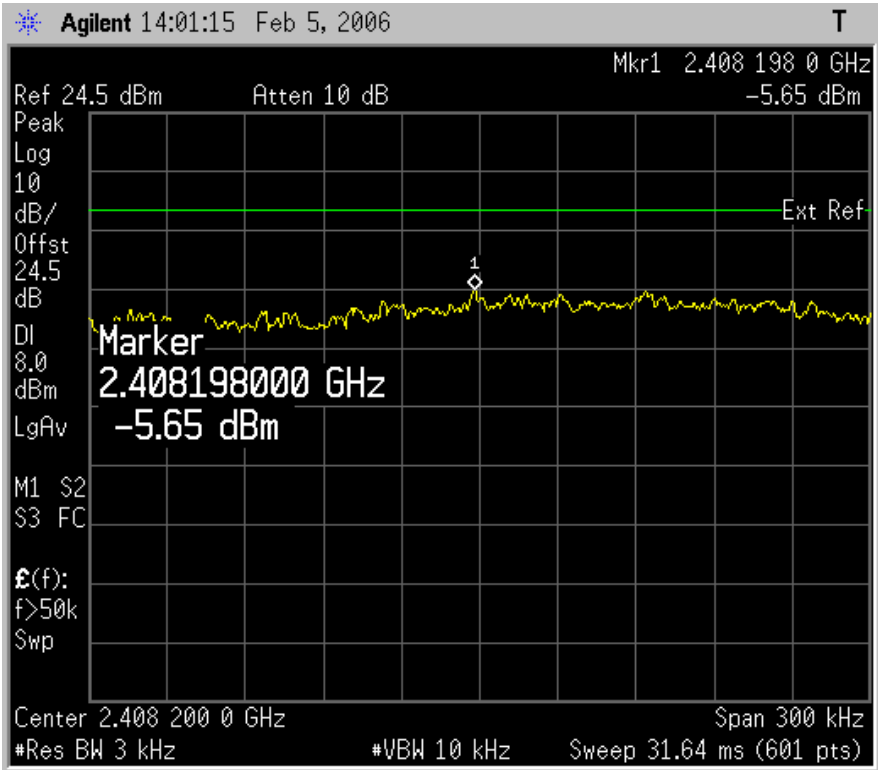
Plot 6.15.4: Peak Power Spectral Density at low carrier frequency, 54Mbps, 802.11g mode
