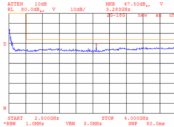
Plot 6.17.69: Tx Radiated emission measurements, 2500 - 4000MHz, at the high carrier frequency, 802.11g mode.
