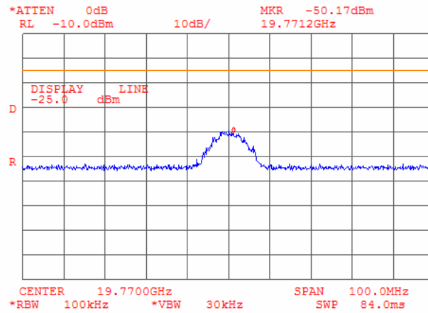
Plot 6.6.40: Tx Conducted spurious emission measurements at the 4 th harmonic of low carrier frequency, OBW 5 MHz
