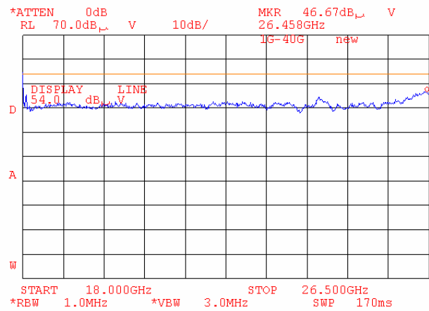
Plot 6.17.98: Tx Radiated emission measurements, 18 - 26.5GHz, at the low carrier frequency, 802.11g mode.
