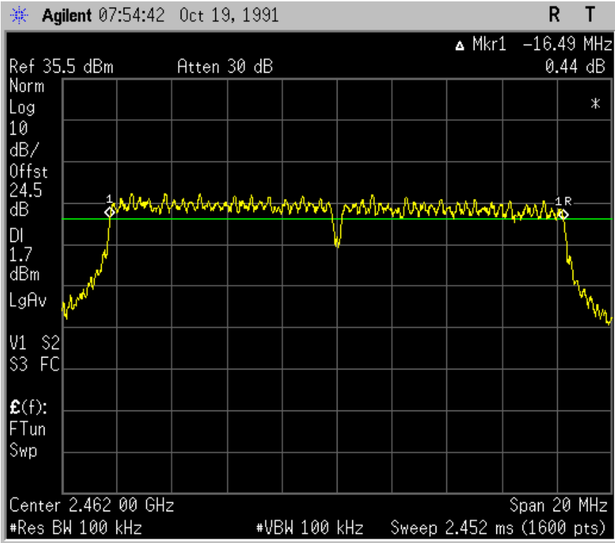
Plot 6.14.6: 6dB Bandwidth at CH11, 54Mbps, 802.11g mode
