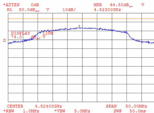
Plot 6.17.73: Tx Radiated emission measurement, at 4824MHz, at the low carrier frequency, 802.11g mode.
