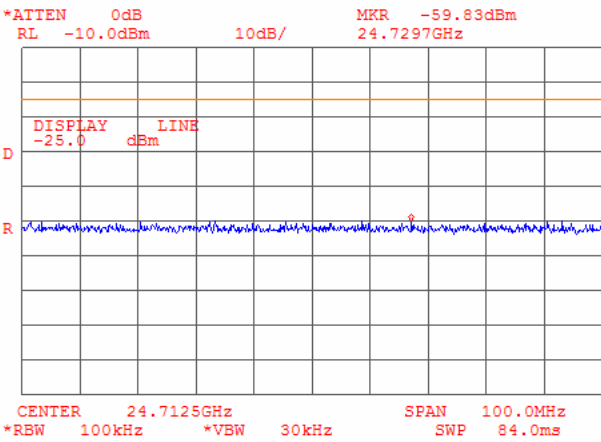
Plot 6.6.44: Tx Conducted spurious emission measurements at the 5 th harmonic of mid carrier frequency, OBW 5 MHz
