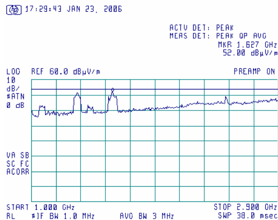
Plot 6.10.4: Rx Radiated Emission measurements in 1000-2900MHz range, Vertical Antenna polarization.
