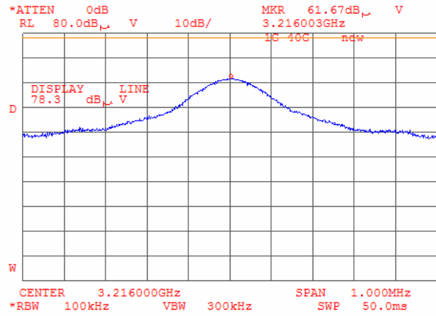
Plot 6.17.65: Tx Radiated emission measurement at 3216MHz, at the low carrier frequency, 802.11g mode.
