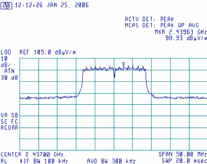
Plot 6.17.10: Tx Radiated emission measurements at the mid carrier frequency, 54Mbps, 802.11g mode, Horizontal polarization.
