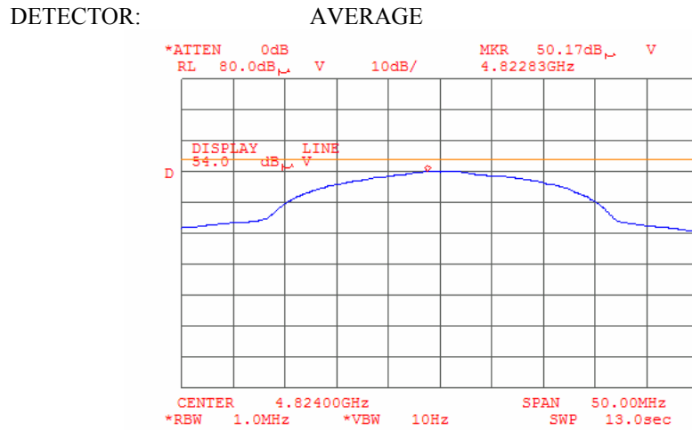
Plot 6.17.74: Tx Radiated emission measurement, at 4824MHz, at the low carrier frequency, 802.11g mode.
