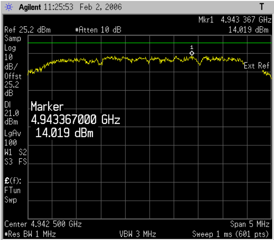
Plot 6.4.1: Peak Power Spectral Density, at low carrier frequency, OBW 5 MHz.
