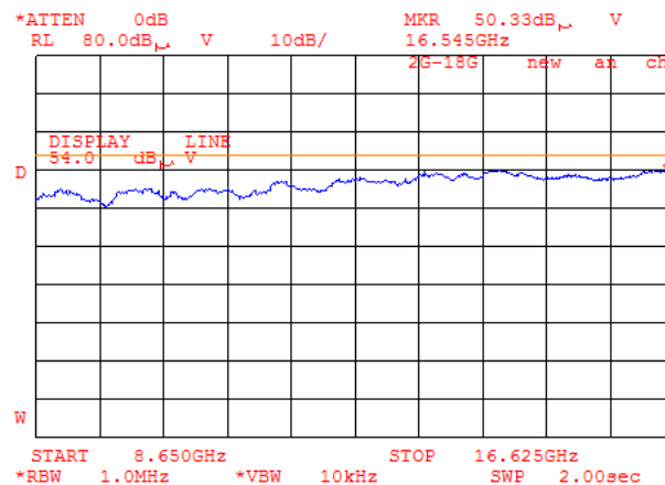
Plot 6.10.10: Rx Radiated Emission measurements in 8650-16625 MHz range, Vertical & Horizontal Antenna polarization.
