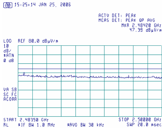
Plot 6.17.59: Tx Radiated emission measurements, 2483.5 - 2500MHz, at the high carrier frequency, 802.11g mode.
