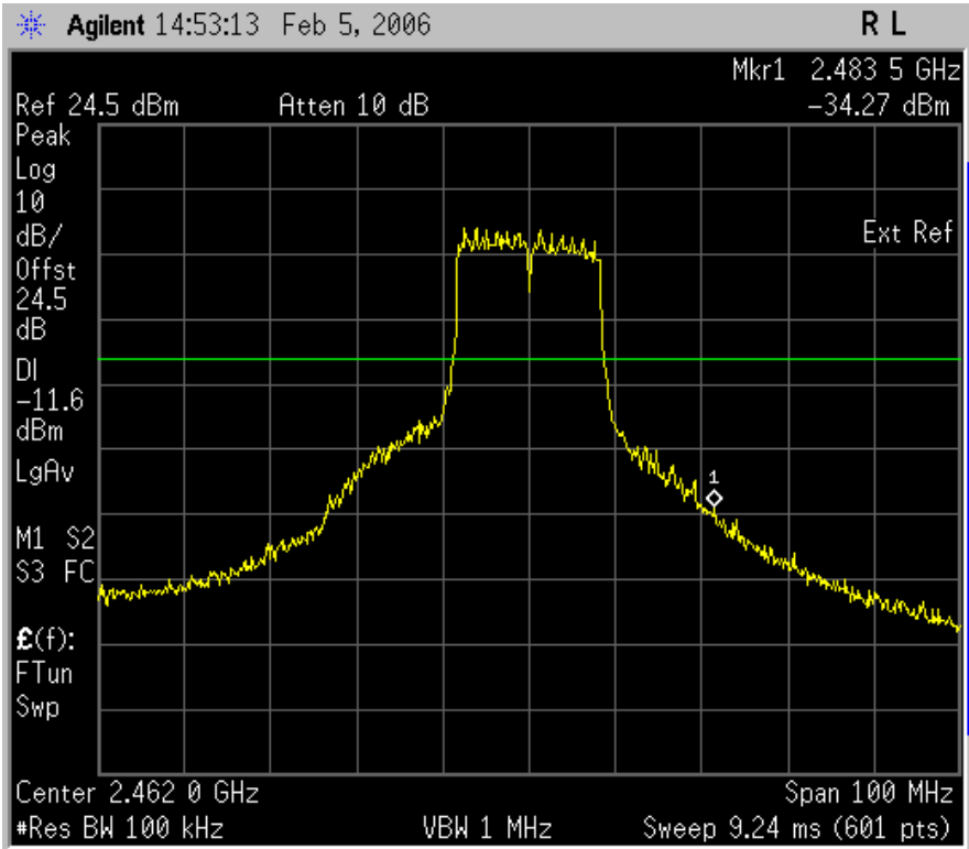
Plot 6.16.11: Tx Conducted emission measurement at the high carrier frequency, high band edge, 802.11g mode.
