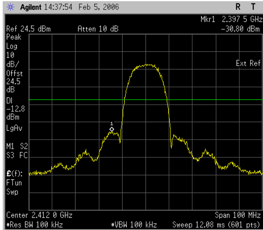
Plot 6.16.1: Tx Conducted emission measurement at the low carrier frequency, low band edge, 802.11b mode.
