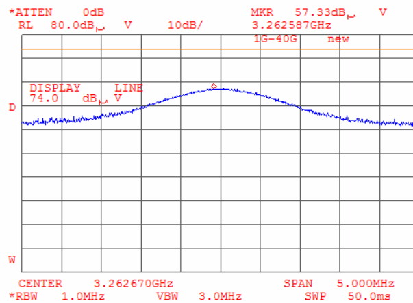
Plot 6.17.68: Tx Radiated emission measurement at 3262MHz, at the mid* carrier frequency, 802.11g mode.
