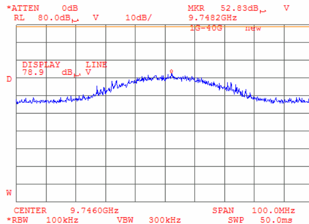
Plot 6.17.88: Tx Radiated emission measurement at 9748MHz, at the mid carrier frequency, 802.11g mode.
