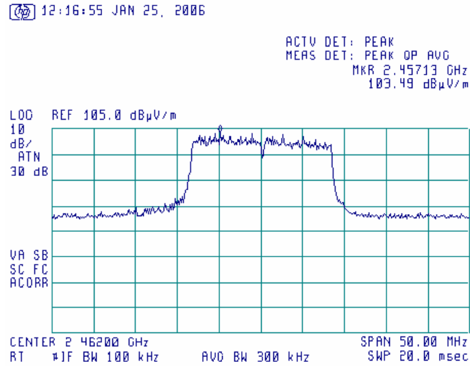
Plot 6.17.12: Tx Radiated emission measurements at the high carrier frequency, 54Mbps, 802.11g mode, Horizontal polarization.
