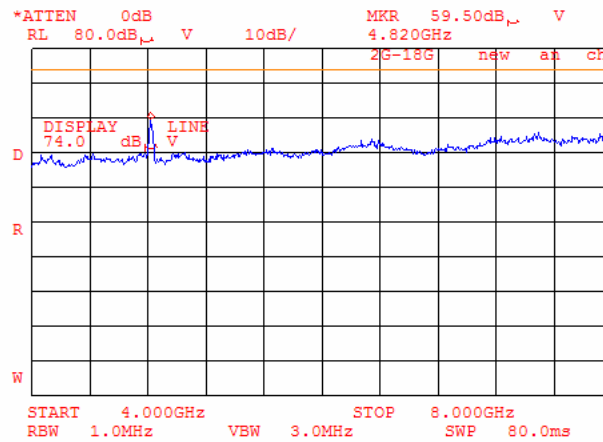
Plot 6.17.71: Tx Radiated emission measurements, 4000 - 8000MHz, at the low carrier frequency, 802.11g mode.
