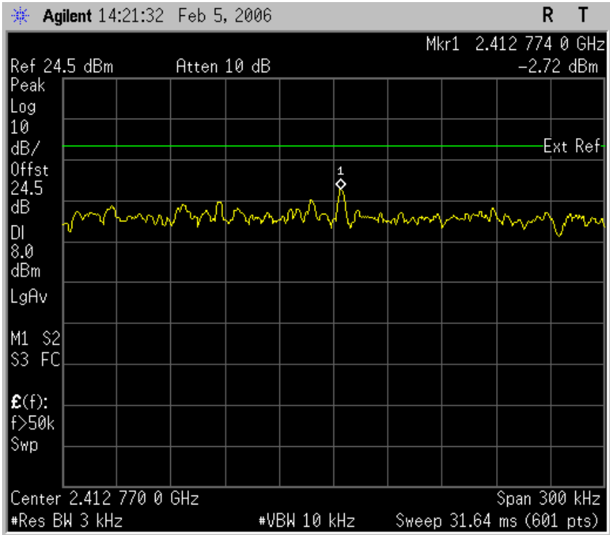
Plot 6.15.1: Peak Power Spectral Density at low carrier frequency, 11Mbps, 802.11b mode
