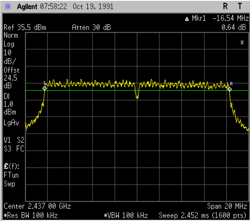
Plot 6.14.5: 6dB Bandwidth at CH6, 54Mbps, 802.11g mode
