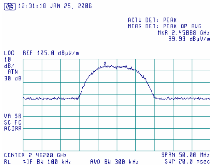
Plot 6.17.5: Tx Radiated emission measurements at the high carrier frequency, 11Mbps, 802.11b mode, Vertical polarization.
