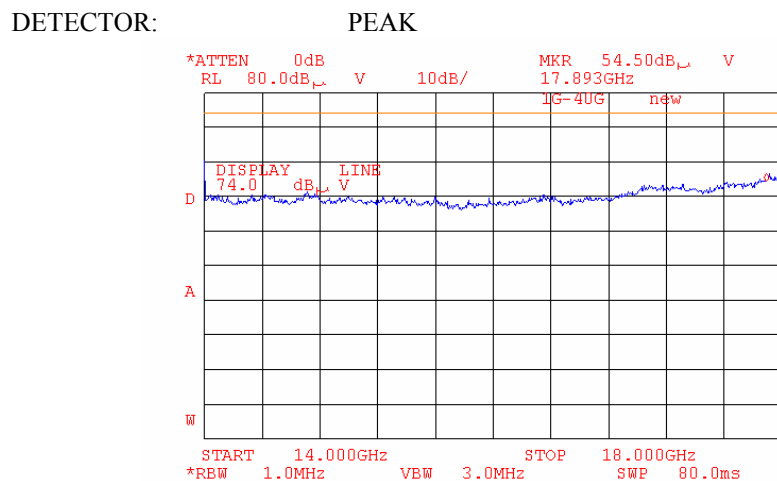
Plot 6.17.94: Tx Radiated emission measurements, 14 - 18GHz, at the mid carrier frequency, 802.11g mode.
