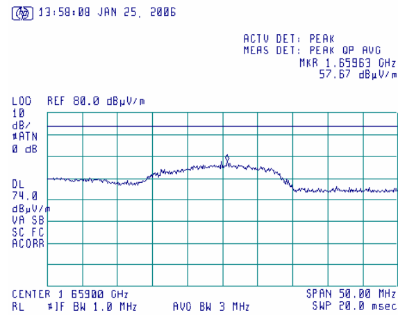
Plot 6.17.34: Tx Radiated emission measurement at 1659MHz, at the low carrier frequency, 802.11g mode.
