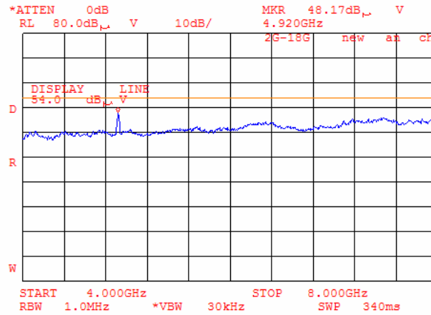
Plot 6.17.81: Tx Radiated emission measurement, at 4924MHz, at the high carrier frequency, 802.11g mode.
