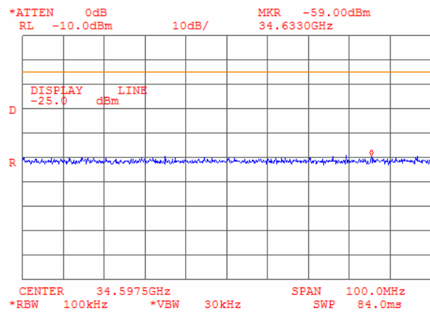
Plot 6.6.50: Tx Conducted spurious emission measurements at the 7 th harmonic of mid carrier frequency, OBW 5 MHz
