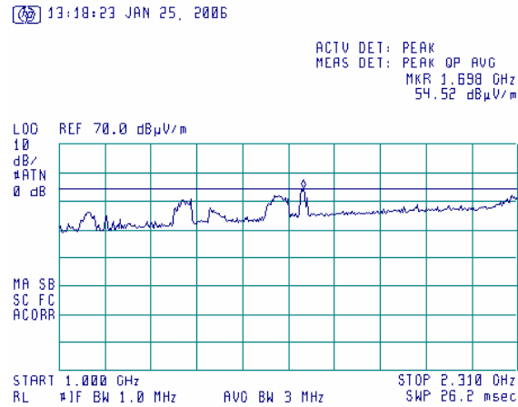
Plot 6.17.39: Tx Radiated emission measurement at 1698 MHz, at the mid carrier frequency, 802.11g mode.
