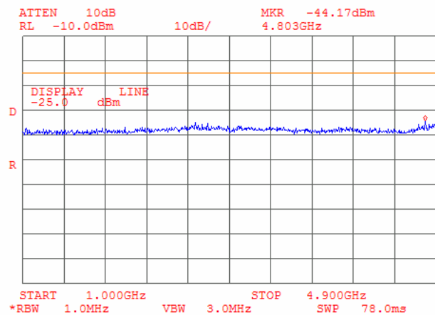
Plot 6.6.10: Tx Spurious emission measurements in 1000 - 4900 MHz range at low carrier frequency, OBW 5 MHz
