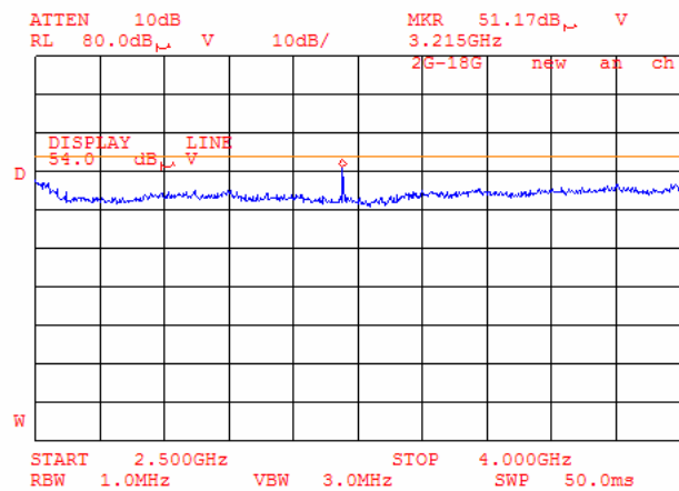
Plot 6.17.64: Tx Radiated emission measurements, 2500 - 4000MHz, at the low carrier frequency, 802.11g mode.
