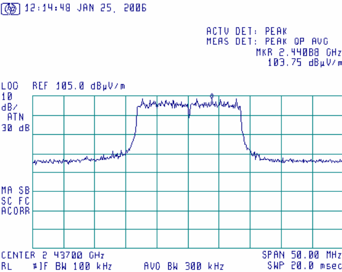
Plot 6.17.9: Tx Radiated emission measurements at the mid carrier frequency, 54Mbps, 802.11g mode, Vertical polarization.
