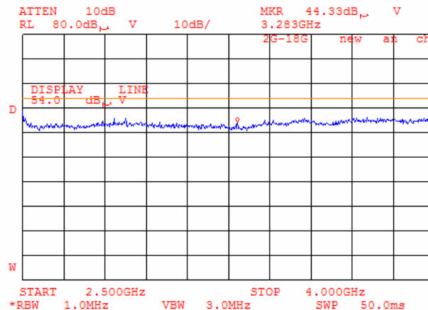
Plot 6.17.63: Tx Radiated emission measurements, 2500 - 4000MHz, at the high carrier frequency, 802.11b mode.
