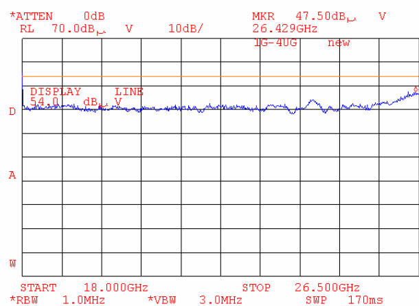
Plot 6.17.100: Tx Radiated emission measurements, 18 - 26.5GHz, at the high carrier frequency, 802.11g mode.
