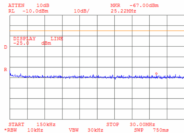
Plot 6.6.4: Tx Spurious emission measurements in 0.15 - 30.0 MHz range at low carrier frequency, OBW 5 MHz
