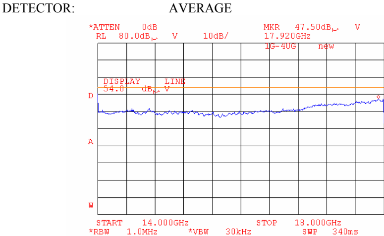
Plot 6.17.97: Tx Radiated emission measurements, 14 - 18GHz, at the high carrier frequency, 802.11g mode.
