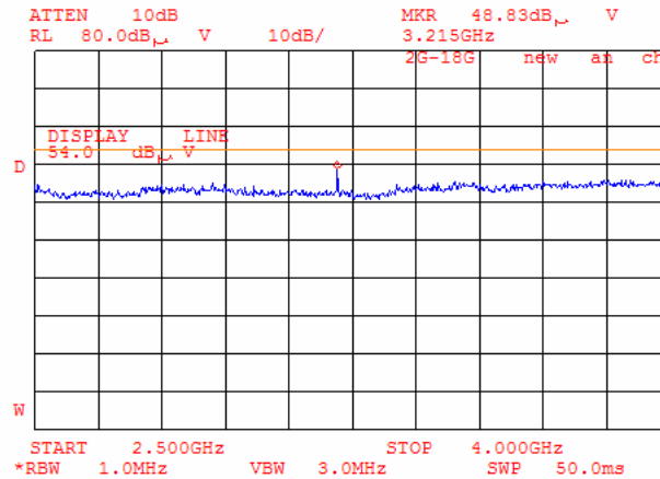
Plot 6.17.61: Tx Radiated emission measurements, 2500 - 4000MHz, at the low carrier frequency, 802.11b mode.
