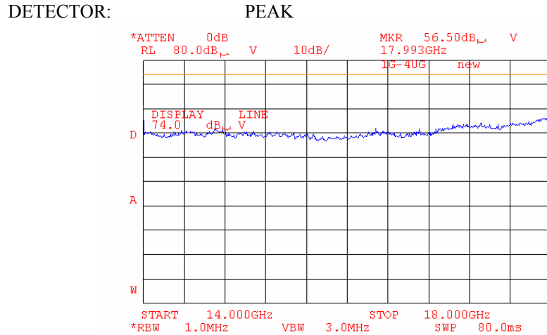
Plot 6.17.92: Tx Radiated emission measurements, 14 - 18GHz, at the low carrier frequency, 802.11g mode.
