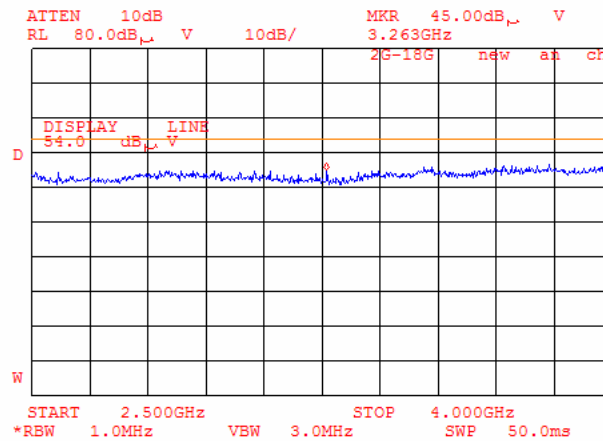
Plot 6.17.62: Tx Radiated emission measurements, 2500 - 4000MHz, at the mid carrier frequency, 802.11b mode.
