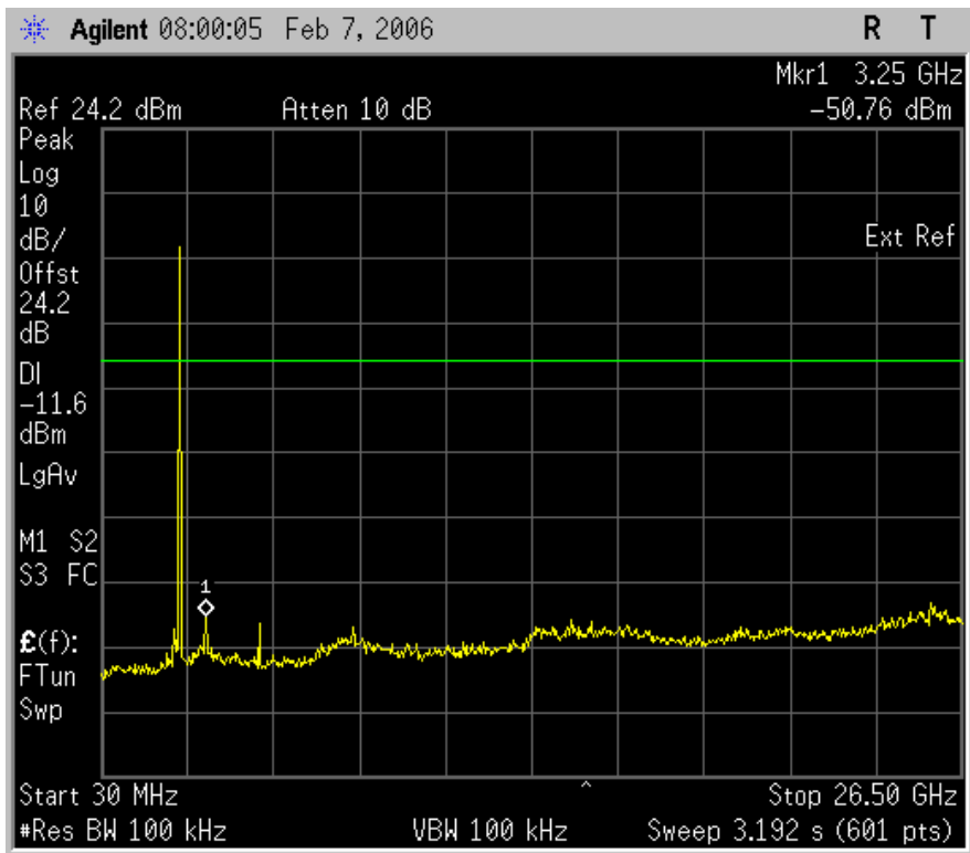
Plot 6.16.4: Tx Conducted emission measurements 0.03-26.5GHz at the mid carrier frequency, 802.11b mode,
