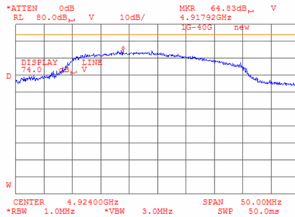
Plot 6.17.82: Tx Radiated emission measurement, at 4924MHz, at the high carrier frequency, 802.11g mode.
