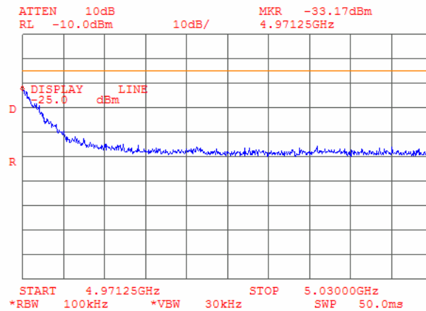
Plot 6.6.23: Tx Spurious emission measurements in 4971.25 – 5030 MHz range at mid carrier frequency, OBW 5 MHz
