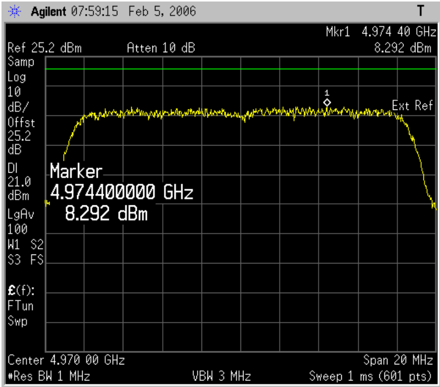
Plot 6.4.9: Peak Power Spectral Density, at high carrier frequency, OBW 20 MHz.
