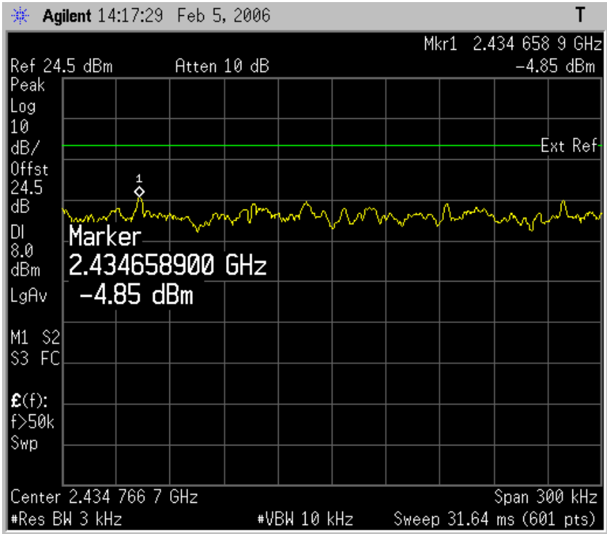
Plot 6.15.2: Peak Power Spectral Density at mid carrier frequency, 11Mbps, 802.11b mode
