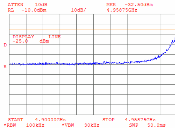
Plot 6.6.14: Tx Spurious emission measurements in 4900 – 4958.75 MHz range at mid carrier frequency, OBW 5 MHz
