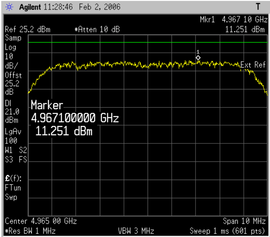
Plot 6.4.5: Peak Power Spectral Density, at mid carrier frequency, OBW 10 MHz.
