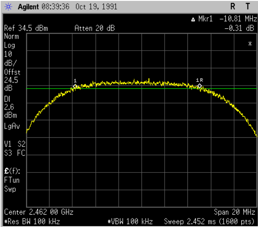
Plot 6.14.3: 6dB Bandwidth at CH11, 11Mbps, 802.11b mode
