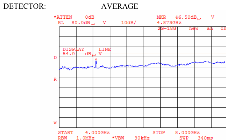
Plot 6.17.76: Tx Radiated emission measurements, 4000 - 8000MHz, at the mid carrier frequency, 802.11g mode.
