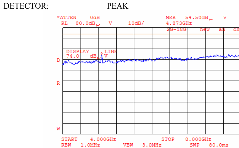
Plot 6.17.75: Tx Radiated emission measurements, 4000 - 8000MHz, at the mid carrier frequency, 802.11g mode.
