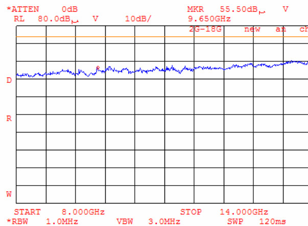
Plot 6.17.83: Tx Radiated emission measurements, 8000 - 14000MHz, at the low carrier frequency, 802.11g mode.
