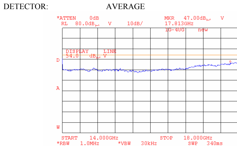
Plot 6.17.93: Tx Radiated emission measurements, 14 - 18GHz, at the low carrier frequency, 802.11g mode.
