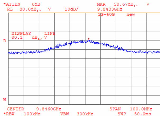
Plot 6.17.91: Tx Radiated emission measurement at 9848MHz, at the high carrier frequency, 802.11g mode.
