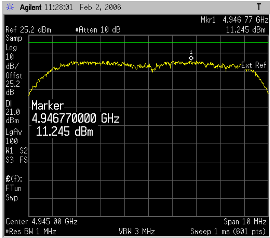
Plot 6.4.4: Peak Power Spectral Density, at low carrier frequency, OBW 10 MHz.
