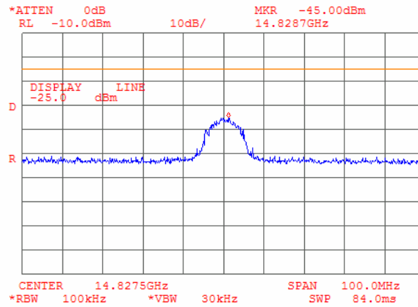
Plot 6.6.37: Tx Conducted spurious emission measurements at the 3 rd harmonic of low carrier frequency, OBW 5 MHz
