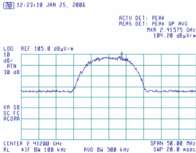
Plot 6.17.1: Tx Radiated emission measurements at the low carrier frequency, 11Mbps, 802.11b mode, Vertical polarization.
