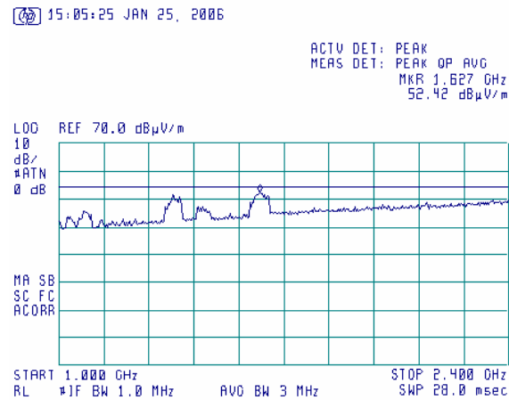
Plot 6.17.31: Tx Radiated emission measurements, 1000 - 2400 MHz at the high carrier frequency, 802.11b mode.
