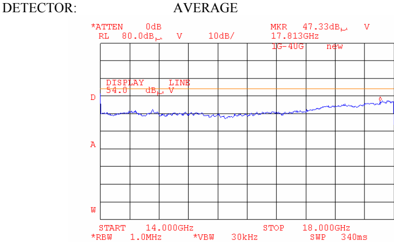
Plot 6.17.95: Tx Radiated emission measurements, 14 - 18GHz, at the mid carrier frequency, 802.11g mode.
