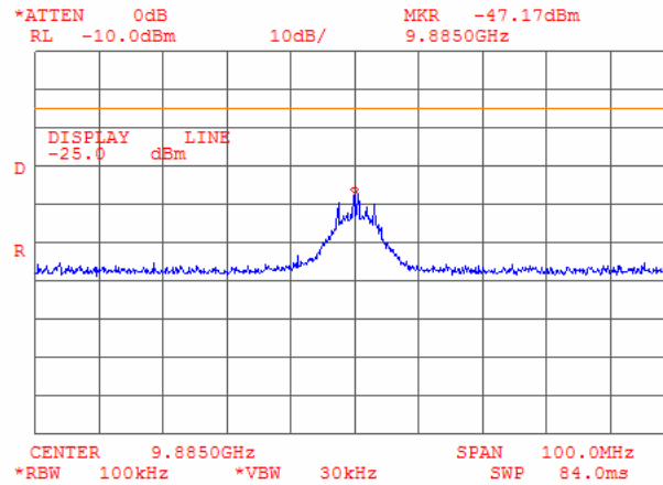
Plot 6.6.34: Tx Conducted spurious emission measurements at the 2 nd harmonic of low carrier frequency, OBW 5 MHz
