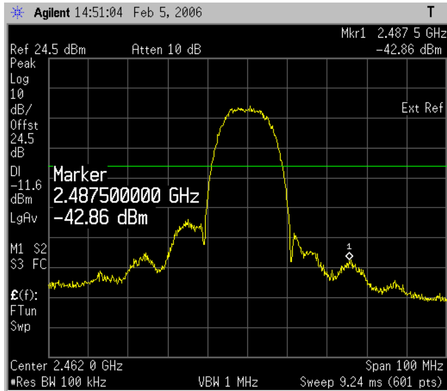
Plot 6.16.5: Tx Conducted emission measurement at the high carrier frequency, high band edge, 802.11b mode.
