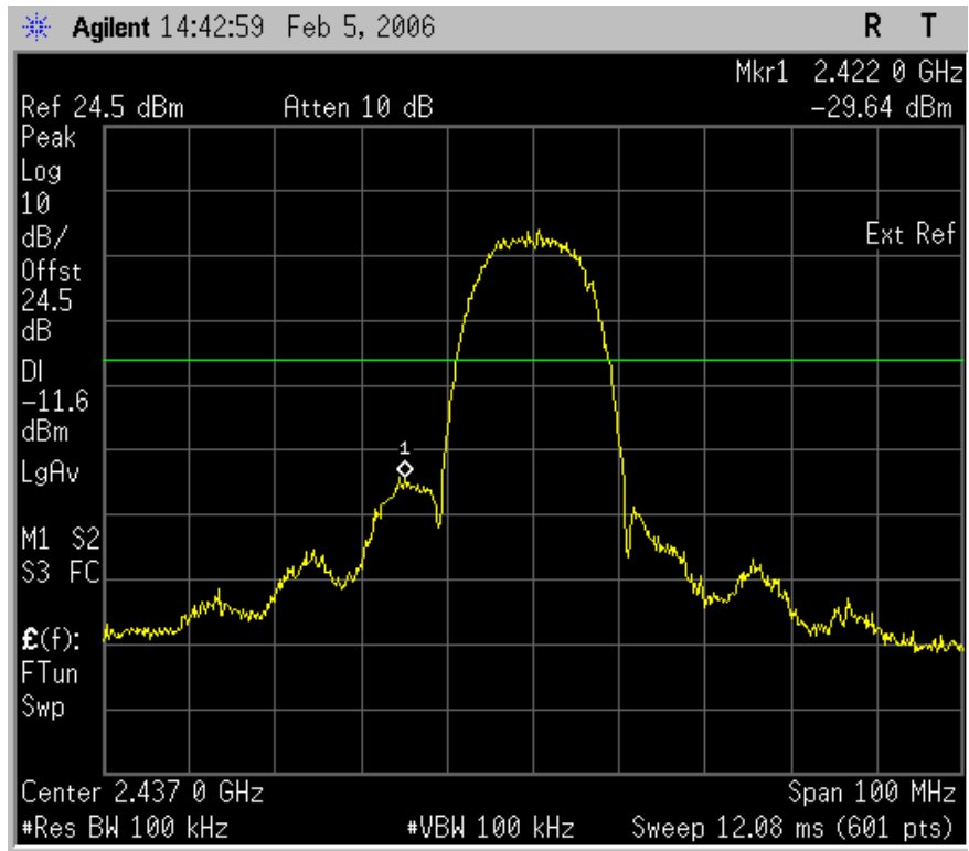
Plot 6.16.3: Tx Conducted emission measurement at the mid carrier frequency, 802.11b mode.
