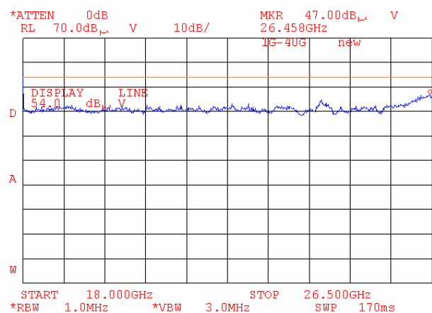
Plot 6.17.99: Tx Radiated emission measurements, 18 - 26.5GHz, at the mid carrier frequency, 802.11g mode.
