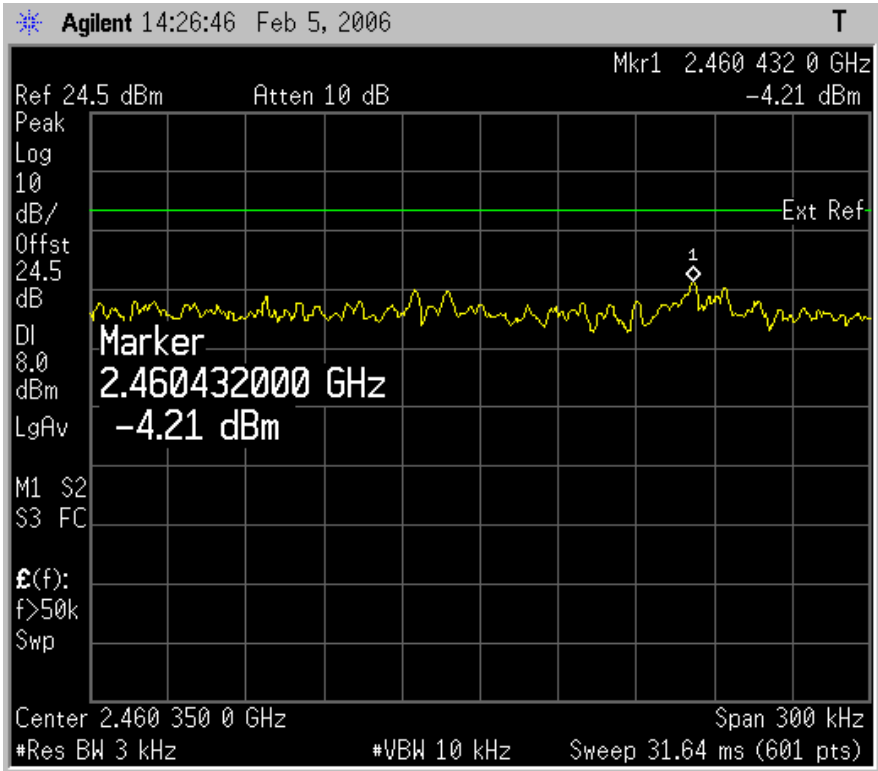
Plot 6.15.3: Peak Power Spectral Density at high carrier frequency, 11Mbps, 802.11b mode
