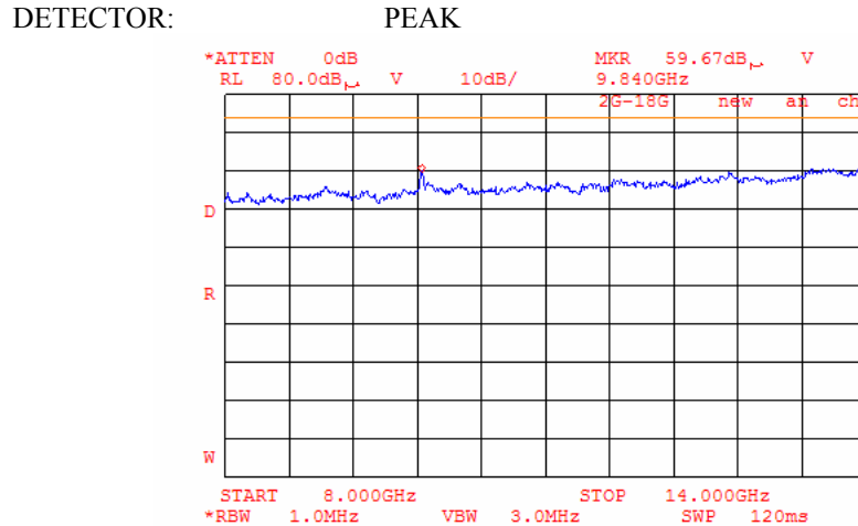
Plot 6.17.89: Tx Radiated emission measurements, 8000 - 14000MHz, at the high carrier frequency, 802.11g mode.
