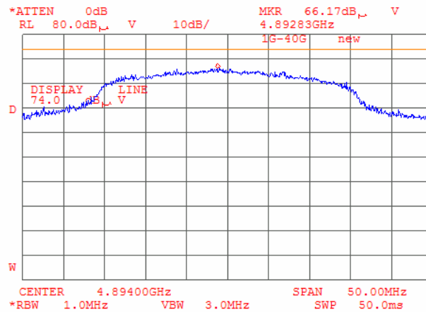
Plot 6.17.78: Tx Radiated emission measurement, at 4894MHz, at the mid carrier frequency, 802.11g mode.
