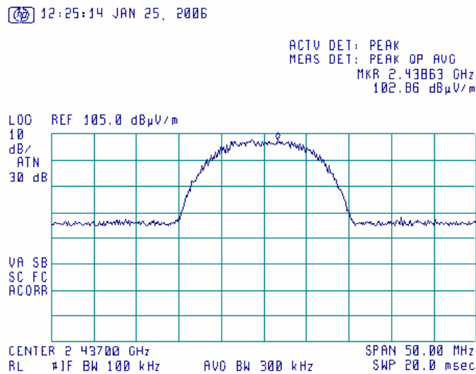
Plot 6.17.3: Tx Radiated emission measurements at the mid carrier frequency, 11Mbps, 802.11b mode, Vertical polarization.
