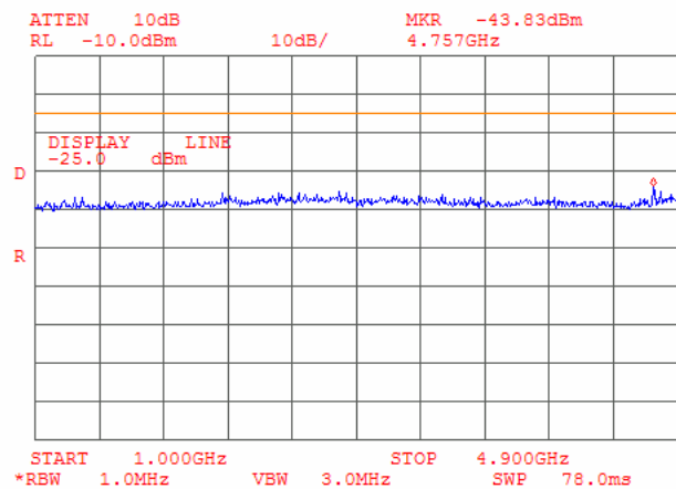
Plot 6.6.11: Tx Spurious emission measurements in 1000 - 4900 MHz range at mid carrier frequency, OBW 5 MHz
