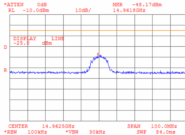
Plot 6.6.39: Tx Conducted spurious emission measurements at the 3 rd harmonic of high carrier frequency, OBW 5 MHz
