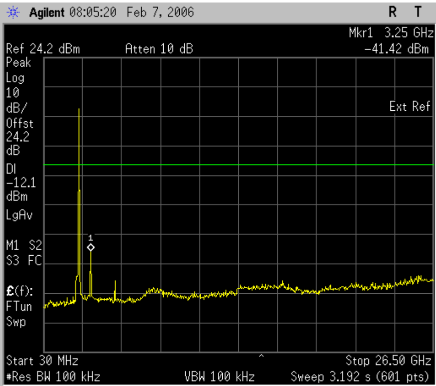
Plot 6.16.10: Tx Conducted emission measurements 0.03-26.5GHz at the mid carrier frequency, 802.11g mode,
