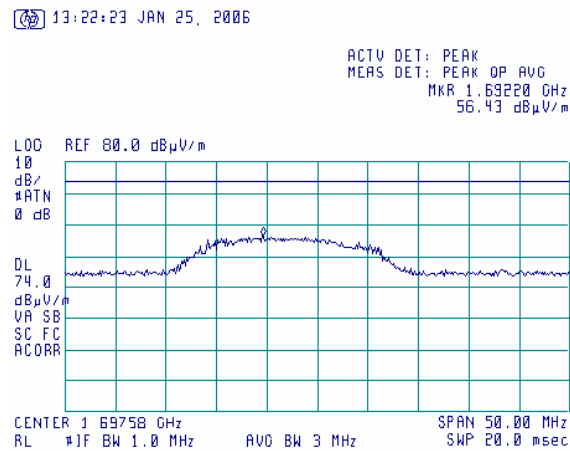
Plot 6.17.40: Tx Radiated emission measurement at 1698 MHz, at the mid carrier frequency, 802.11g mode.
