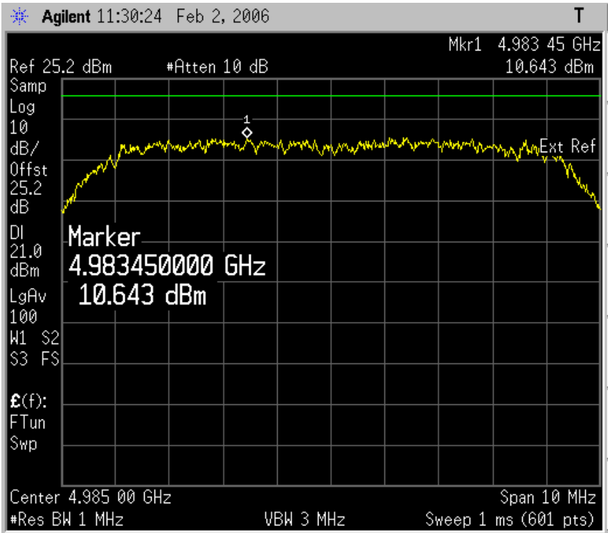
Plot 6.4.6: Peak Power Spectral Density, at high carrier frequency, OBW 10 MHz.
