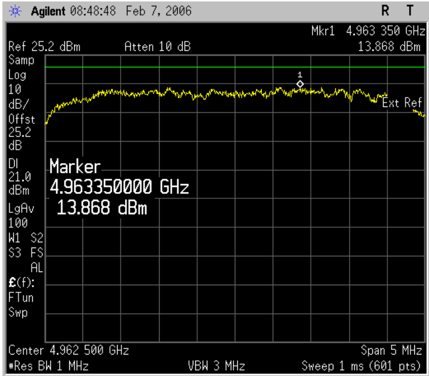
Plot 6.4.2: Peak Power Spectral Density, at mid carrier frequency, OBW 5 MHz.
