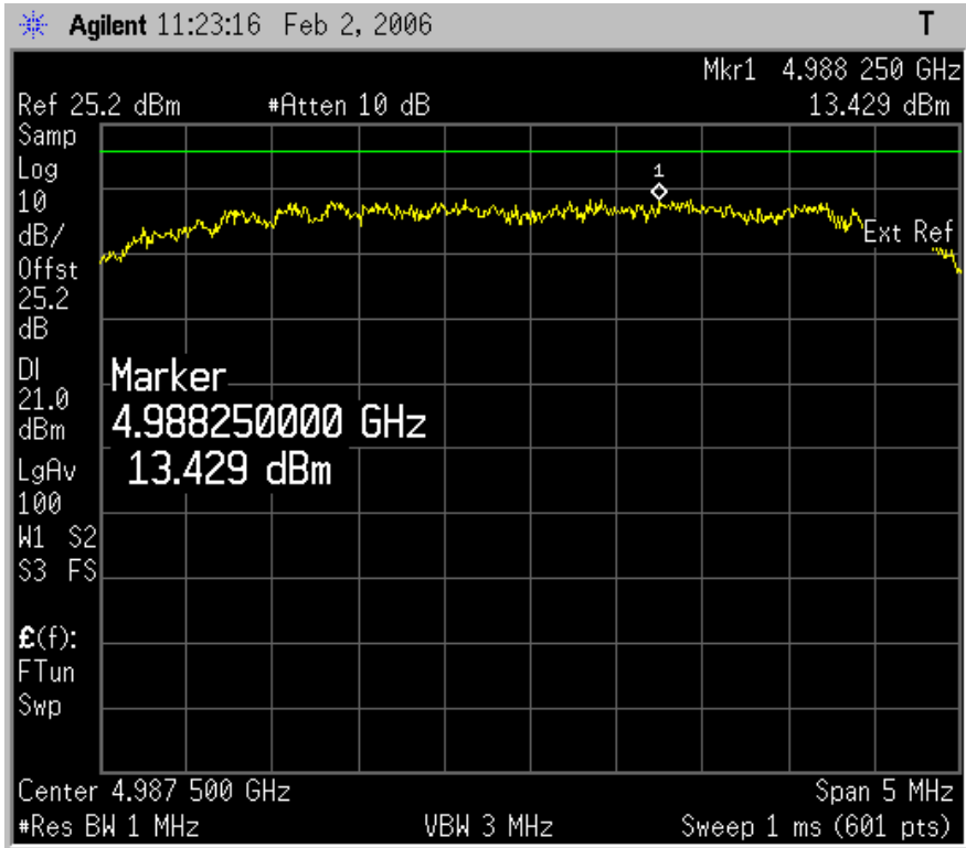
Plot 6.4.3: Peak Power Spectral Density, at high carrier frequency, OBW 5 MHz.
