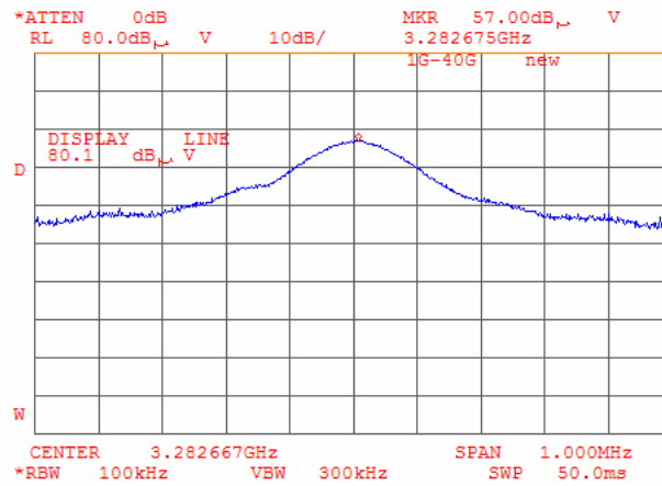
Plot 6.17.70: Tx Radiated emission measurement at 3283MHz, at the high carrier frequency, 802.11g mode.
