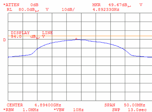
Plot 6.17.79: Tx Radiated emission measurements, 4000 - 8000MHz, at the high carrier frequency, 802.11g mode.
