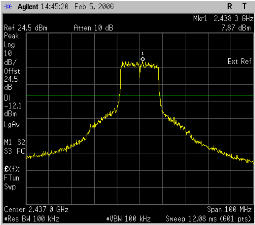
Plot 6.16.9: Tx Conducted emission measurement at the mid carrier frequency, 802.11g mode.
