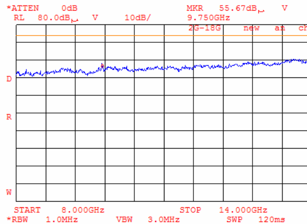
Plot 6.17.86: Tx Radiated emission measurements, 8000 - 14000MHz, at the mid carrier frequency, 802.11g mode.
