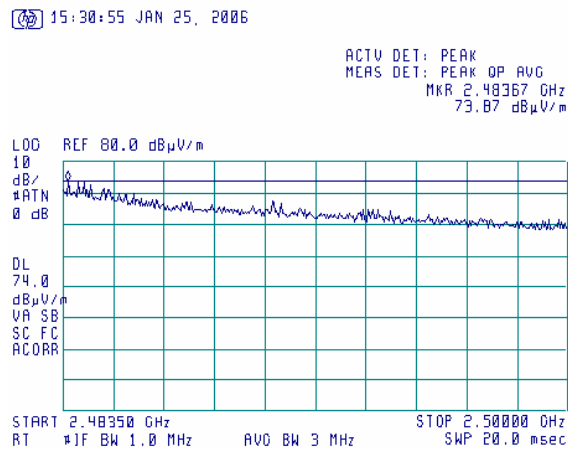
Plot 6.17.60: Tx Radiated emission measurements, 2483.5 - 2500MHz, at the high carrier frequency, 802.11g mode.
