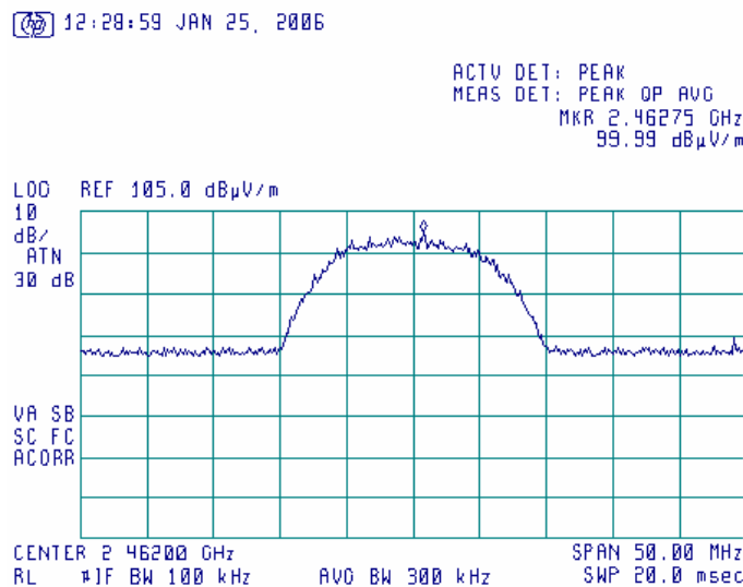
Plot 6.17.6: Tx Radiated emission measurements at the high carrier frequency, 11Mbps, 802.11b mode, Horizontal polarization.
