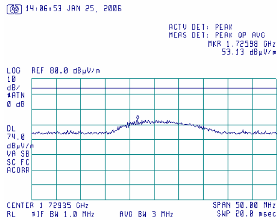
Plot 6.17.46: Tx Radiated emission measurement at 1729 MHz, at the high carrier frequency, 802.11g mode.
