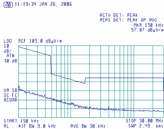
Plot 6.17.17: Tx Radiated emission measurements, 0.15 - 30 MHz at the high carrier frequency, 802.11g mode.
