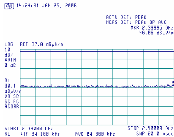
Plot 6.17.48: Tx Radiated emission measurements, 2390 - 2400MHz, at the high carrier frequency, 802.11g mode.
