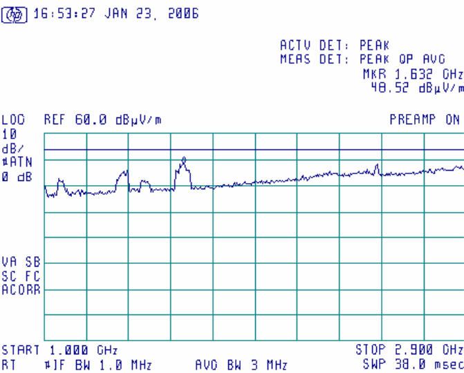
Plot 6.18.5: Rx Radiated Emission measurements in 1000 - 2900 MHz range, Horizontal Antenna polarization.
