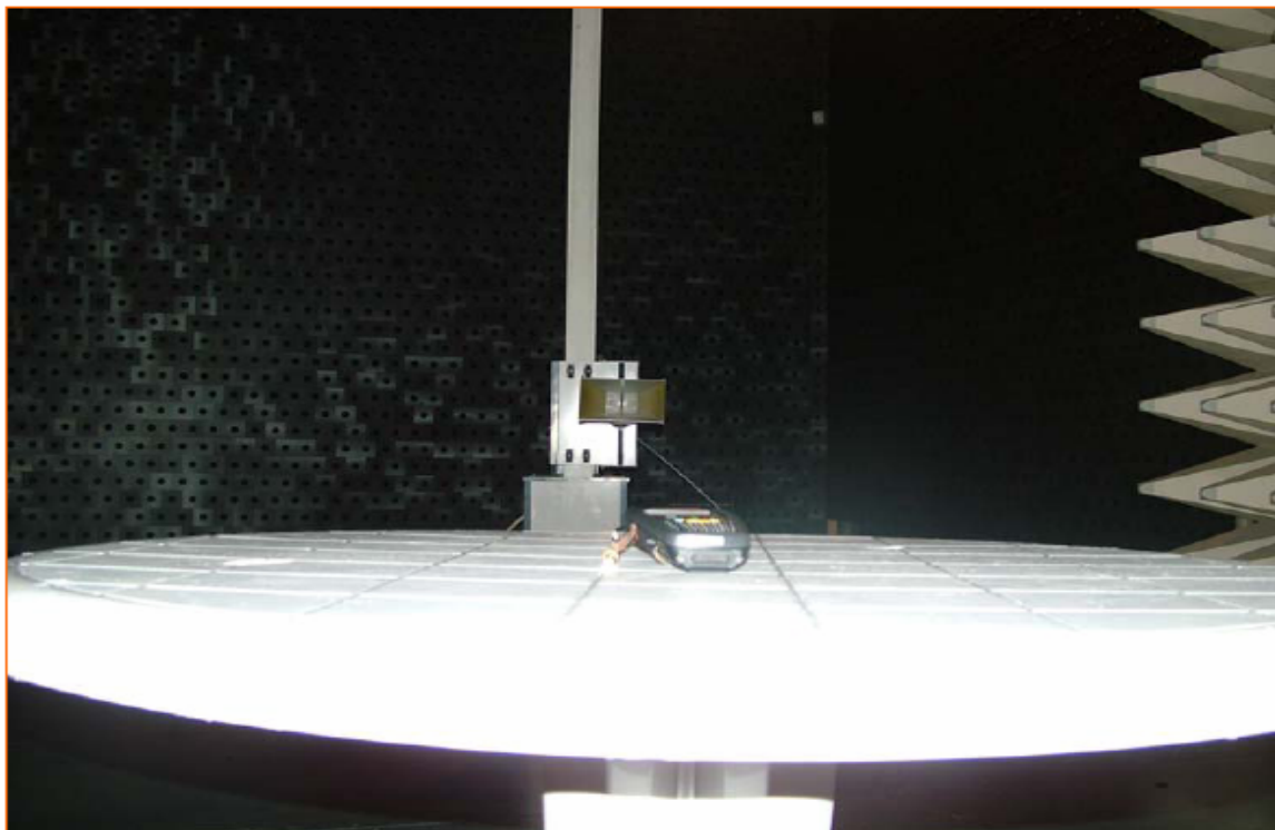
Photograph 4: Radiated measurements
