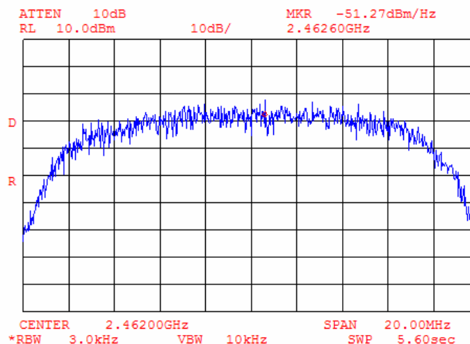
Plot 9.4.23 Peak spectral power density at high frequency within 6 dB band, bit rate 11 Mbps
