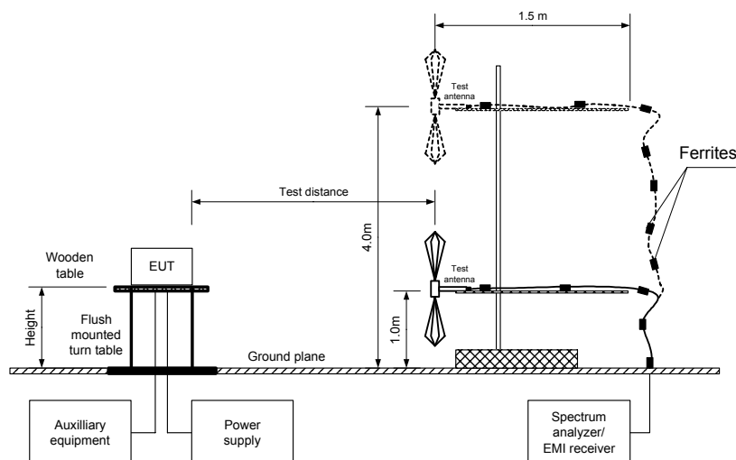
Figure 9.3.2 Setup for spurious emission field strength measurements above 30 MHz
