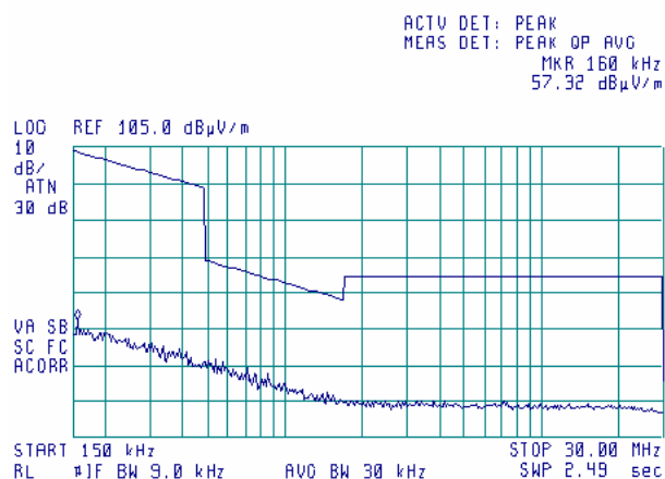
Plot 8.8.14 Radiated emission measurements from 0.15 to 30 MHz at the mid carrier frequency (BT+G20-1900)
