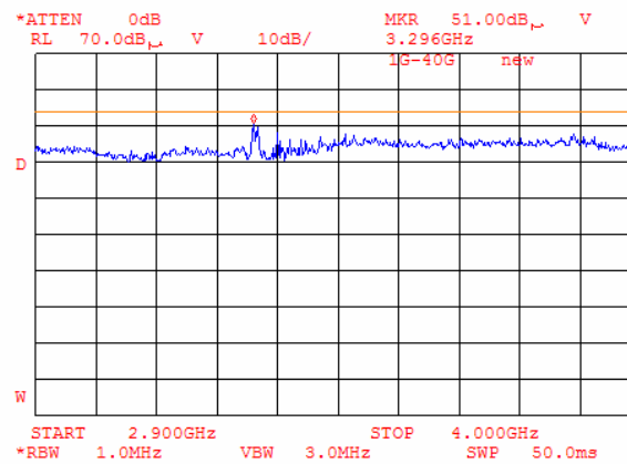
Plot 8.8.79 Radiated emission measurements at 3296 MHz at the low carrier frequency (BT and G20-850)
