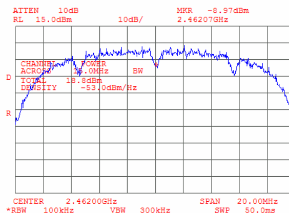
Plot 9.2.10 Peak output power at high frequency, Bit Rate 2 Mbps
