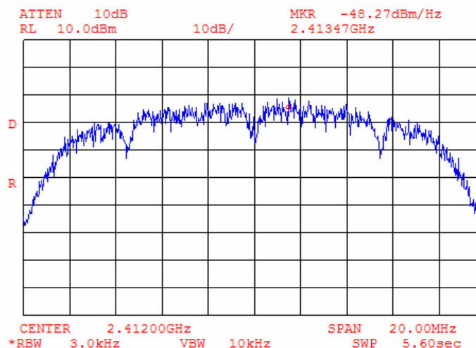
Plot 9.4.3 Peak spectral power density at low frequency within 6 dB band, bit rate 2 Mbps
