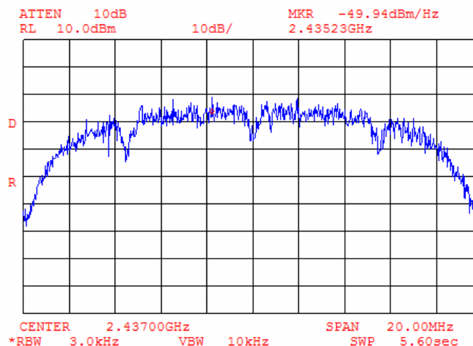
Plot 9.4.9 Peak spectral power density at mid frequency within 6 dB band, bit rate 1 Mbps
