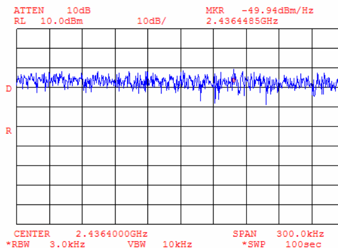
Plot 9.4.12 Peak spectral power density at mid frequency zoomed at the peak, bit rate 2 Mbps
