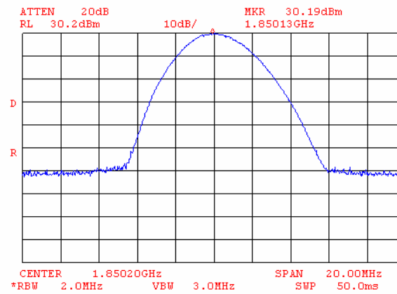
Plot 7.3.10 Occupied bandwidth test result at low frequency, reference level
