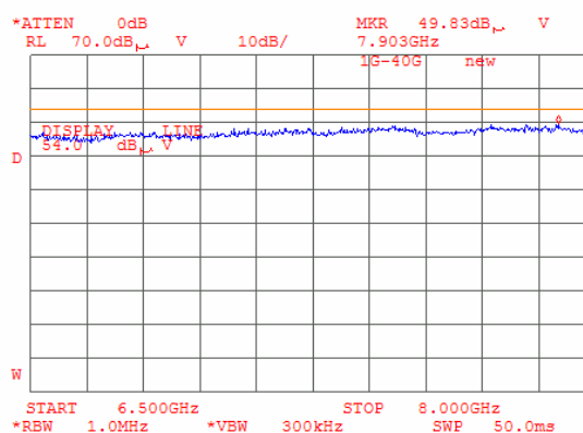
Plot 9.3.48 Radiated emission measurements from 6500 to 8000 MHz at the mid carrier frequency (WLAN + BT)
