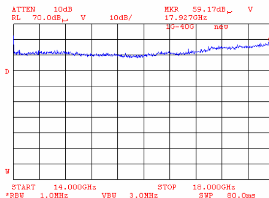
Plot 8.8.134 Radiated emission measurements from 14000 to 18000 MHz at the high carrier frequency (BT and G20-850)
