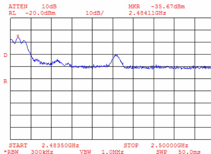
Plot 8.7.4 The highest band edge emission at high carrier frequency with hopping function disabled
