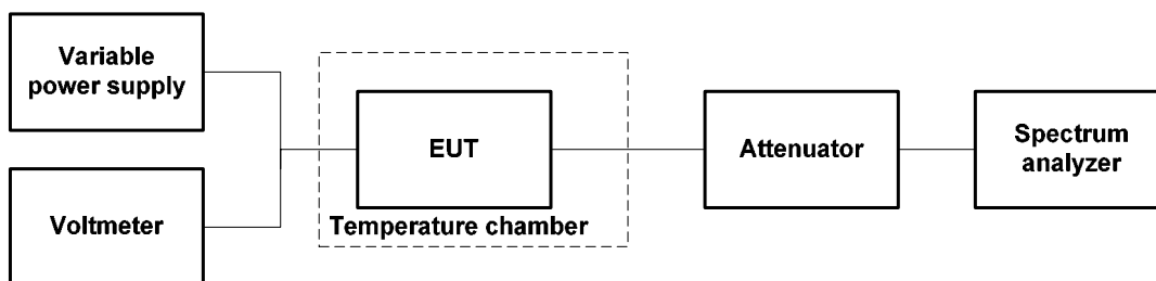
Figure 7.4.1 Frequency stability test setup
