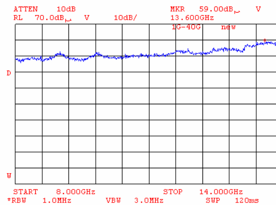
Plot 8.8.120 Radiated emission measurements from 8000 to 14000 MHz at the mid carrier frequency (BT and G20-850)
