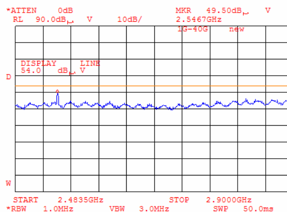
Plot 8.8.73 Radiated emission measurements at 2546 MHz at the high carrier frequency (BT and G20-850)
