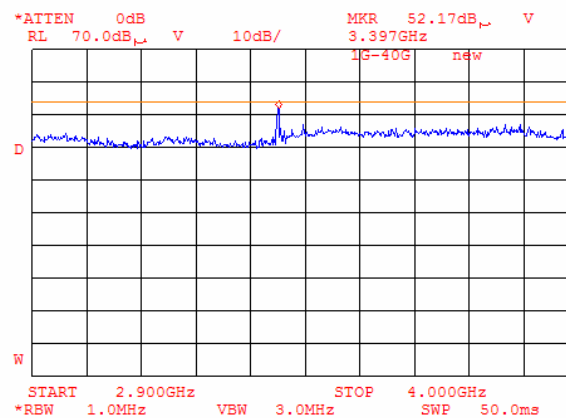
Plot 8.8.83 Radiated emission measurements at 3395 MHz at the high carrier frequency (BT and G20-850)
