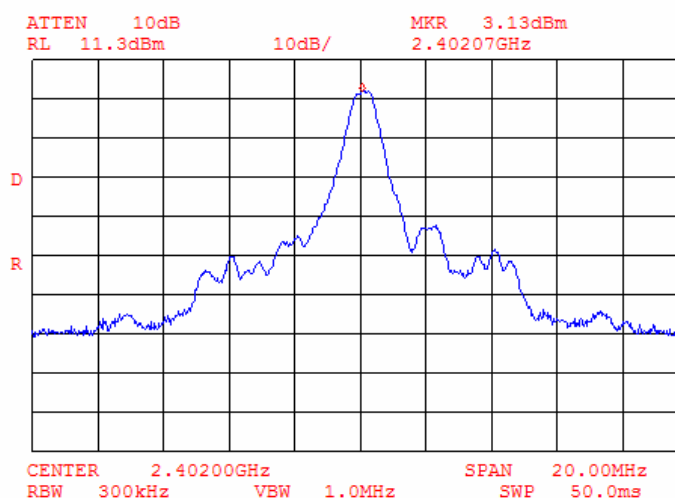
Plot 8.7.1 The highest emission level within the assigned band at low carrier frequency
