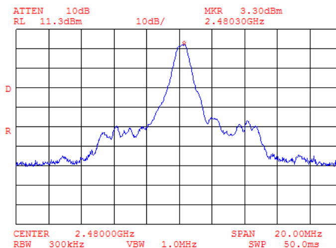
Plot 8.7.2 The highest emission level within the assigned band at high carrier frequency
