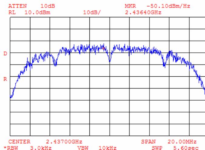
Plot 9.4.11 Peak spectral power density at mid frequency within 6 dB band, bit rate 2 Mbps
