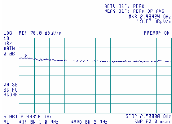
Plot 9.3.26 Radiated emission measurements at band edge at the high carrier frequency, bit rate 1 Mbps
