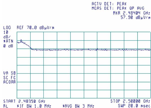
Plot 8.8.75 Radiated emission measurements from 2483.5 to 2500 MHz at the high carrier frequency (BT and G20-1900)
