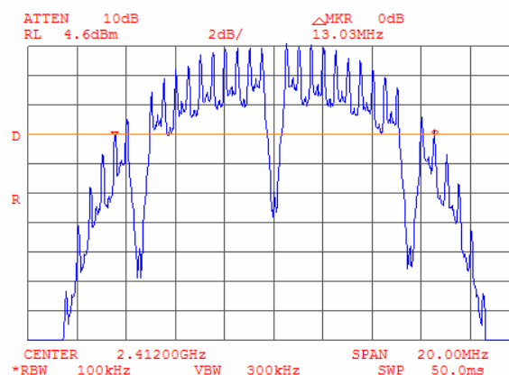
Plot 9.1.2 The 6 dB bandwidth test result at low frequency, Bit Rate 2 Mbps
