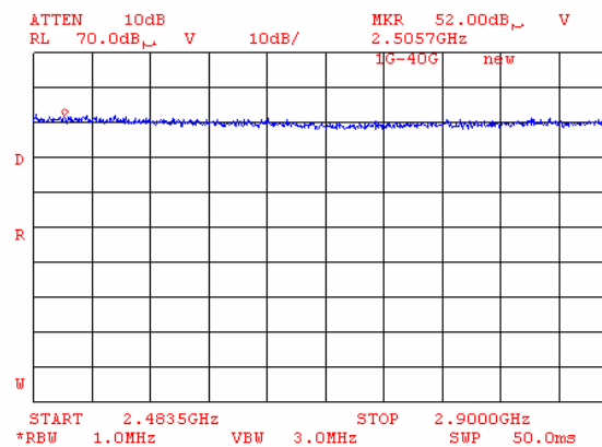
Plot 8.8.71 Radiated emission measurements from 2483.5 to 2900 MHz at the mid carrier frequency (BT and G20-1900)
