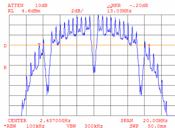
Plot 9.1.6 The 6 dB bandwidth test result at mid frequency, Bit Rate 2 Mbps
