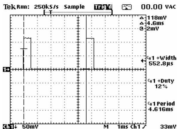
Plot 7.1.1 Duty cycle test results, G20 850
