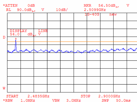
Plot 8.8.69 Radiated emission measurements at 2509 MHz at the mid carrier frequency (BT and G20-850)
