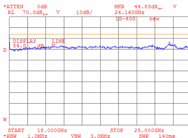
Plot 9.3.58 Radiated emission measurements from 18000 to 25000 MHz at the high carrier frequency (WLAN + BT)
