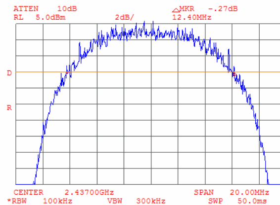
Plot 9.1.8 The 6 dB bandwidth test result at mid frequency, Bit Rate 11 Mbps
