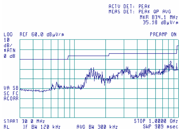
Plot 9.3.12 Radiated emission measurements from 30 to 1000 MHz at the high carrier frequency
