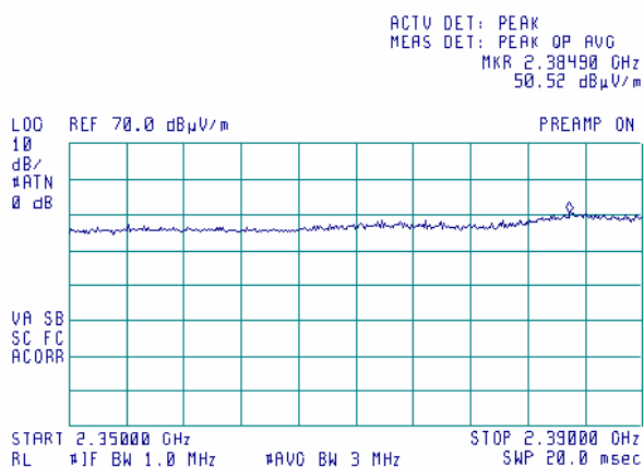
Plot 9.3.24 Radiated emission measurements at band edge at the low carrier frequency, bit rate 11 Mbps
