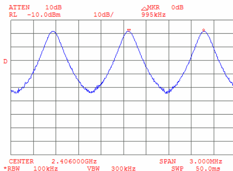
Plot 8.3.1 Carrier frequency separation
