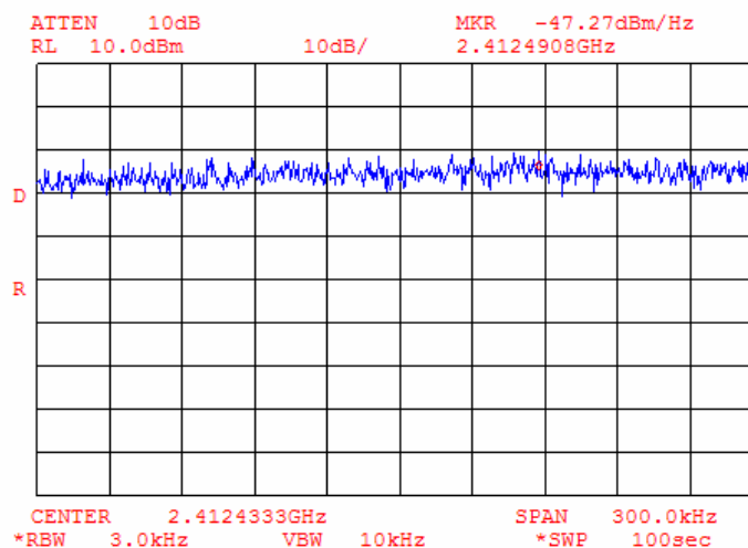
Plot 9.4.8 Peak spectral power density at low frequency zoomed at the peak, bit rate 11 Mbps
