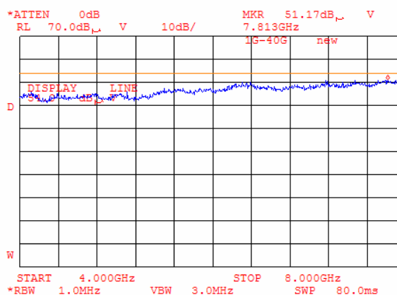
Plot 8.8.103 Radiated emission measurements at 4244 MHz at the high carrier frequency (BT and G20-850)
