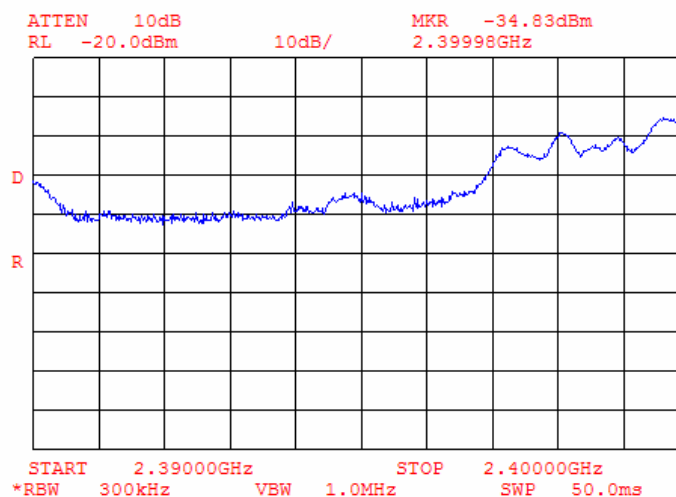
Plot 8.7.3 The highest band edge emission at low carrier frequency with hopping function disabled
