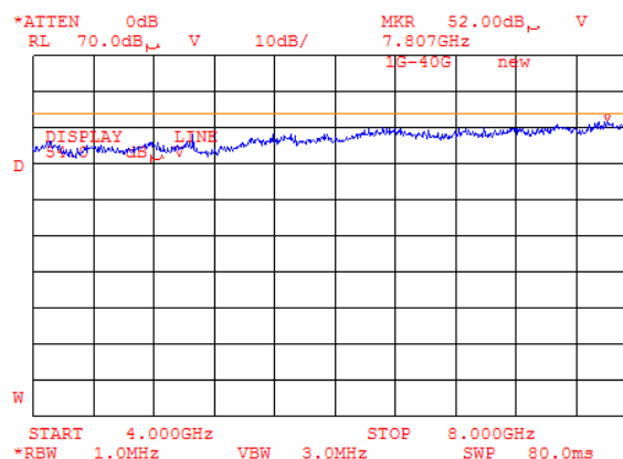
Plot 8.8.91 Radiated emission measurements at 4121 MHz at the low carrier frequency (BT and G20-850)
