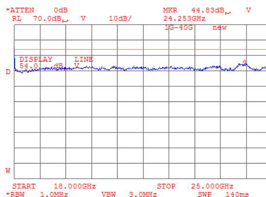
Plot 8.8.144 Radiated emission measurements from 18000 to 25000 MHz at the low carrier frequency (BT and G20-1900)
