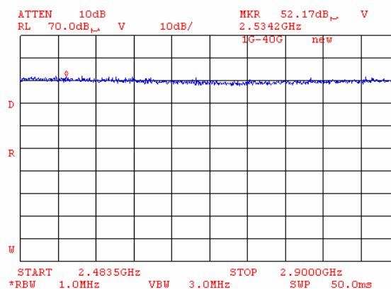
Plot 8.8.67 Radiated emission measurements from 2483.5 to 2900 MHz at the low carrier frequency (BT and G20-1900)
