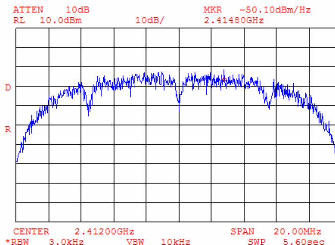
Plot 9.4.1 Peak spectral power density at low frequency within 6 dB band, bit rate 1 Mbps
