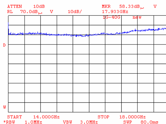
Plot 8.8.140 Radiated emission measurements from 14000 to 18000 MHz at the high carrier frequency (BT and G20-1900)
