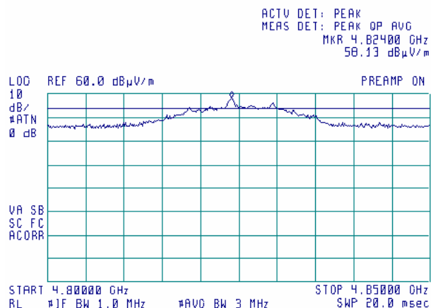
Plot 9.3.42 Radiated emission measurements from 4800 to 4850 MHz at the low carrier frequency (WLAN second harmonic)
