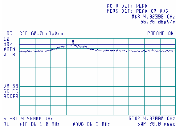
Plot 9.3.46 Radiated emission measurements from 4900 to 4970 MHz at the high carrier frequency (WLAN and BT second harmonic)
