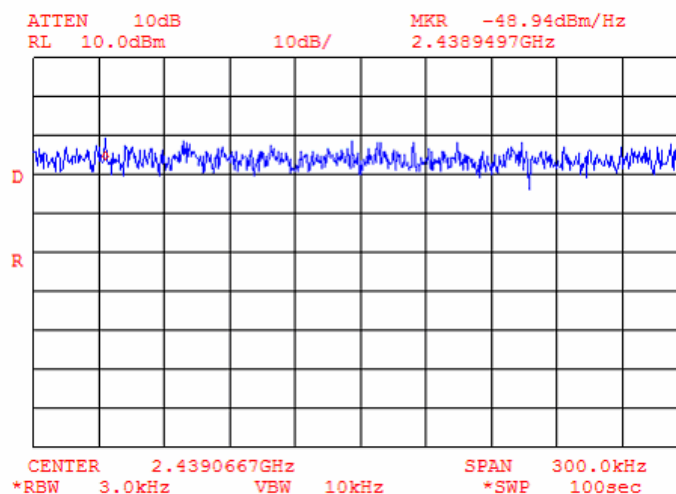
Plot 9.4.16 Peak spectral power density at mid frequency zoomed at the peak, bit rate 11 Mbps
