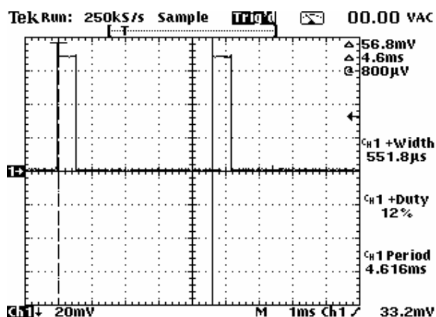
Plot 7.1.2 Duty cycle test results, G20 1900
