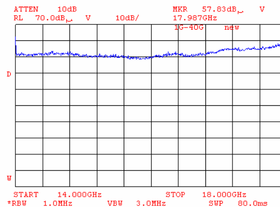
Plot 8.8.130 Radiated emission measurements from 14000 to 18000 MHz at the low carrier frequency (BT and G20-850)
