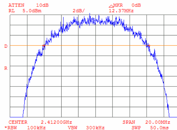
Plot 9.1.4 The 6 dB bandwidth test result at low frequency, Bit Rate 11 Mbps
