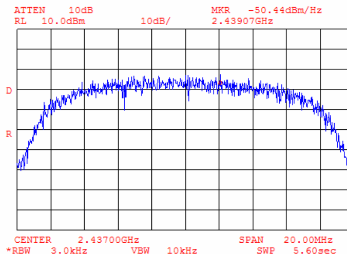
Plot 9.4.15 Peak spectral power density at mid frequency within 6 dB band, bit rate 11 Mbps
