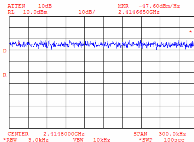
Plot 9.4.2 Peak spectral power density at low frequency zoomed at the peak, bit rate 1 Mbps
