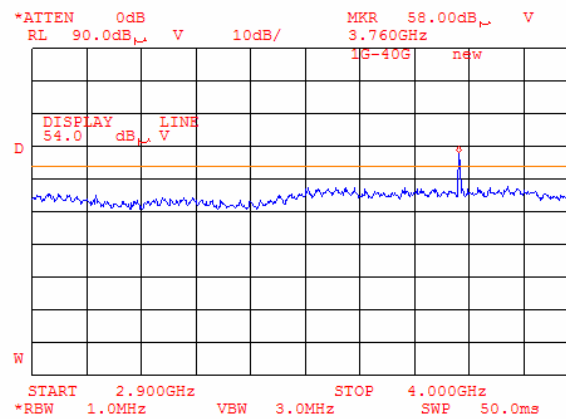
Plot 8.8.87 Radiated emission measurements at 3760 MHz at the mid carrier frequency (BT and G20-1900)
