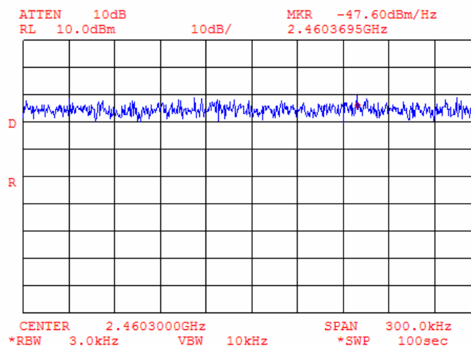
Plot 9.4.20 Peak spectral power density at high frequency zoomed at the peak, bit rate 2 Mbps
