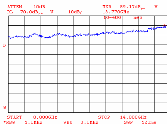
Plot 8.8.118 Radiated emission measurements from 8000 to 14000 MHz at the low carrier frequency (BT and G20-850)
