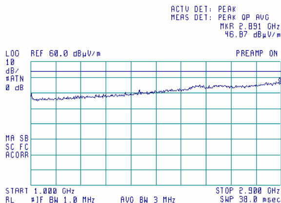
Plot 10.1.4 Radiated emission measurements above 1000 MHz, horizontal antenna polarization
