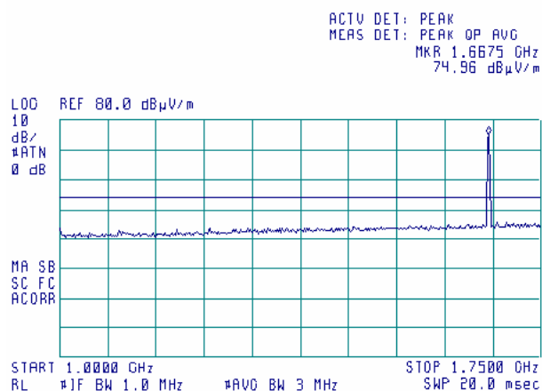
Plot 8.8.46 Radiated emission measurements at 1673 MHz at the mid carrier frequency (BT and G20-850)
