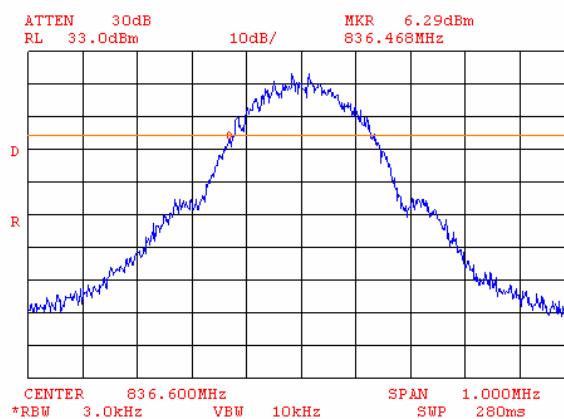
Plot 7.3.5 Occupied bandwidth test result at mid frequency, lower reference point
