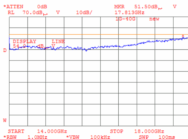
Plot 9.3.54 Radiated emission measurements from 14000 to 18000 MHz at the mid carrier frequency (WLAN + BT)
