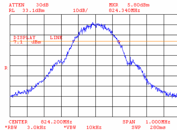
Plot 7.3.3 Occupied bandwidth test result at low frequency, higher reference point
