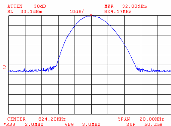
Plot 7.3.1 Occupied bandwidth test result at low frequency, reference level
