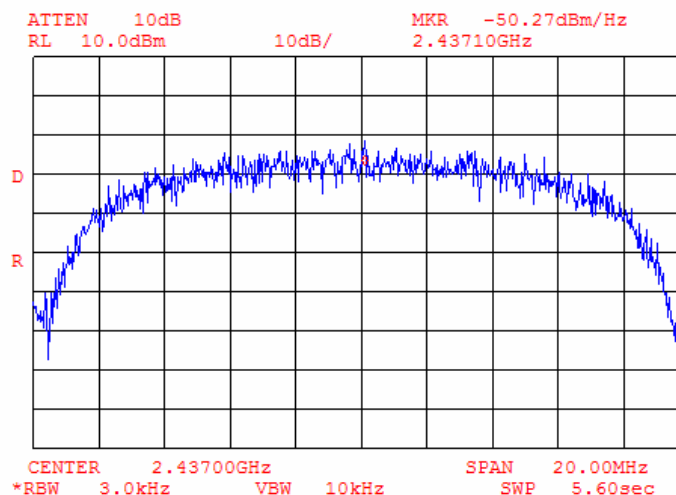
Plot 9.4.13 Peak spectral power density at mid frequency within 6 dB band, bit rate 5.5 Mbps
