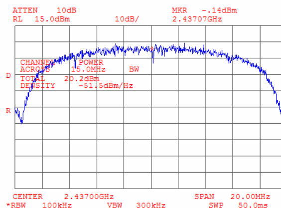
Plot 9.2.8 Peak output power at mid frequency, Bit Rate 11 Mbps
