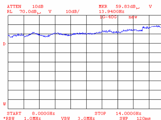
Plot 8.8.128 Radiated emission measurements from 8000 to 14000 MHz at the high carrier frequency (BT and G20-1900)
