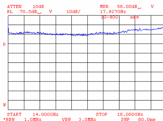
Plot 8.8.136 Radiated emission measurements from 14000 to 18000 MHz at the low carrier frequency (BT and G20-1900)
