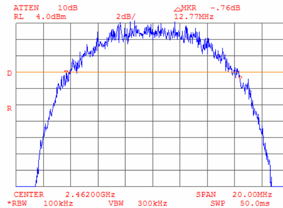
Plot 9.1.12 The 6 dB bandwidth test result at high frequency, Bit Rate 11 Mbps
