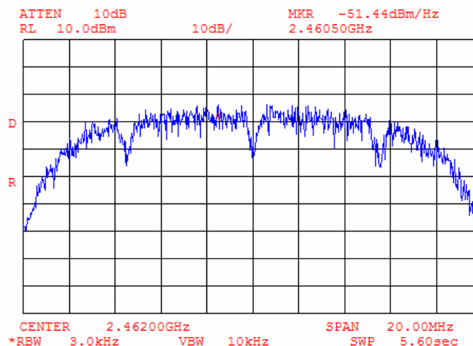
Plot 9.4.17 Peak spectral power density at high frequency within 6 dB band, bit rate 1 Mbps
