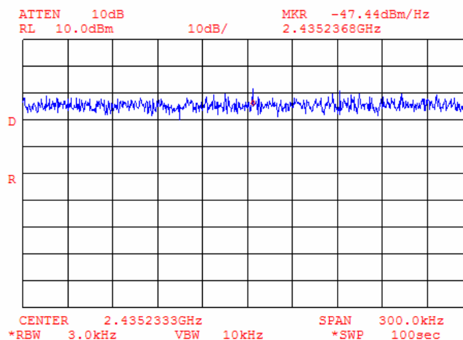
Plot 9.4.10 Peak spectral power density at mid frequency zoomed at the peak, bit rate 1 Mbps
