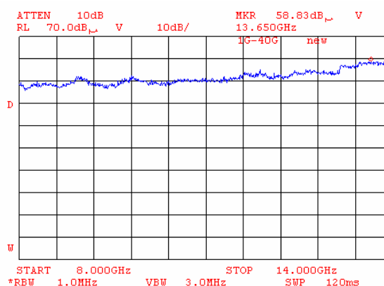
Plot 8.8.124 Radiated emission measurements from 8000 to 14000 MHz at the low carrier frequency (BT and G20-1900)
