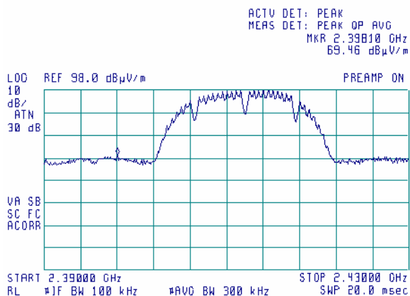
Plot 9.3.20 Radiated emission measurements at band edge at the low carrier frequency, bit rate 1 Mbps
