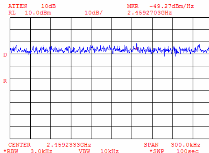
Plot 9.4.22 Peak spectral power density at high frequency zoomed at the peak, bit rate 5.5 Mbps
