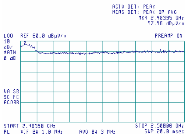
Plot 9.3.28 Radiated emission measurements at band edge at the high carrier frequency, bit rate 11 Mbps
