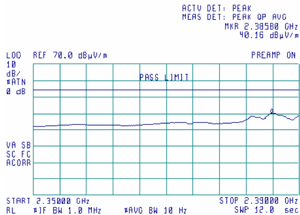
Plot 9.3.22 Radiated emission measurements at band edge at the low carrier frequency, bit rate 11 Mbps
