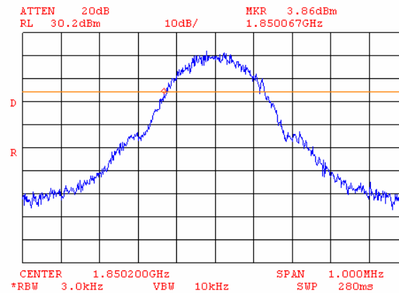
Plot 7.3.11 Occupied bandwidth test result at low frequency, lower reference point
