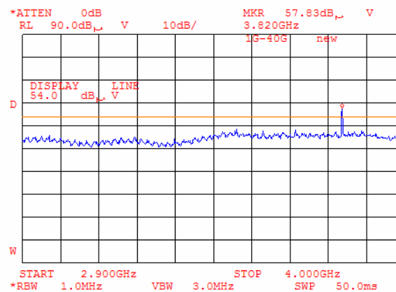
Plot 8.8.89 Radiated emission measurements at 3819 MHz at the high carrier frequency (BT and G20-1900)
