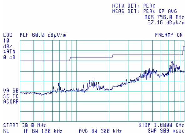
Plot 10.1.2 Radiated emission measurements in 30 - 1000 MHz range, horizontal antenna polarization
