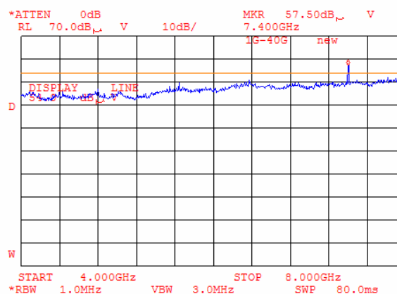
Plot 8.8.109 Radiated emission measurements at 5550 MHz at the low carrier frequency (BT and G20-1900)
