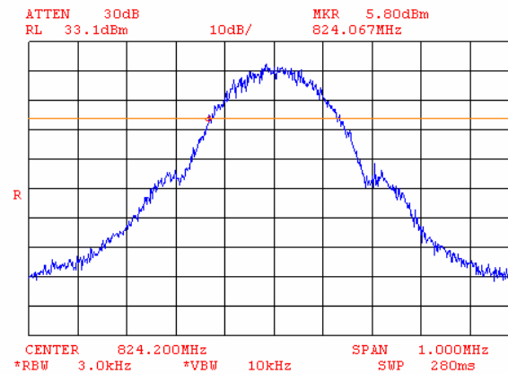
Plot 7.3.2 Occupied bandwidth test result at low frequency, lower reference point
