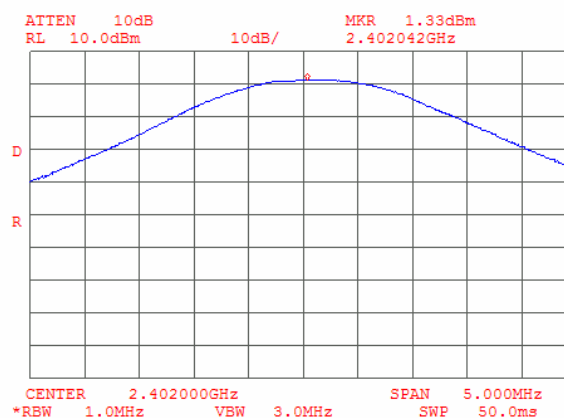
Plot 8.6.1 Peak output power at low frequency
