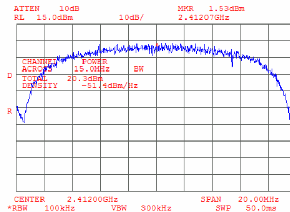
Plot 9.2.4 Peak output power at low frequency, Bit Rate 11 Mbps
