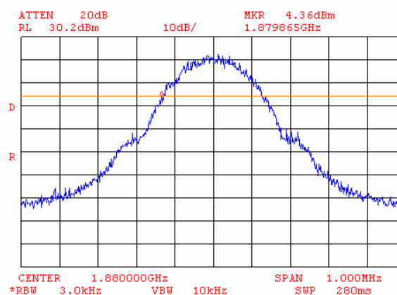
Plot 7.3.14 Occupied bandwidth test result at mid frequency, lower reference point
