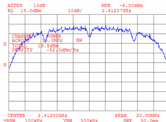
Plot 9.2.2 Peak output power at low frequency, Bit Rate 2 Mbps
