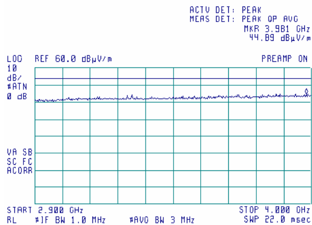
Plot 9.3.36 Radiated emission measurements from 2900 to 4000 MHz at the mid carrier frequency
