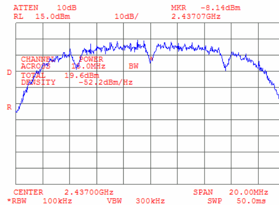
Plot 9.2.6 Peak output power at mid frequency, Bit Rate 2 Mbps
