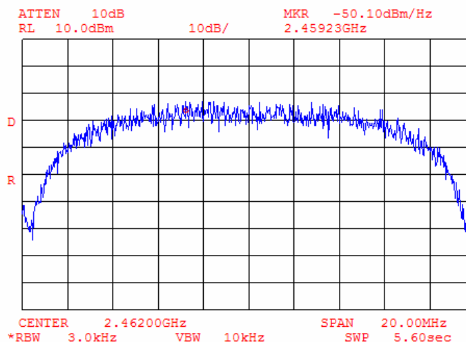
Plot 9.4.21 Peak spectral power density at high frequency within 6 dB band, bit rate 5.5 Mbps
