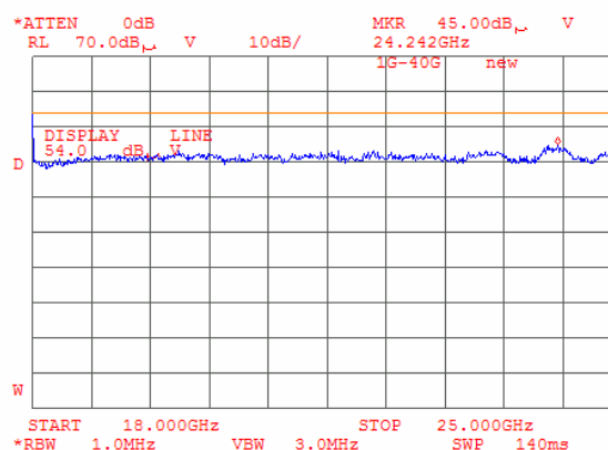
Plot 8.8.146 Radiated emission measurements from 18000 to 25000 MHz at the high carrier frequency (BT and G20-1900)
