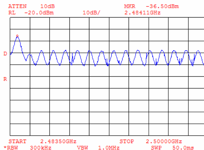
Plot 8.7.5 The higher band edge emissions with hopping function enabled
