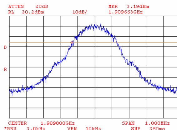
Plot 7.3.18 Occupied bandwidth test result at high frequency, higher reference point
