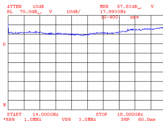
Plot 8.8.132 Radiated emission measurements from 14000 to 18000 MHz at the mid carrier frequency (BT and G20-850)
