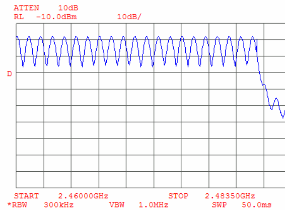
Plot 8.4.3 Number of hopping frequencies at 2460 – 2483.5 MHz range
