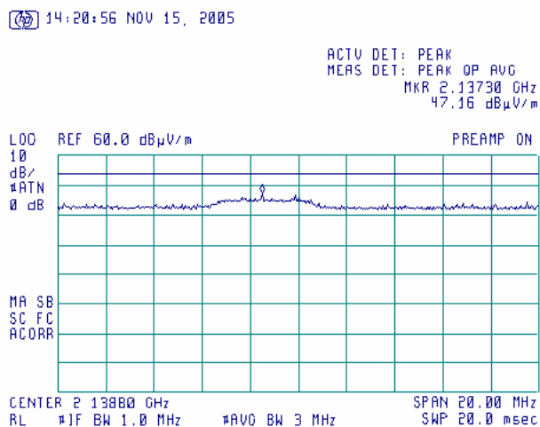
Plot 8.8.32 Radiated emission measurements at 2137 MHz at the low carrier frequency (BT and G20-850)
