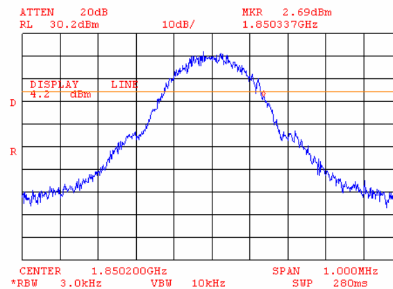
Plot 7.3.12 Occupied bandwidth test result at low frequency, higher reference point
