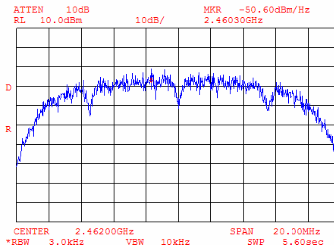
Plot 9.4.19 Peak spectral power density at high frequency within 6 dB band, bit rate 2 Mbps
