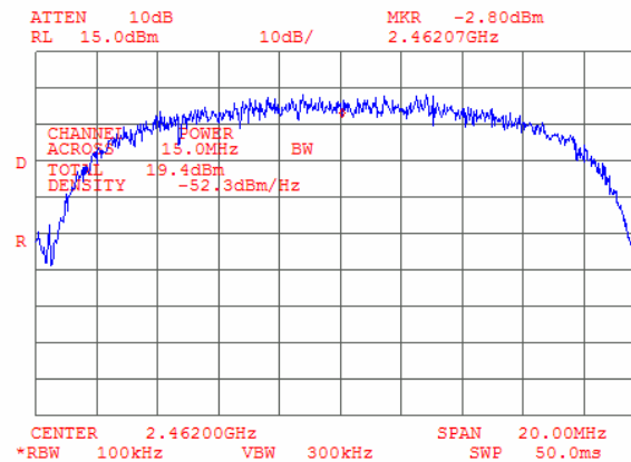
Plot 9.2.12 Peak output power at high frequency, Bit Rate 11 Mbps
