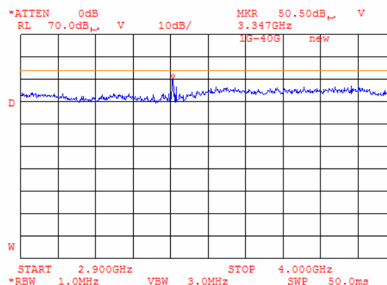
Plot 8.8.81 Radiated emission measurements at 3346 MHz at the mid carrier frequency (BT and G20-850)
