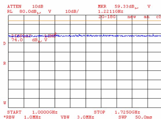
Plot 8.8.60 Radiated emission measurements from 1000 to 1725 MHz at the high carrier frequency (BT and G20-1900)
