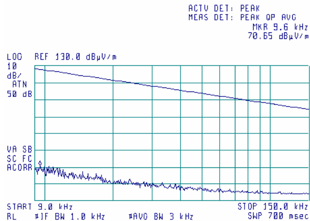
Plot 8.8.12 Radiated emission measurements from 9 to 150 kHz at the high carrier frequency (BT+G20-1900)
