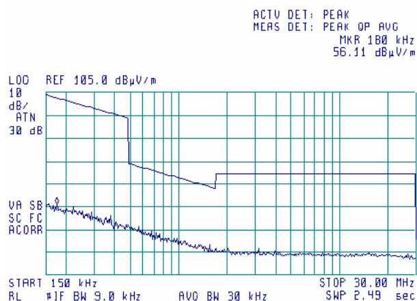
Plot 8.8.8 Radiated emission measurements from 0.15 to 30 MHz at the mid carrier frequency (BT+G20-850)
