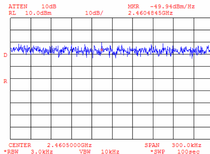
Plot 9.4.18 Peak spectral power density at high frequency zoomed at the peak, bit rate 1 Mbps
