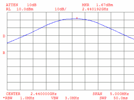
Plot 8.6.2 Peak output power at mid frequency
