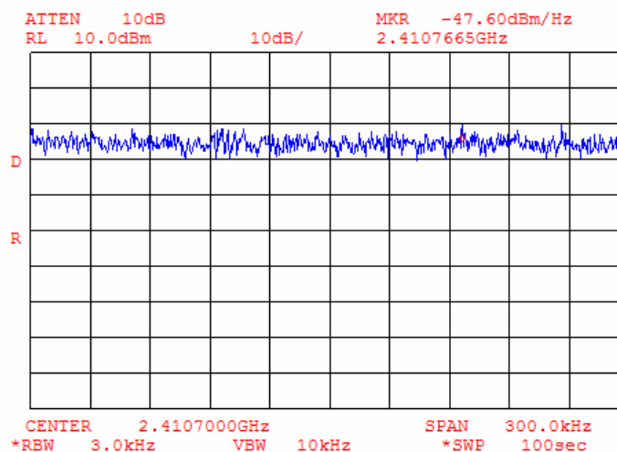
Plot 9.4.6 Peak spectral power density at low frequency zoomed at the peak, bit rate 5.5 Mbps
