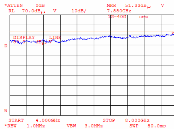
Plot 8.8.97 Radiated emission measurements at 4182 MHz at the mid carrier frequency (BT and G20-850)
