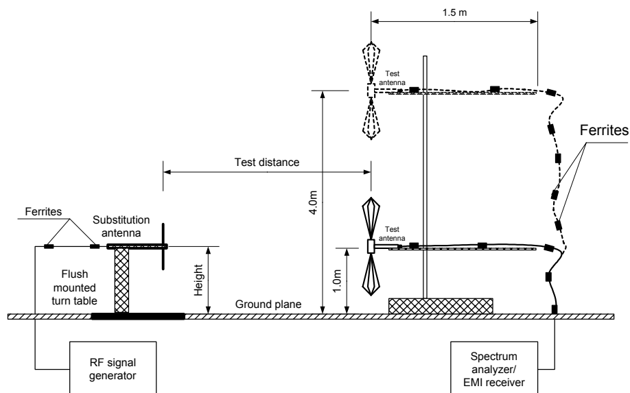
Figure 7.2.2 Setup for substitution peak output power measurements
