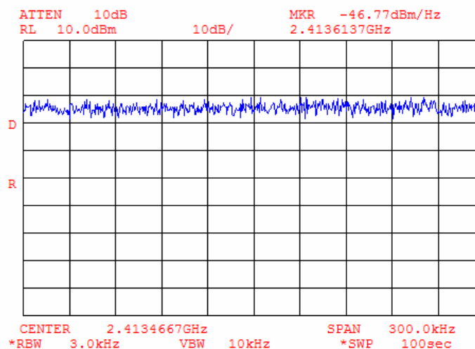
Plot 9.4.4 Peak spectral power density at low frequency zoomed at the peak, bit rate 2 Mbps
