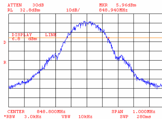
Plot 7.3.9 Occupied bandwidth test result at high frequency, higher reference point
