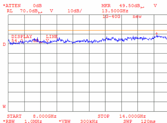
Plot 9.3.52 Radiated emission measurements from 8000 to 14000 MHz at the high carrier frequency (WLAN + BT)
