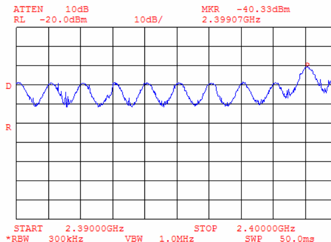
Plot 8.7.6 The lower band edge emission with hopping function enabled
