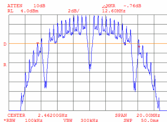
Plot 9.1.10 The 6 dB bandwidth test result at high frequency, Bit Rate 2 Mbps
