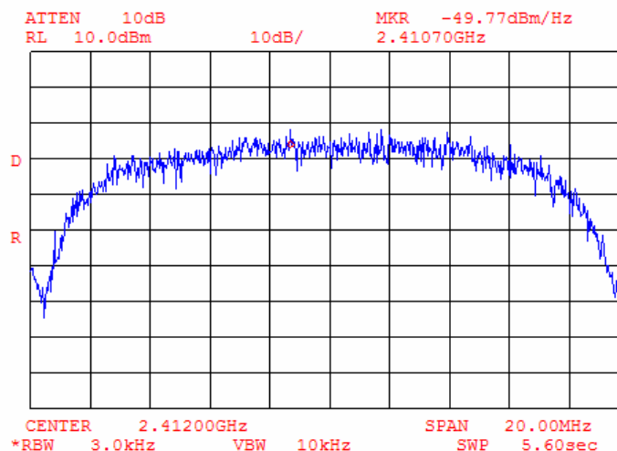
Plot 9.4.5 Peak spectral power density at low frequency within 6 dB band, bit rate 5.5 Mbps
