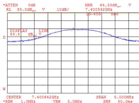
Plot 8.8.111 Radiated emission measurements from 4000 to 8000 MHz at the mid carrier frequency (BT and G20-1900)
