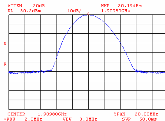
Plot 7.3.16 Occupied bandwidth test result at high frequency, reference level
