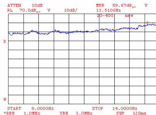
Plot 8.8.126 Radiated emission measurements from 8000 to 14000 MHz at the mid carrier frequency (BT and G20-1900)
