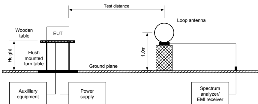
Figure 8.8.1 Setup for spurious emission field strength measurements below 30 MHz
