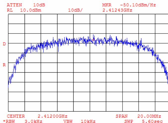
Plot 9.4.7 Peak spectral power density at low frequency within 6 dB band, bit rate 11 Mbps
