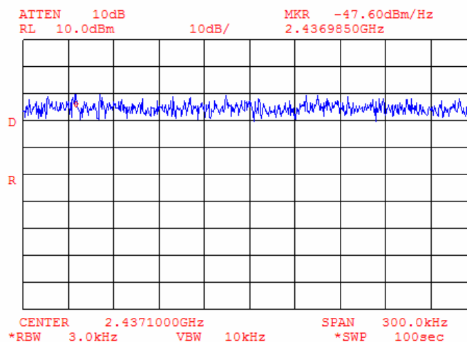
Plot 9.4.14 Peak spectral power density at mid frequency zoomed at the peak, bit rate 5.5 Mbps
