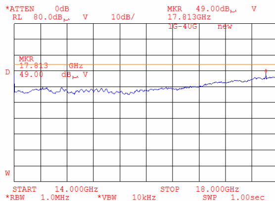
Plot 8.1.115 Radiated emission measurements from 14000 to 18000 MHz at the low carrier frequency (BT and G20-1900)
