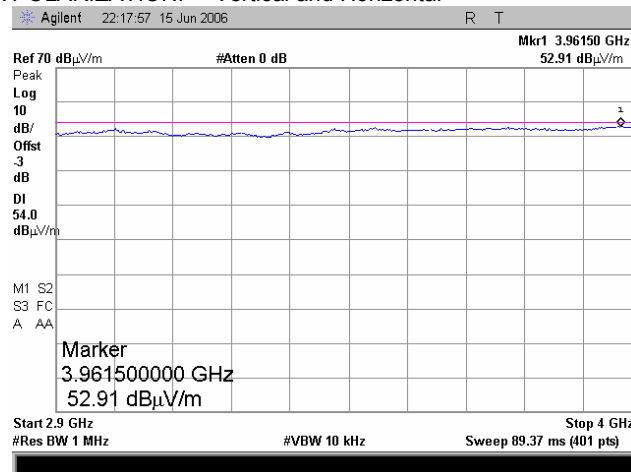
Plot 8.1.66 Radiated emission measurements at 3346 MHz at the mid carrier frequency (BT and G20-850)
