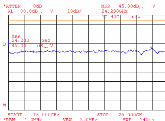
Plot 8.1.123 Radiated emission measurements from 18000 to 25000 MHz at the high carrier frequency (BT and G20-850)
