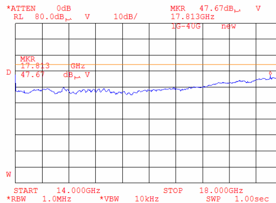
Plot 8.1.113 Radiated emission measurements from 14000 to 18000 MHz at the high carrier frequency (BT and G20-850)
