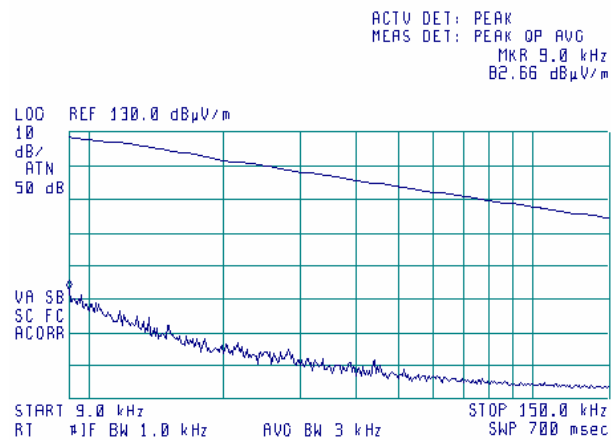
Plot 8.1.12 Radiated emission measurements from 9 to 150 kHz at the high carrier frequency (BT+G20-1900)
