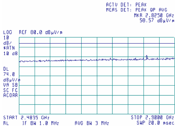
Plot 8.1.52 Radiated emission measurements from 2483.5 to 2900 MHz at the low carrier frequency (BT and G20-1900)
