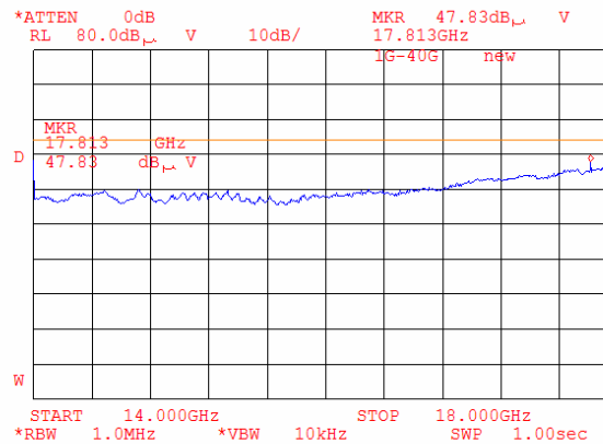
Plot 8.1.111 Radiated emission measurements from 14000 to 18000 MHz at the mid carrier frequency (BT and G20-850)
