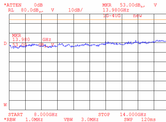
Plot 8.1.105 Radiated emission measurements from 8000 to 14000 MHz at the high carrier frequency (BT and G20-850)
