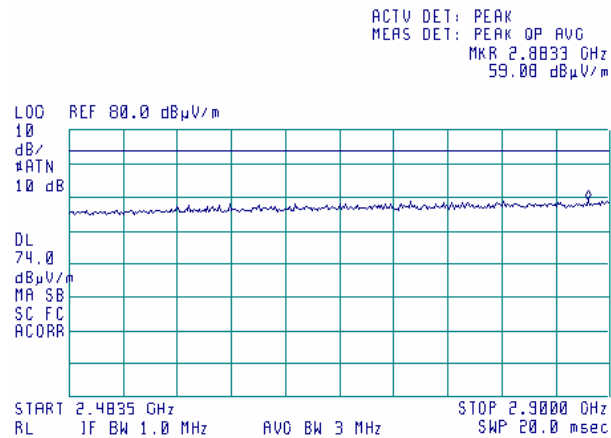
Plot 8.1.56 Radiated emission measurements from 2483.5 to 2900 MHz at the mid carrier frequency (BT and G20-1900)
