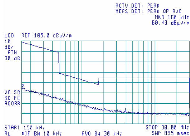
Plot 8.1.8 Radiated emission measurements from 0.15 to 30 MHz at the mid carrier frequency (BT+G20-850)
