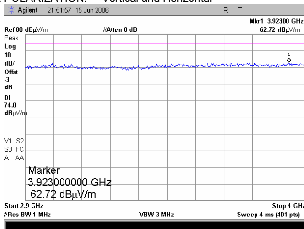
Plot 8.1.74 Radiated emission measurements from 2900 to 4000 MHz at the mid carrier frequency (BT and G20-1900)
