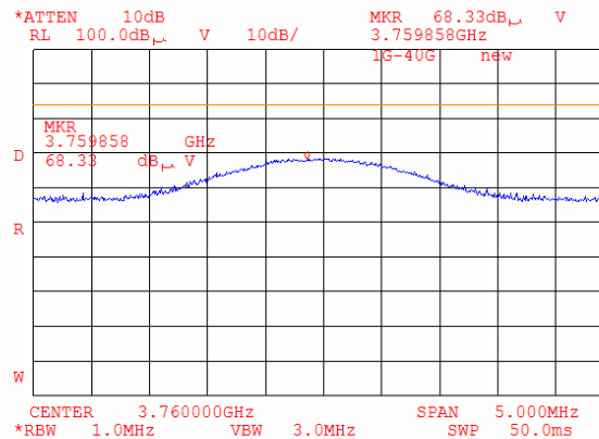
Plot 8.1.76 Radiated emission measurements from 2900 to 4000 MHz at the high carrier frequency (BT and G20-1900)
