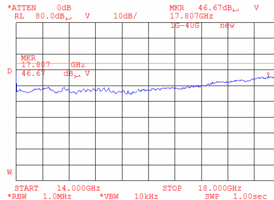
Plot 8.1.117 Radiated emission measurements from 14000 to 18000 MHz at the mid carrier frequency (BT and G20-1900)
