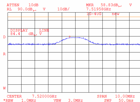
Plot 8.1.97 Radiated emission measurements from 4000 to 8000 MHz at the high carrier frequency (G20-1900 and BT)
