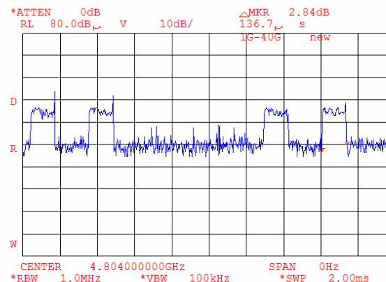
Plot 8.1.128 Second pulse duration measurements
