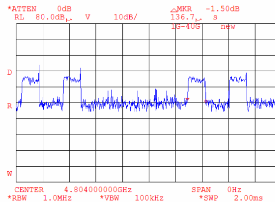
Plot 8.1.127 First pulse duration measurements
