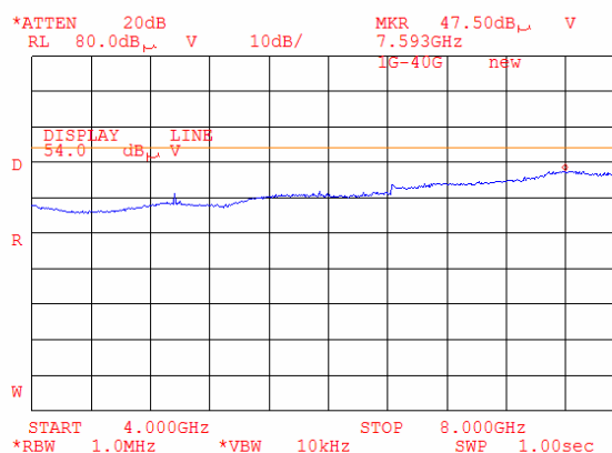
Plot 8.1.85 Radiated emission measurements from 4000 to 8000 MHz at the low carrier frequency (G20-1900 and BT)
