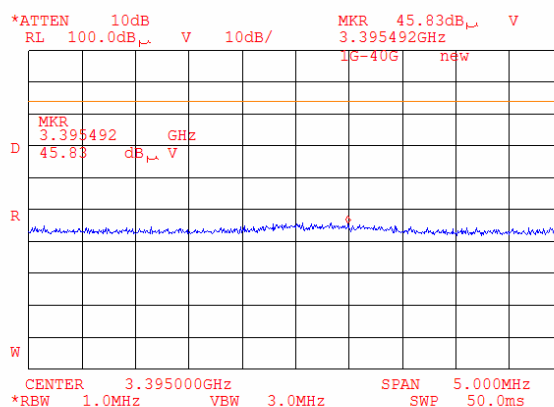
Plot 8.1.70 Radiated emission measurements from 2900 to 4000 MHz at the low carrier frequency (BT and G20-1900)
