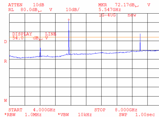
Plot 8.1.87 Radiated emission measurements at 4804 MHz at the low carrier frequency (G20-1900 and BT)
