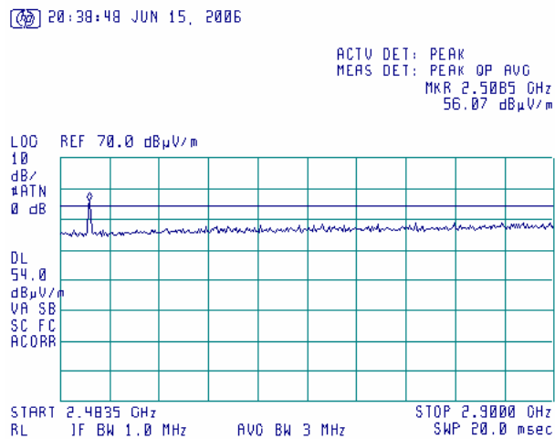
Plot 8.1.54 Radiated emission measurements at 2509 MHz at the mid carrier frequency (BT and G20-850)
