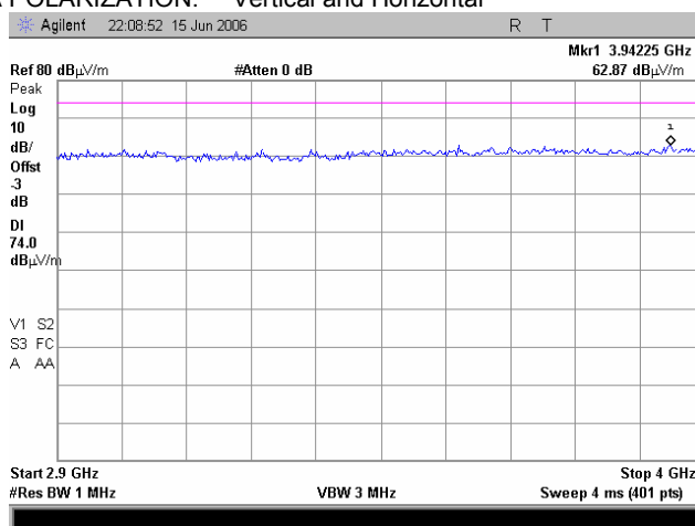
Plot 8.1.68 Radiated emission measurements from 2900 to 4000 MHz at the high carrier frequency (BT and G20-850)
