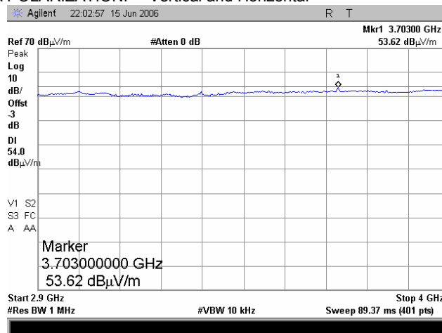
Plot 8.1.72 Radiated emission measurements at 3700 MHz at the low carrier frequency (BT and G20-1900)
