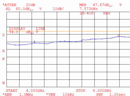
Plot 8.1.83 Radiated emission measurements from 4000 to 8000 MHz at the high carrier frequency (G20-850 and BT)
