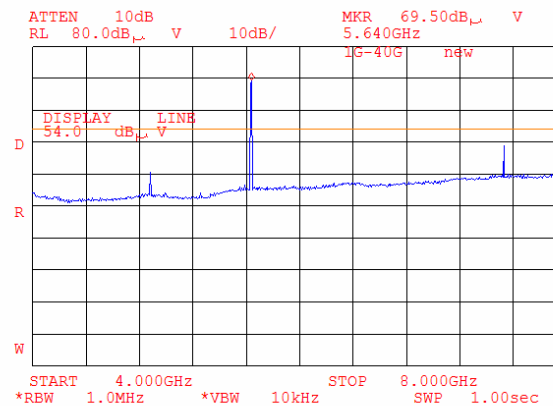
Plot 8.1.93 Radiated emission measurements at 4880 MHz at the mid carrier frequency (G20-1900 and BT)
