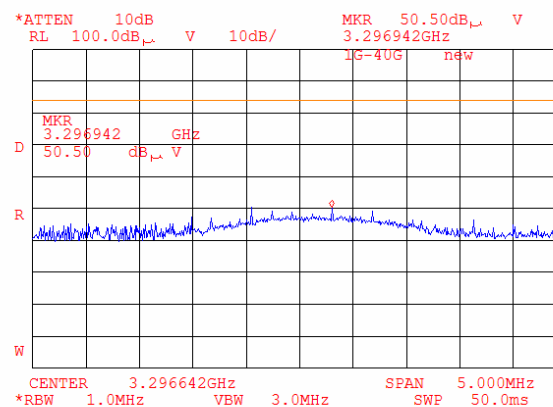
Plot 8.1.64 Radiated emission measurements from 2900 to 4000 MHz at the mid carrier frequency (BT and G20-850)
