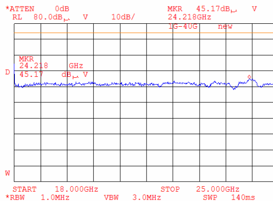
Plot 8.1.125 Radiated emission measurements from 18000 to 25000 MHz at the mid carrier frequency (BT and G20-1900)
