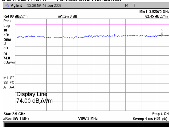
Plot 8.1.62 Radiated emission measurements from 2900 to 4000 MHz at the low carrier frequency (BT and G20-850)
