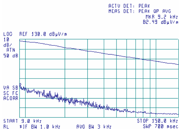
Plot 8.1.6 Radiated emission measurements from 9 to 150 kHz at the high carrier frequency (BT+G20-850)
