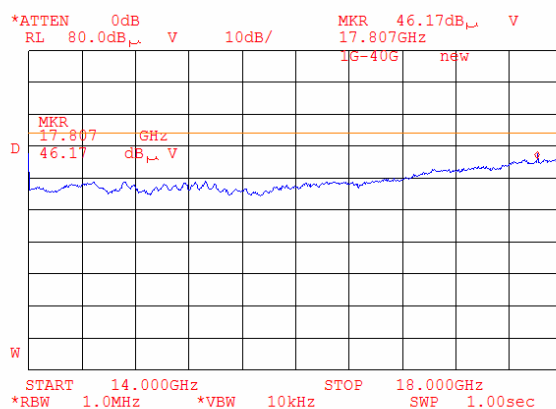
Plot 8.1.119 Radiated emission measurements from 14000 to 18000 MHz at the high carrier frequency (BT and G20-1900)
