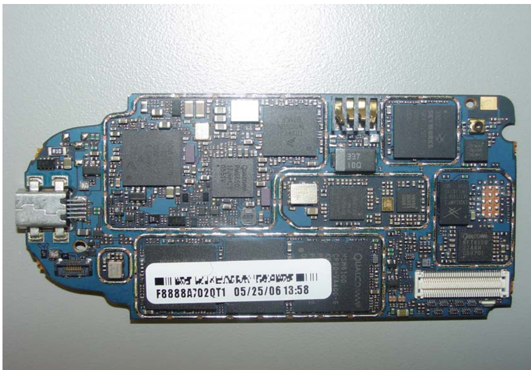
Photograph 9-3: Back side view of radio PC Board, without shields.
