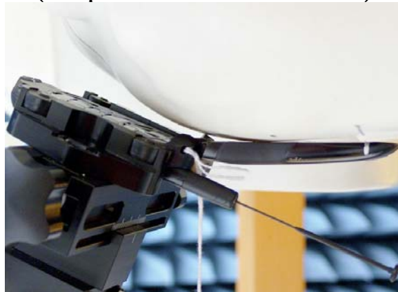
Figure 9: Assessment at the Head DUT at the left ear in tilt position. (same position used for antenna retracted)
