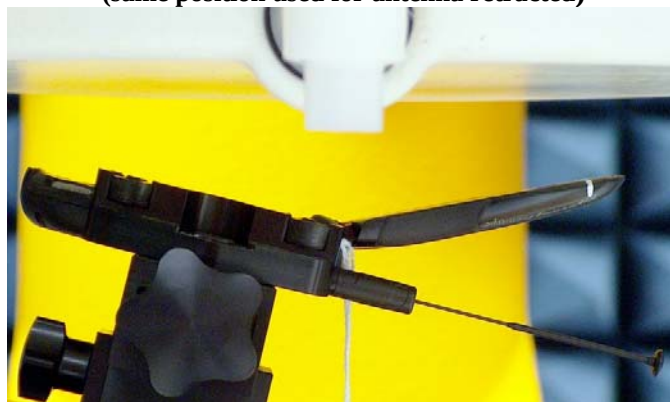
Figure 6: Face Assessment DUT Flip opened w/ front side separated 2.5cm from the phantom. (same position used for antenna retracted)
