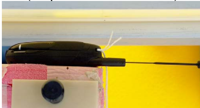
Figure 5: Body Assessment DUT w/ front side separated 2.5cm from the phantom. (same position used for antenna retracted)
