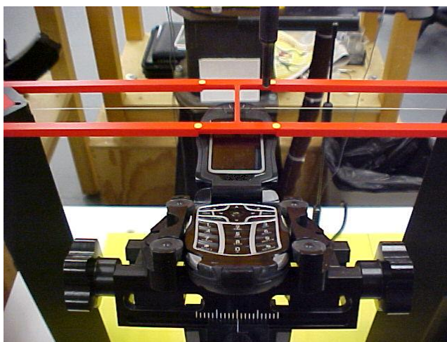
Figure A6-2. Views from the front
