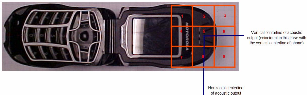
Figure A6-1. Phone Open - Orientation of Wireless Device and Measurement Plane
