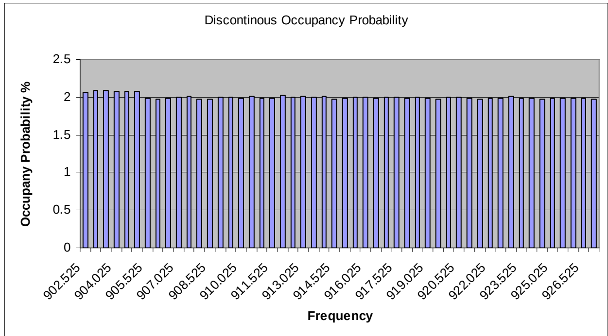
Figure 6c-7. Histogram for 900 MHz ISM Band Discontinuous Transmission
