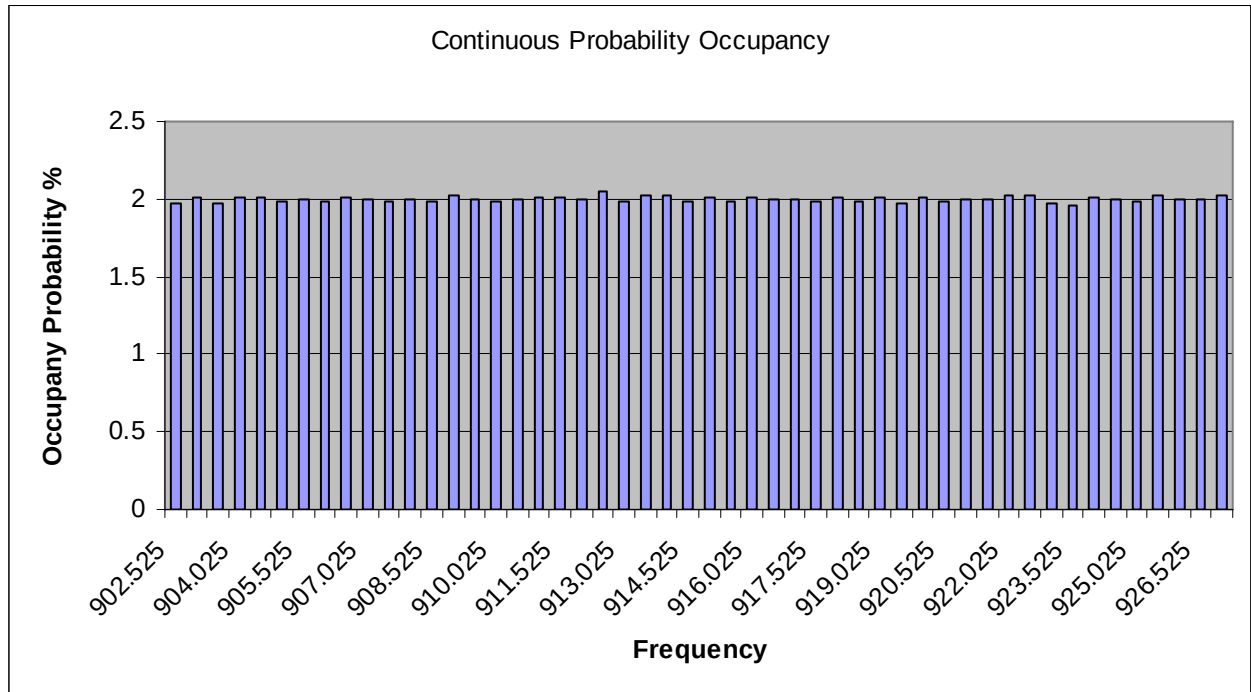
Figure 6c-6. Histogram for 900 MHz ISM Band Continuous Transmission
