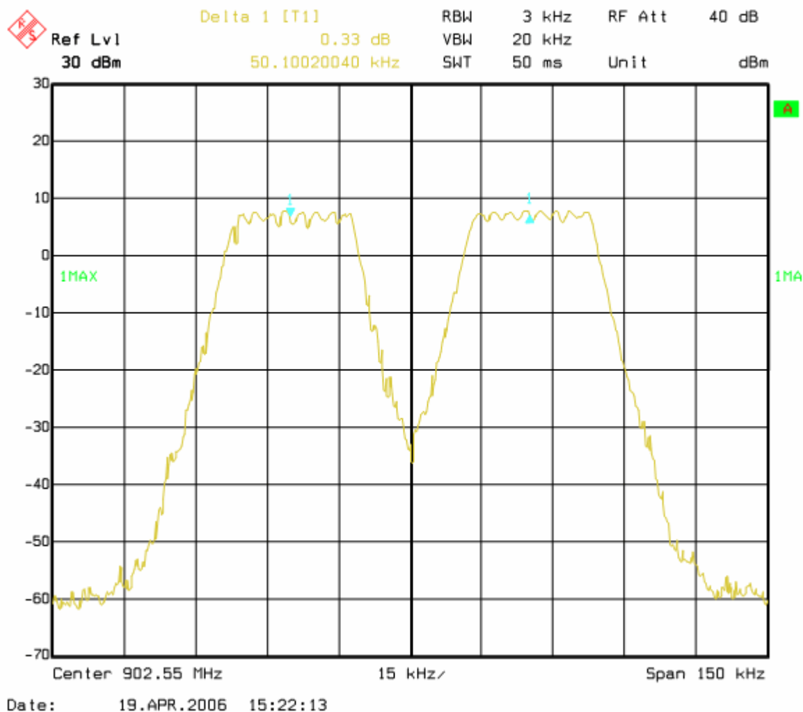
Figure 6c-3. Adjacent hopset separation.
