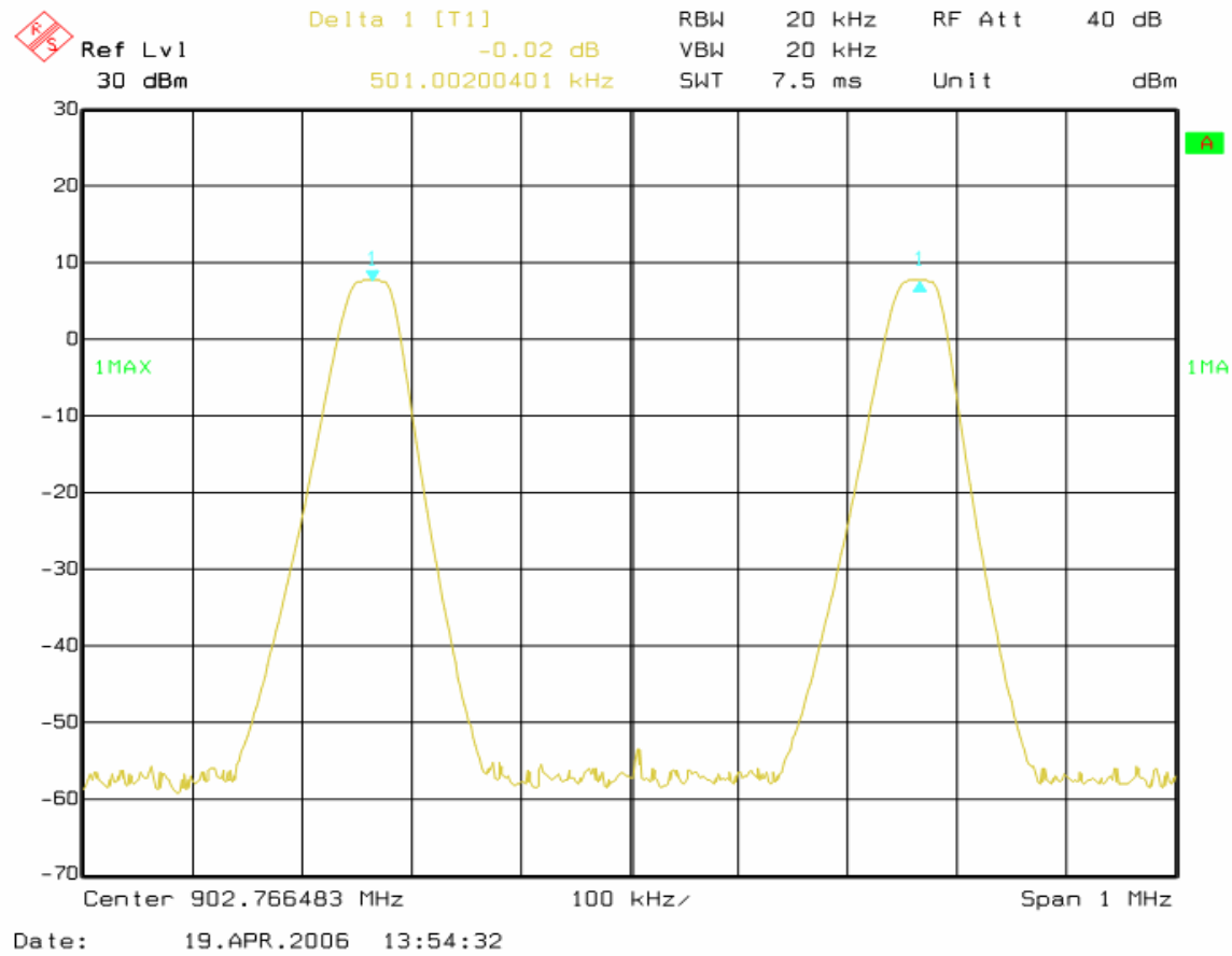
Figure 6b-2.1 Plot of MOTotalk ISM Band adjacent channel separation within a hopset
