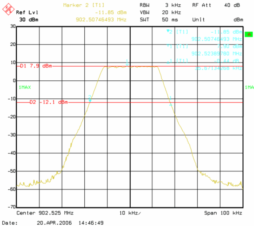
Figure 6b-2.2.1 MOTOTalk 8-FSK traffic channel Occupied bandwidth at 902.525 MHz
