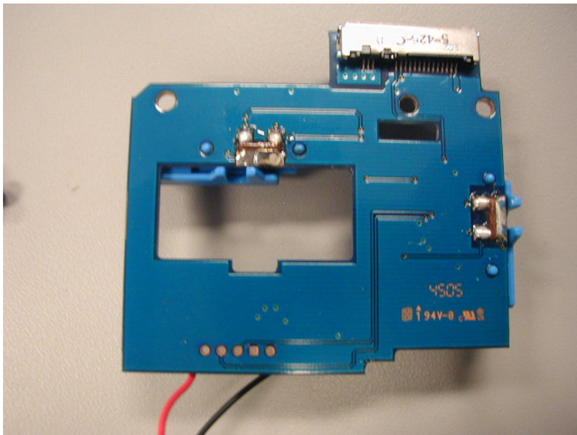
Photograph 9-4: Bottom view of Handheld Controller PC Board.
