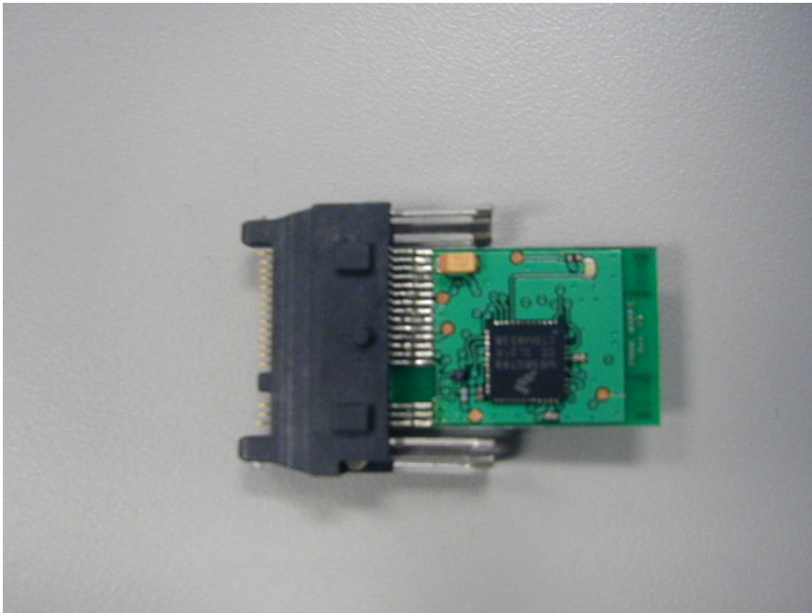
Photograph 9-1: Front side view of Dongle PC Board
