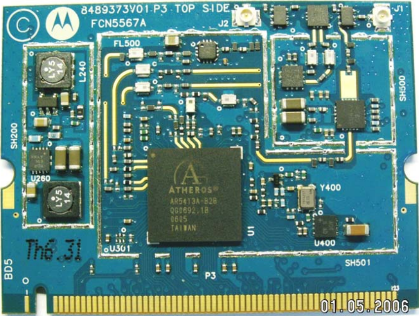
Photograph 9.2: Top view of WDE1000.
