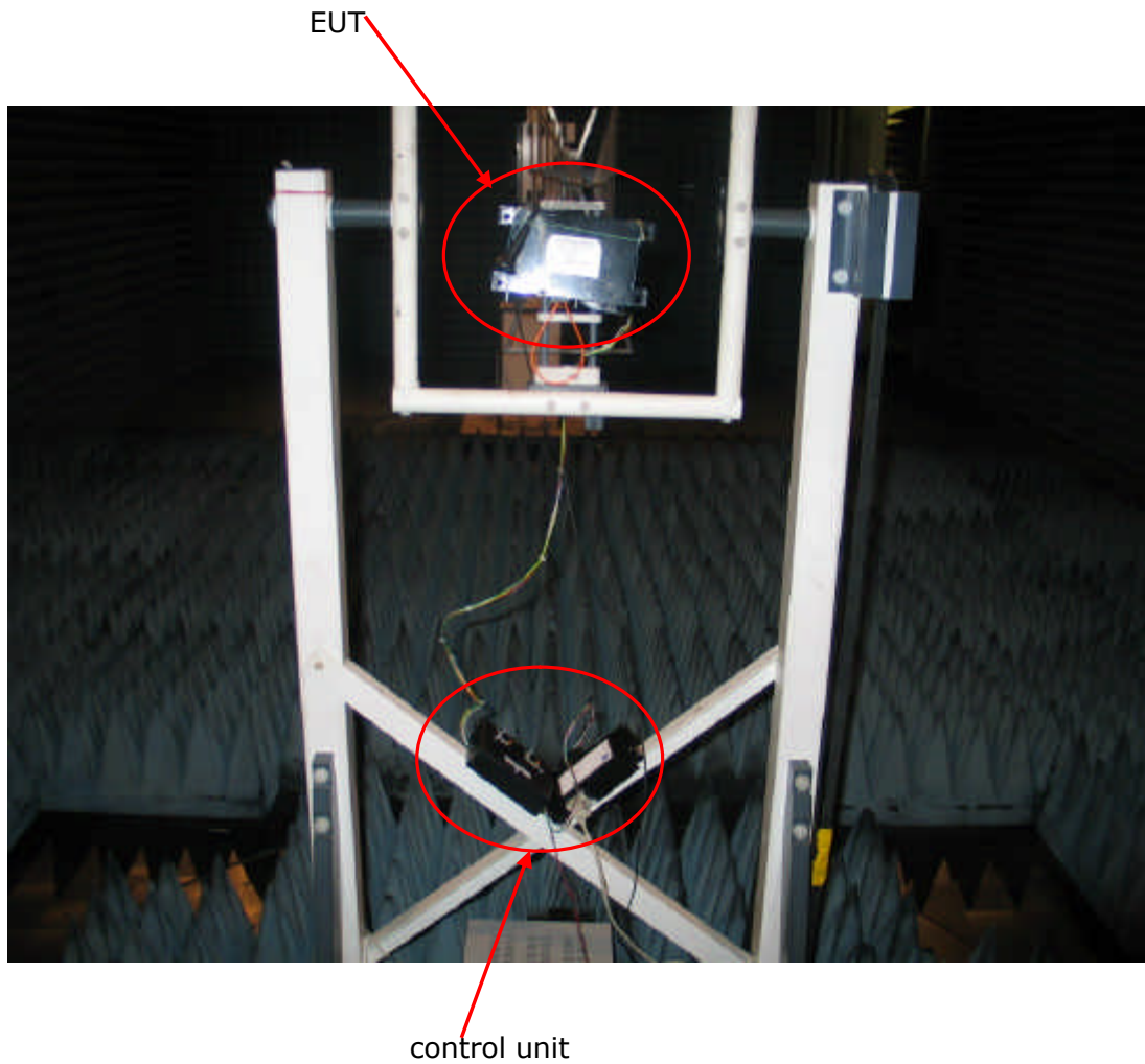
Photo 1: Test setup for radiated measurements. EUT with control unit
