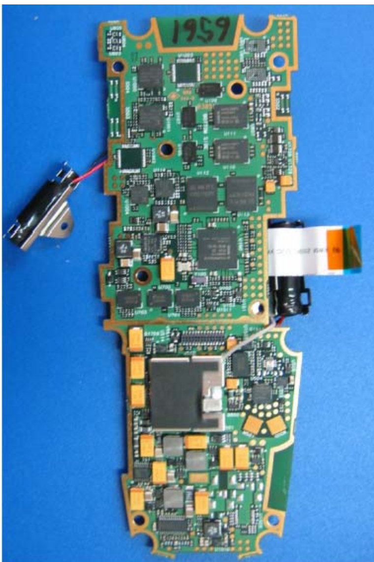
Photograph No.5 HC700-L main PCB bottom side view
