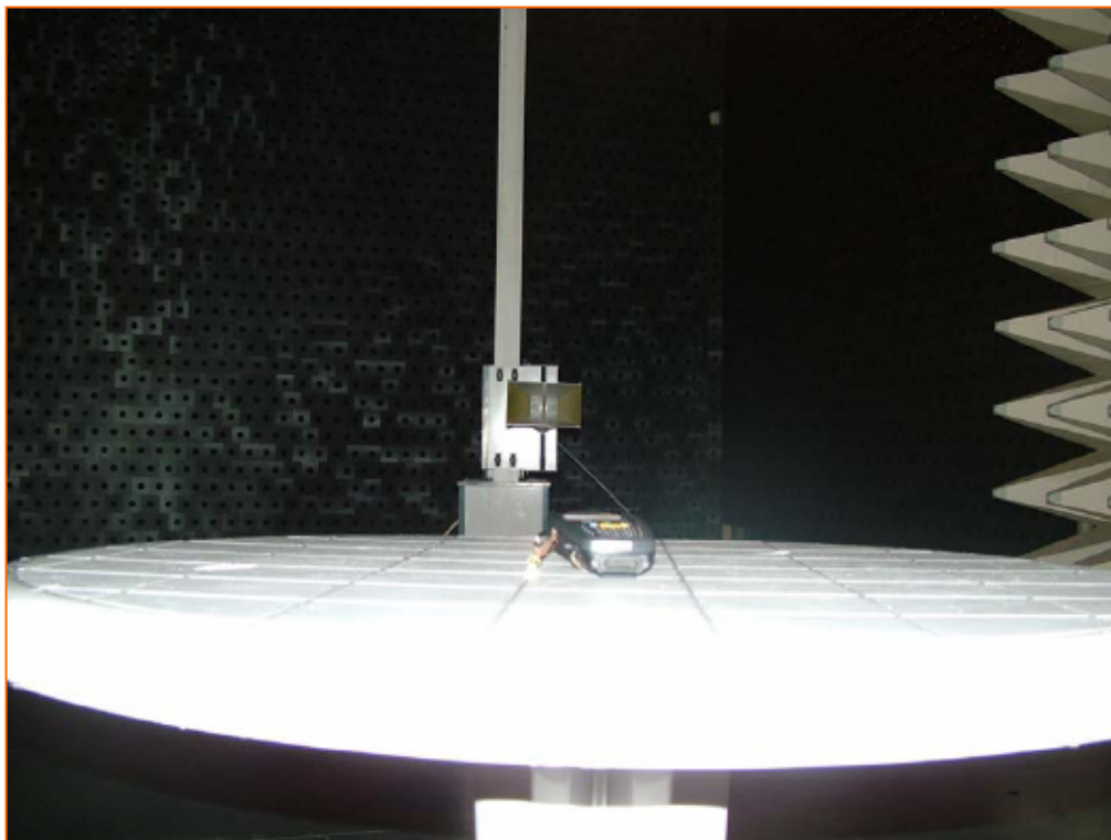
Photograph 4: Radiated measurements
