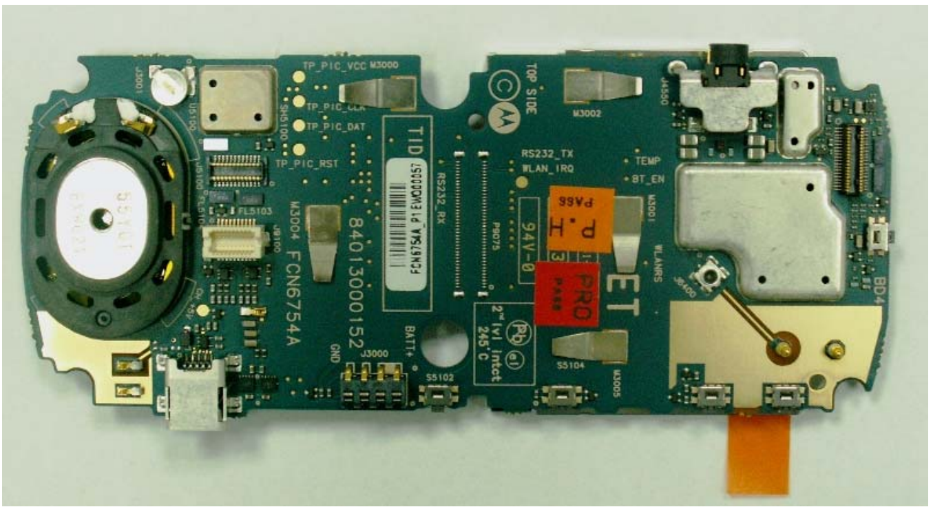
Photograph No. 2 - EWP3100 – Bottom Side with Shields
