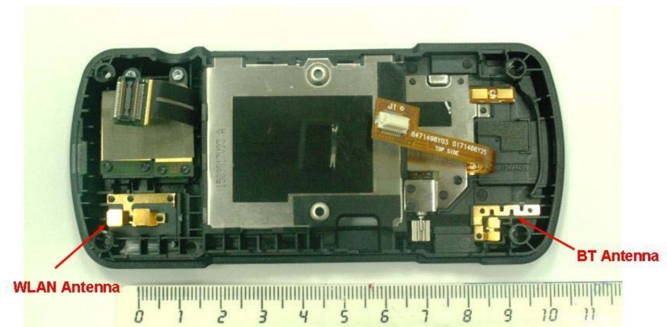
Photograph No. 7 - EWP3100 Antennas View
