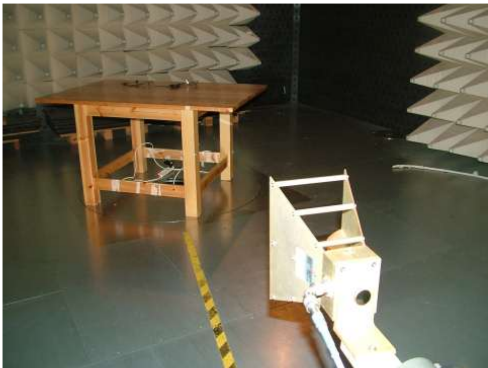
Photograph 2: Field strength of spurious radiation measurements
