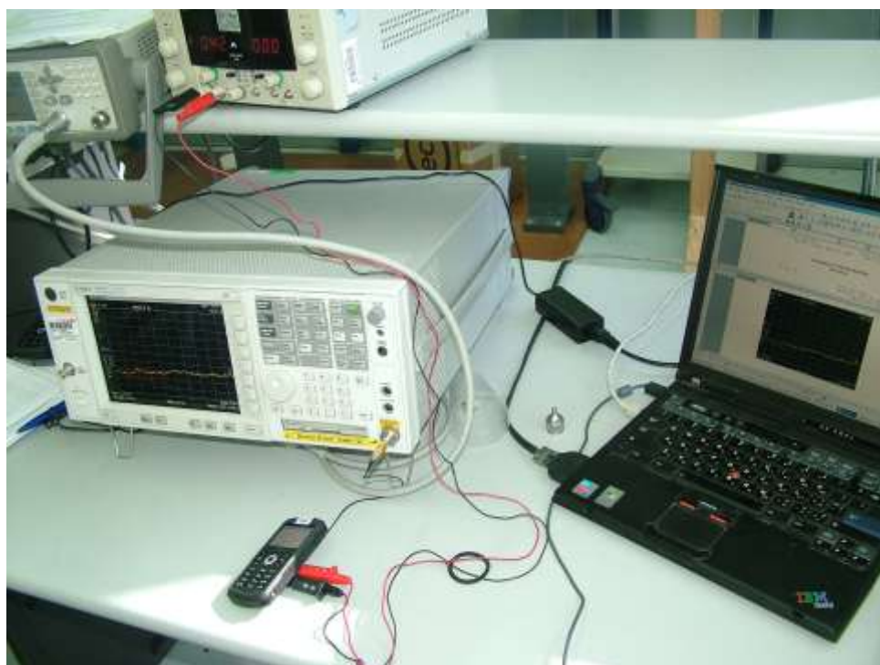
Photograph 4: Frequency stability test
