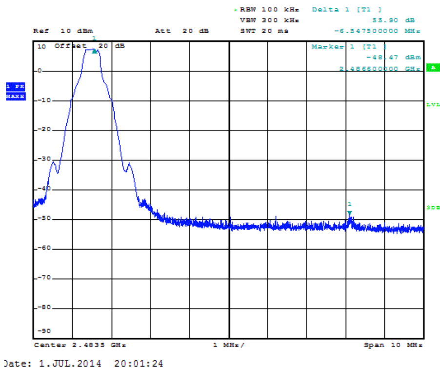
Figure 7.3.1.2-2: Upper Band-edge (GFSK)
