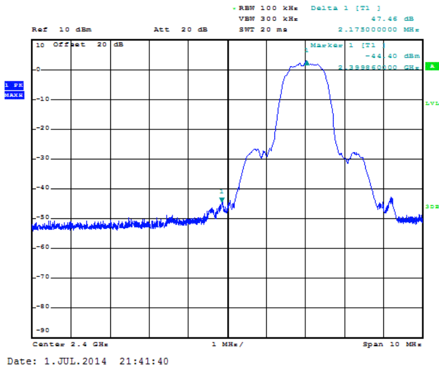
Figure 7.3.1.2-5: Lower Band-edge ( \pi/4 DQPSK)
