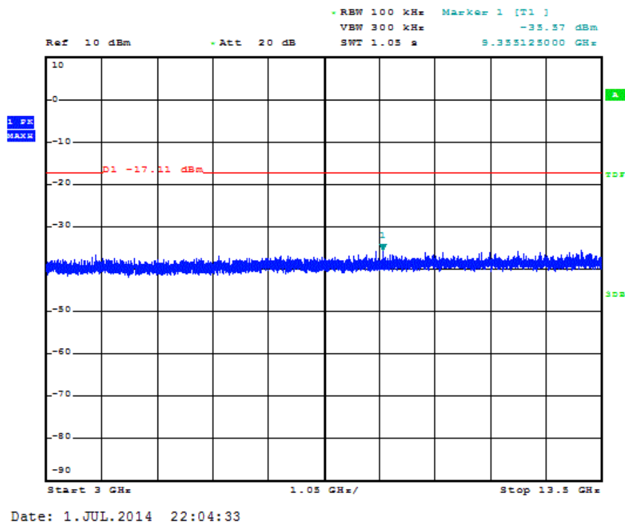
Figure 7.3.2.2-19: 3 GHz –13.5 GHz – Middle Channel ( \pi/4 DQPSK)
