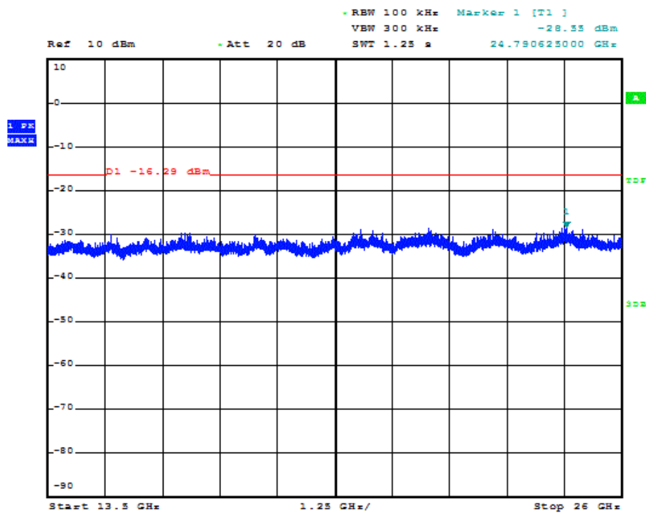
Figure 7.3.2.2-36: 13.5 GHz –26 GHz – High Channel (8DPSK)
