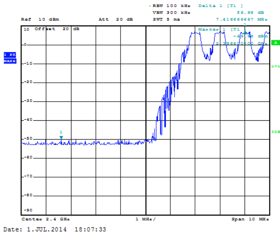
Figure 7.3.1.2-3: Lower Band-edge – Hopping Mode (GFSK)
