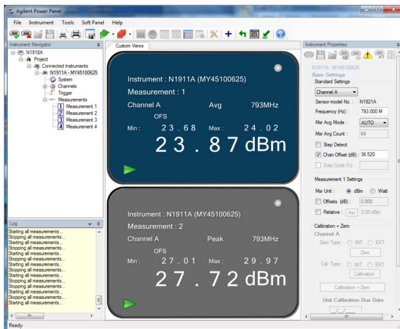
16-QAM 10MHz 1/49 RB Size/RB Offset
