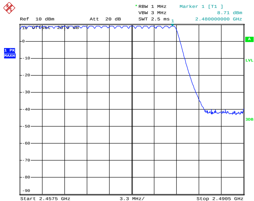
Figure 7.4.2.2-2: Number of Hopping Channels (24 – 56)
