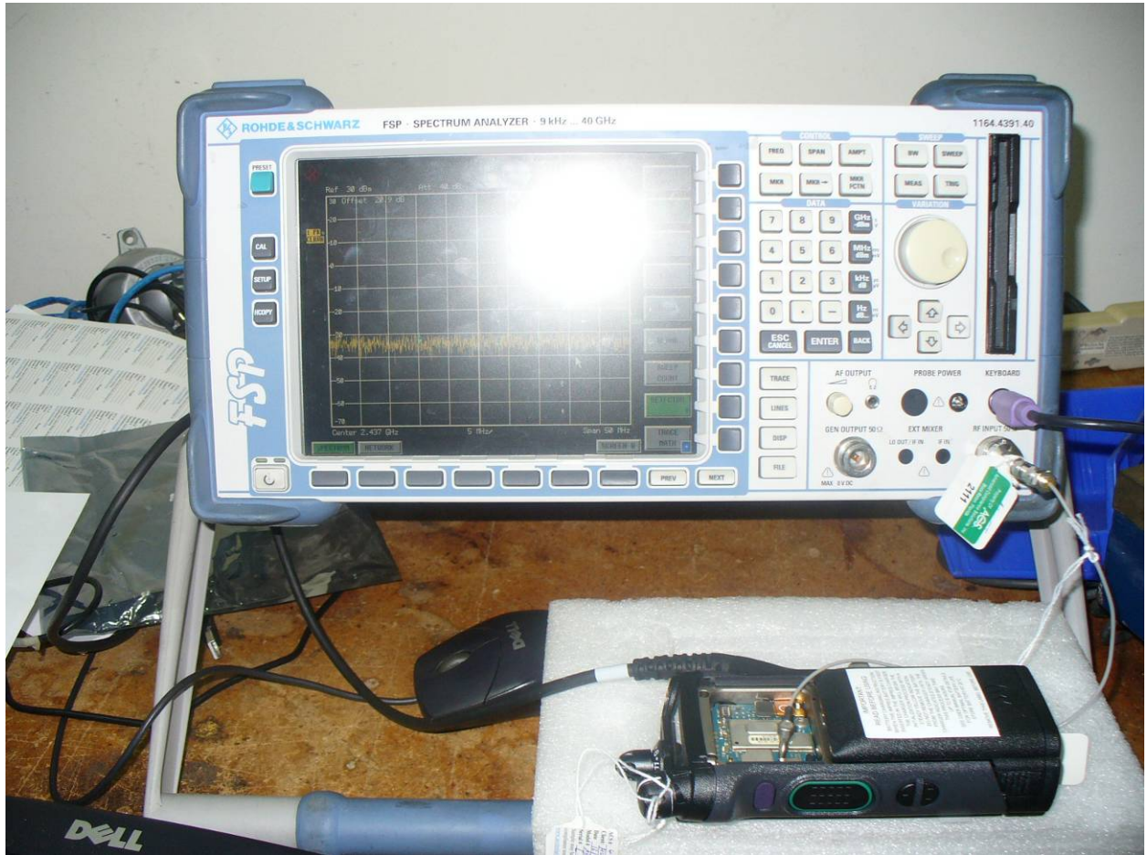
Figure 5: RF Conducted Emissions
