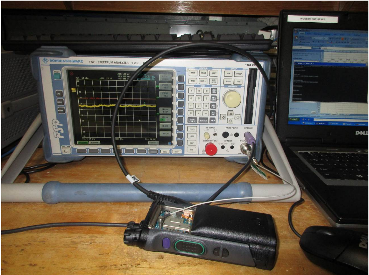
Figure 15: RF Conducted Emissions
