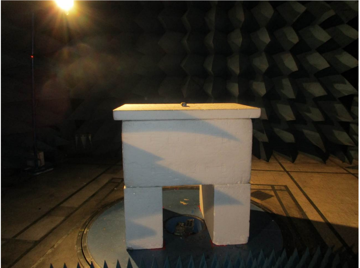
Figure 11: Radiated Emissions – Front View – EUT Flat (Above 1 GHz)
