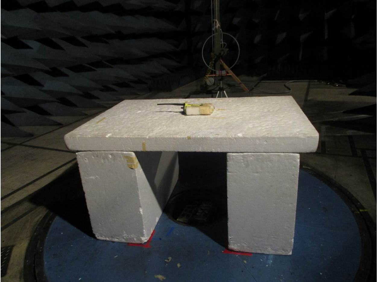
Figure 2: Radiated Emissions – Back View – EUT on Side (9 kHz – 30 MHz)
