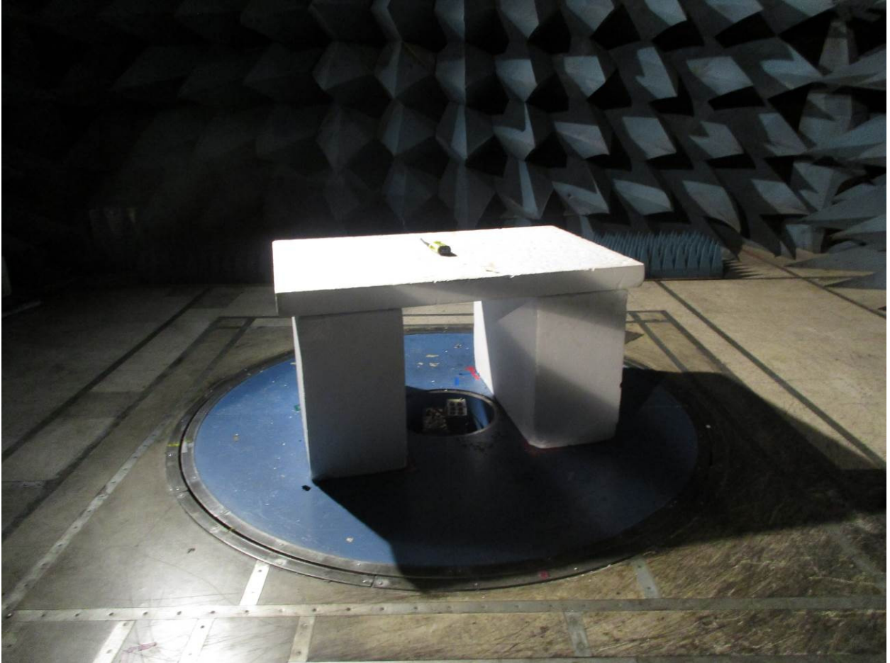
Figure 7: Radiated Emissions – Front View – EUT Flat (Below 1 GHz)
