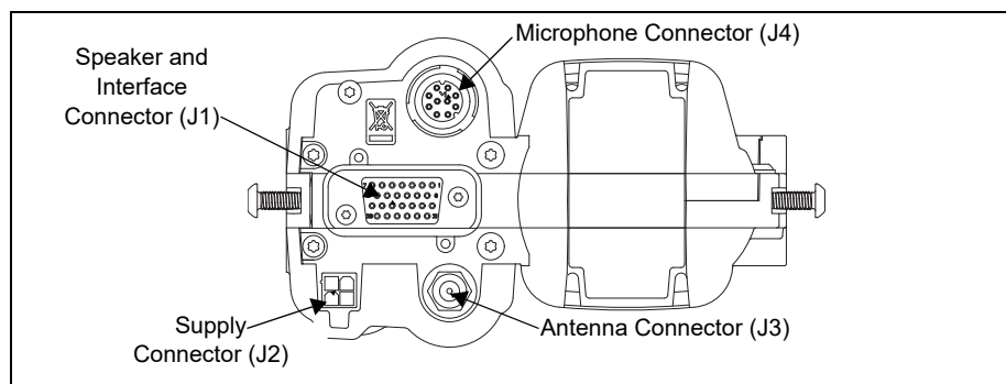
Figure 7: Console Connections
