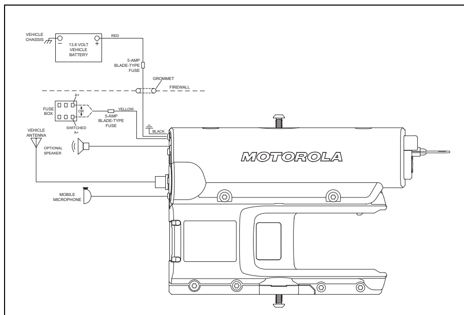
Figure 8: Console Cabling
