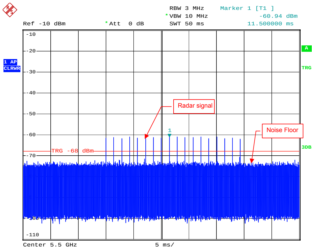
Radar Signal 0
