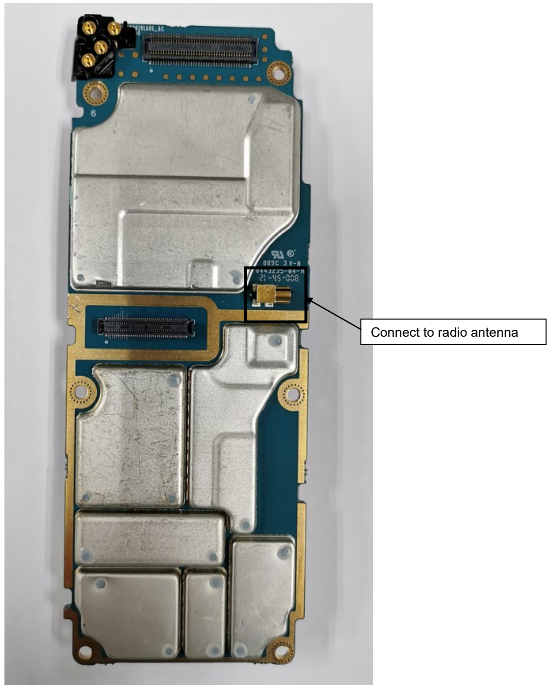
RF board with Shields (Top)
