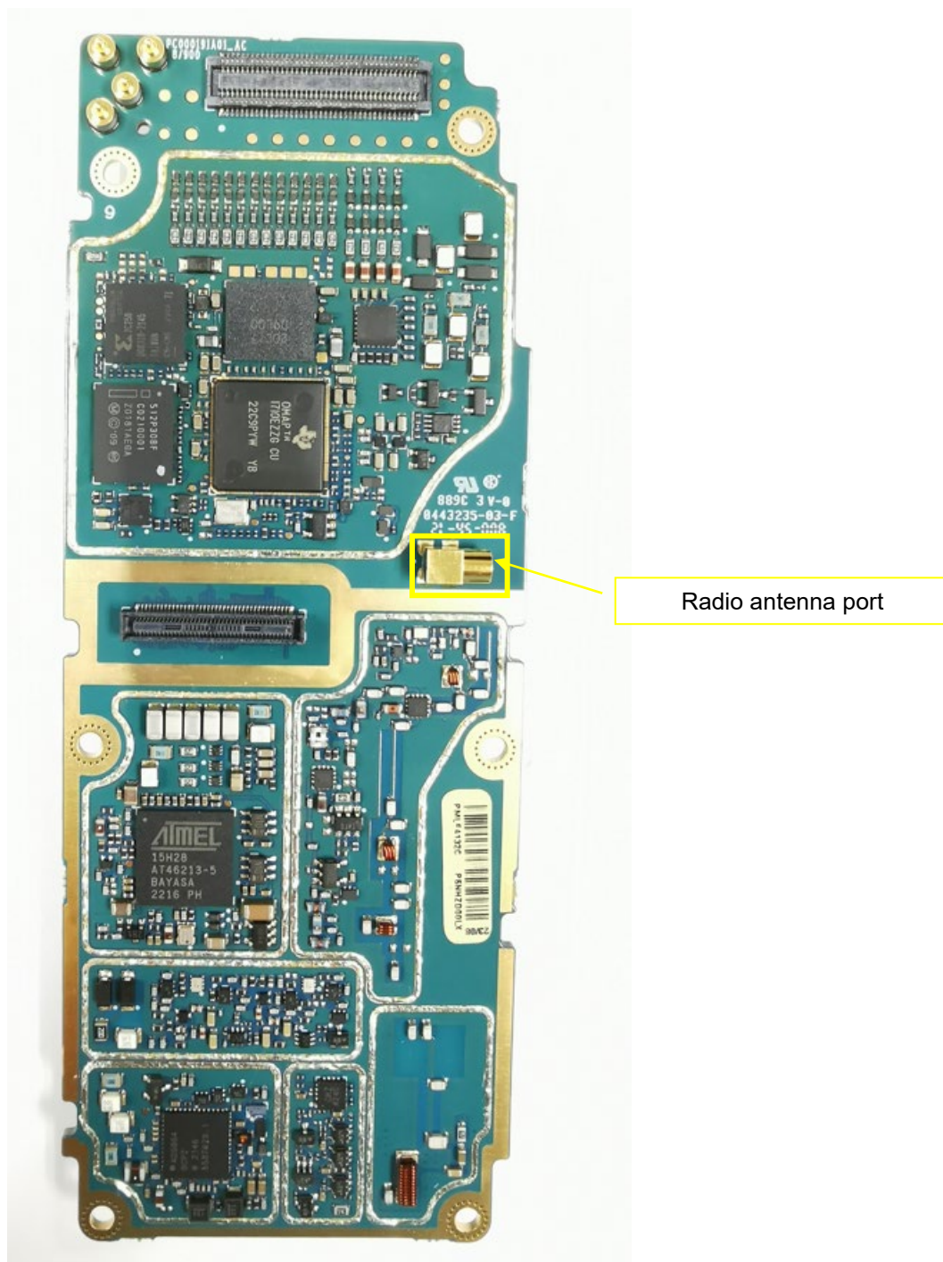
RF board without Shields (Top)
