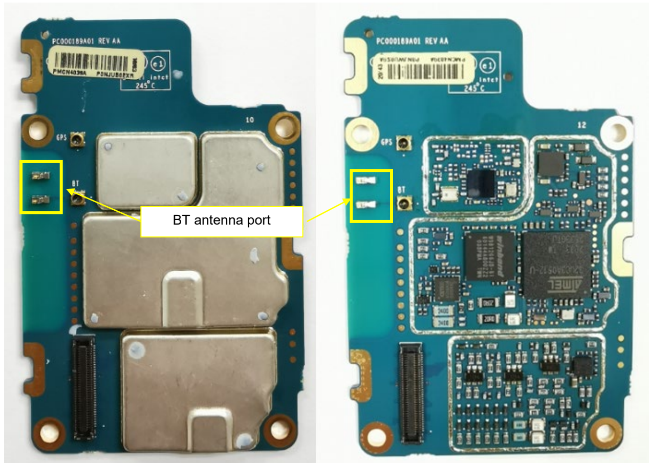
Expansion board with and without shields (Top)
