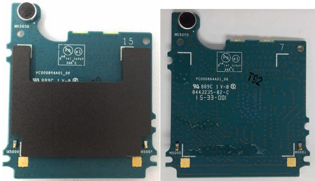
Interface board (Top) with and without Poron Pad
